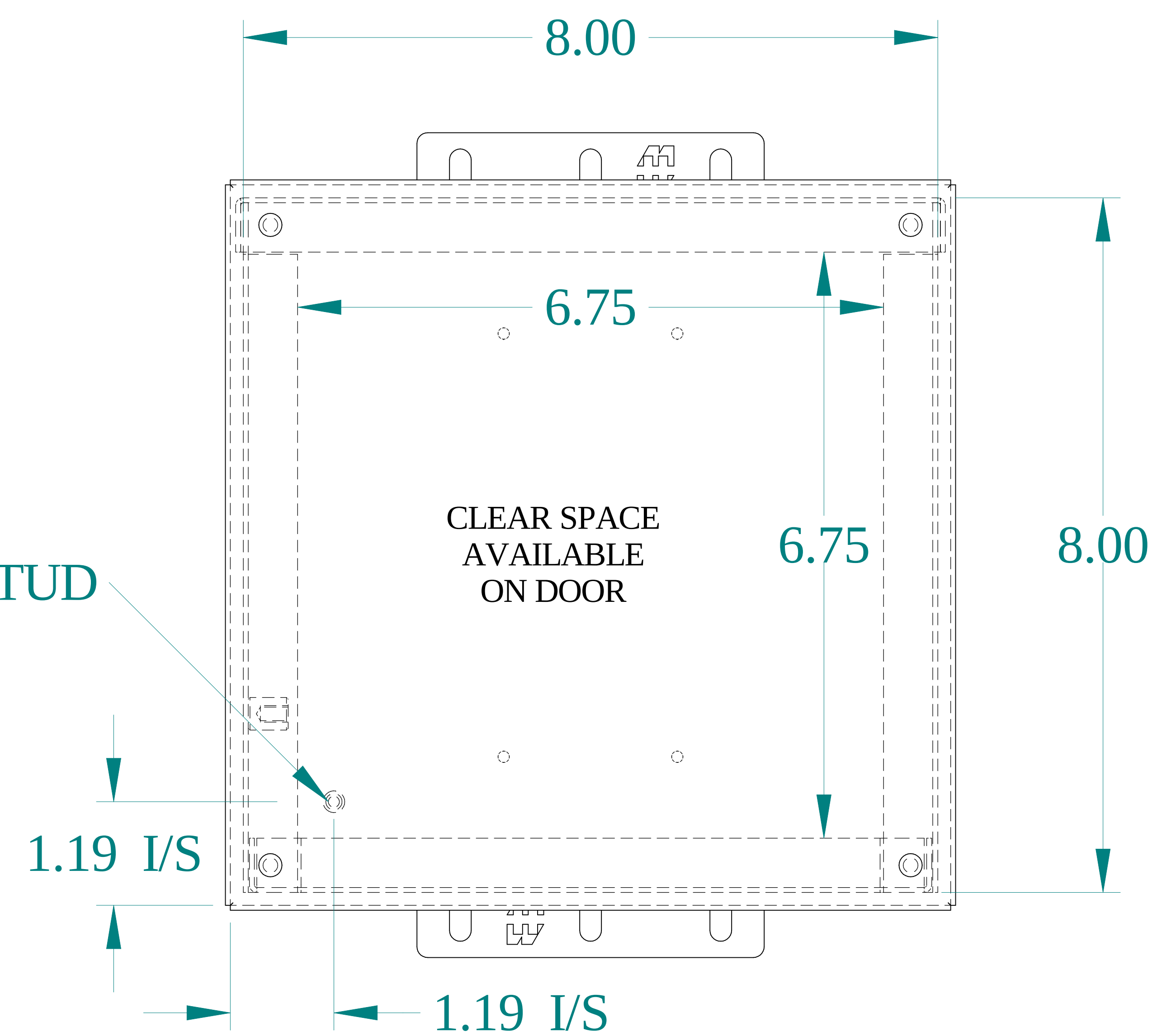
FRONT VIEW
