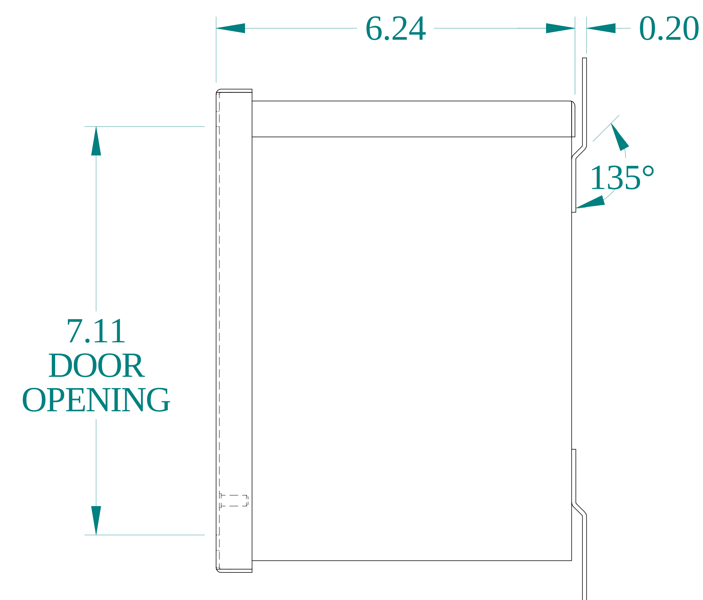
SIDE VIEW
