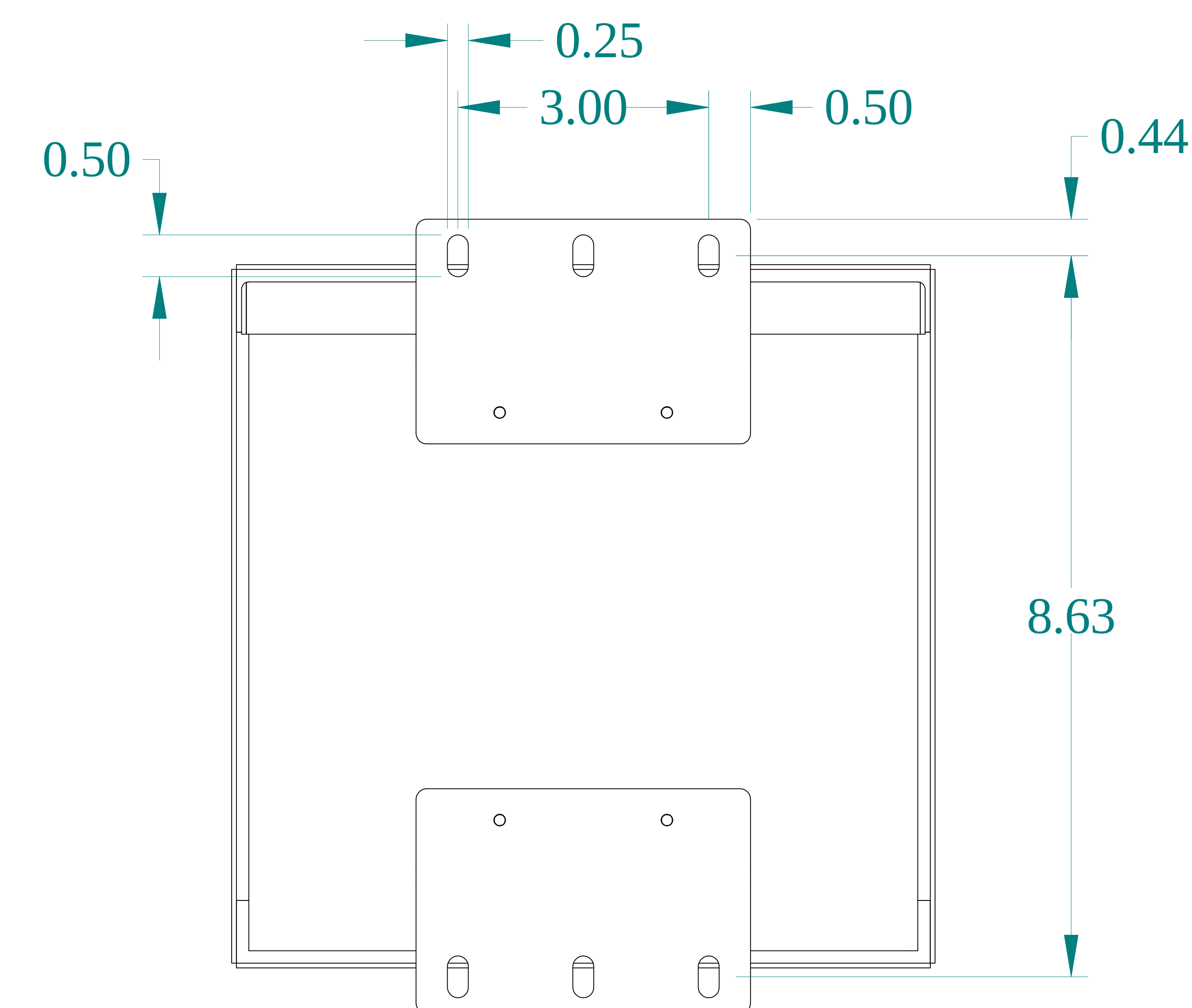
BACK VIEW
