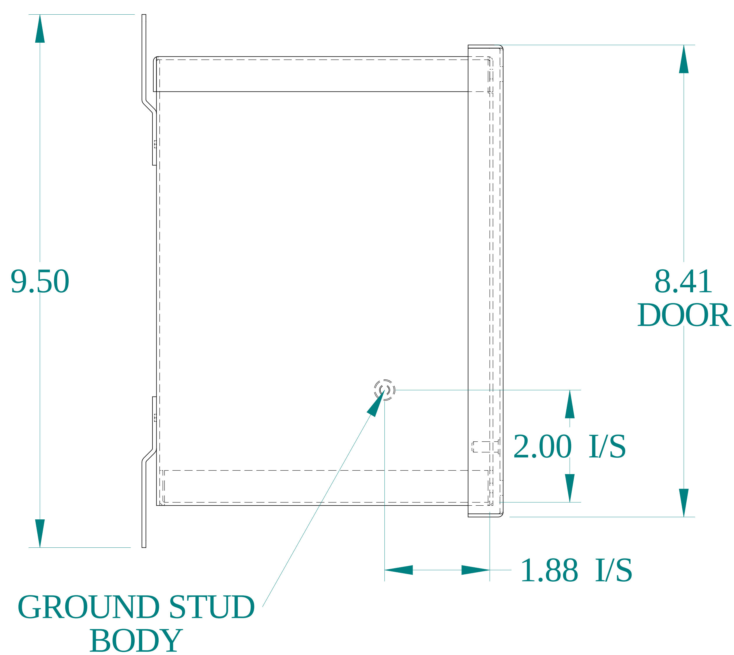
SIDE VIEW
