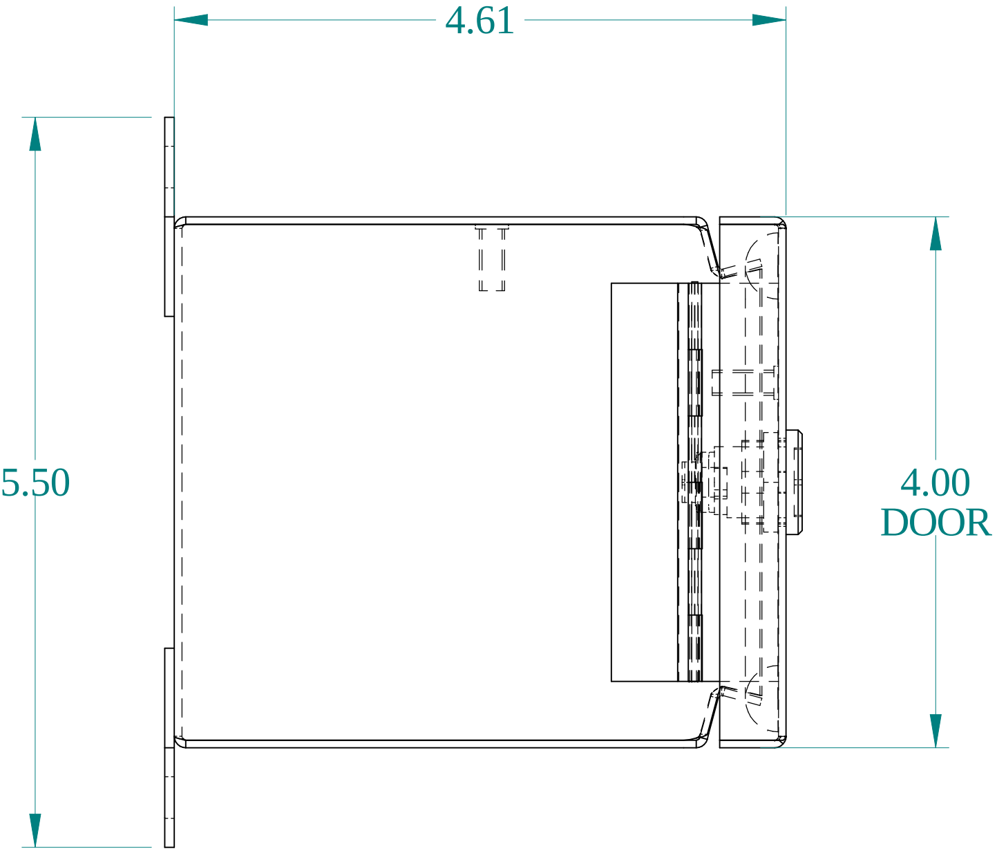
SIDE VIEW
