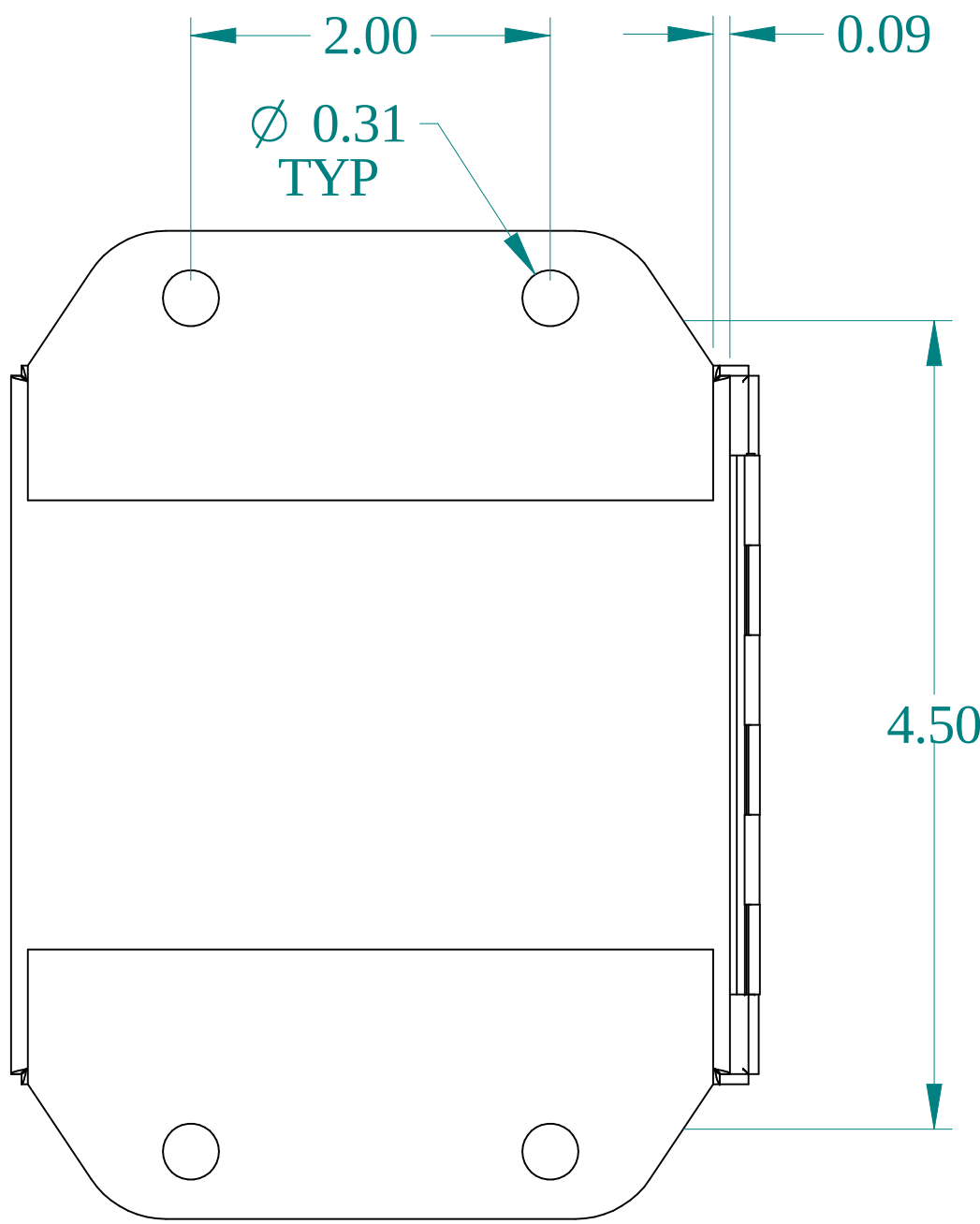
BACK VIEW
