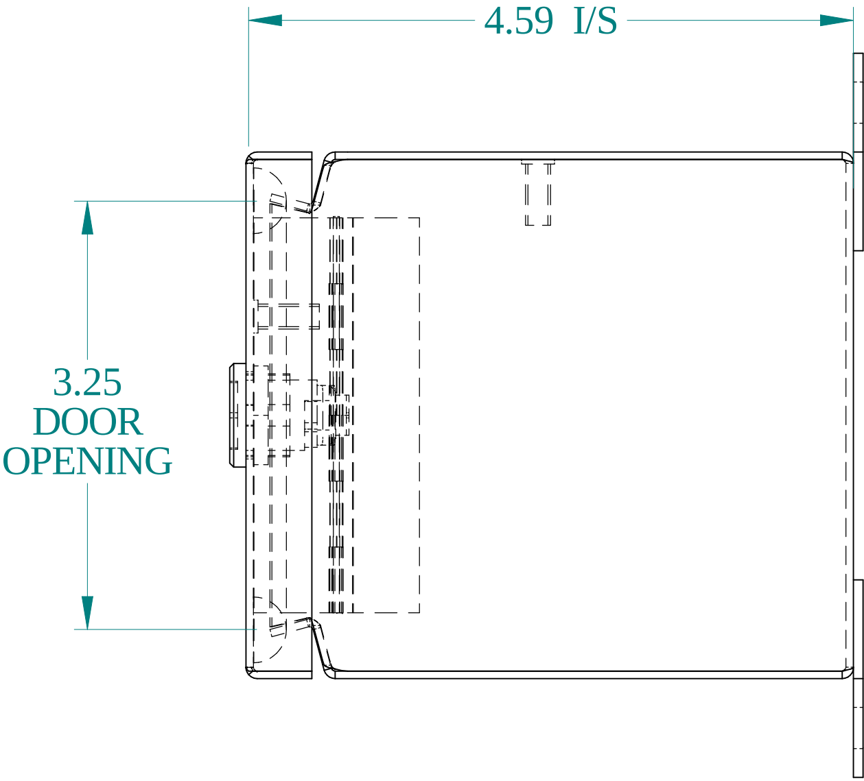
SIDE VIEW
