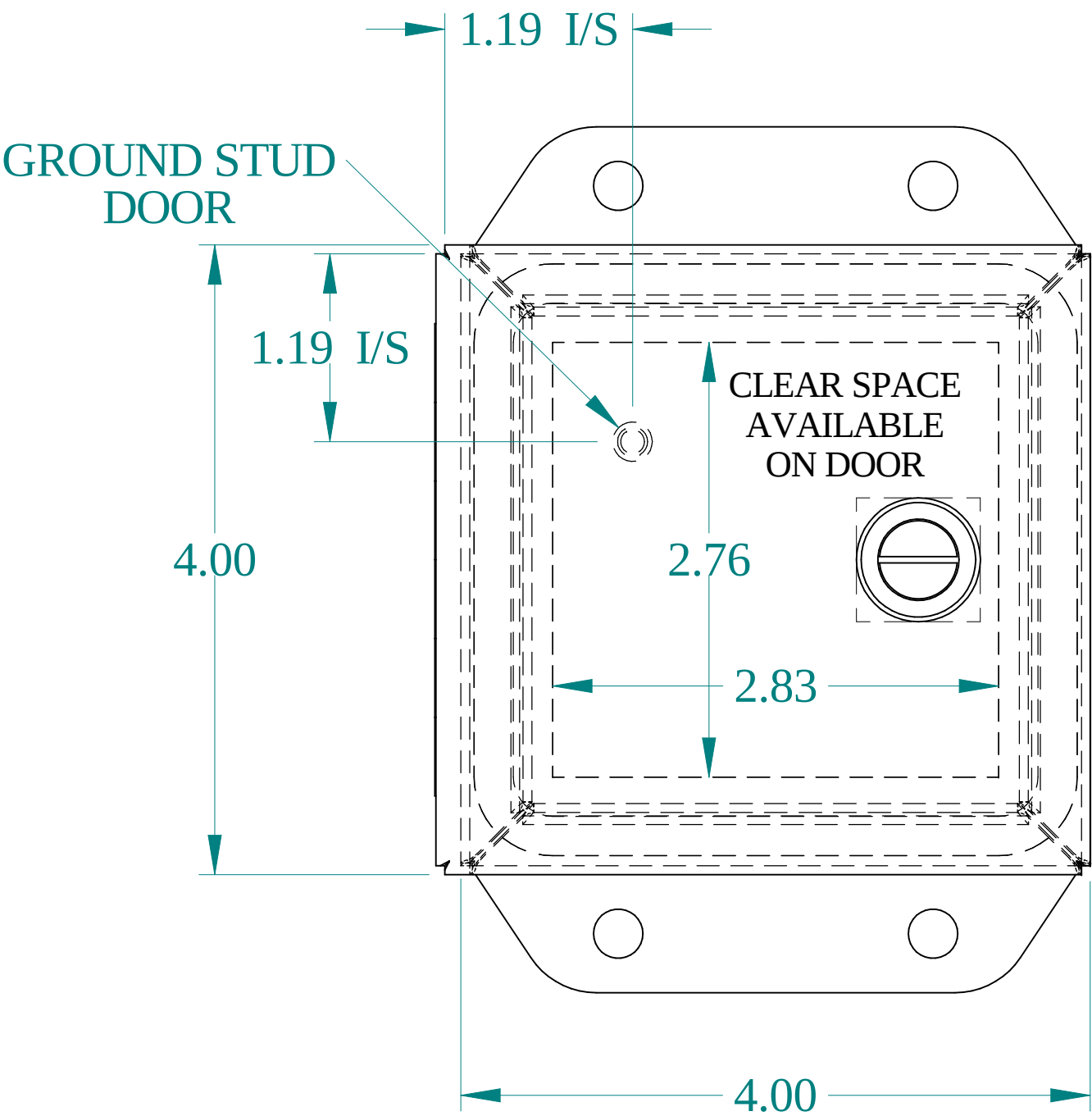
FRONT VIEW
