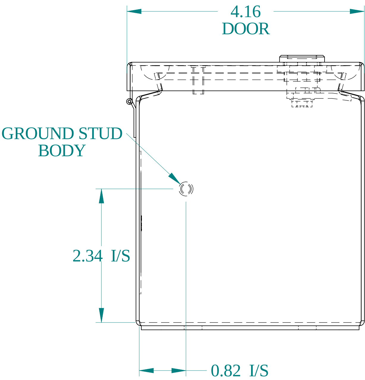
BOTTOM VIEW
