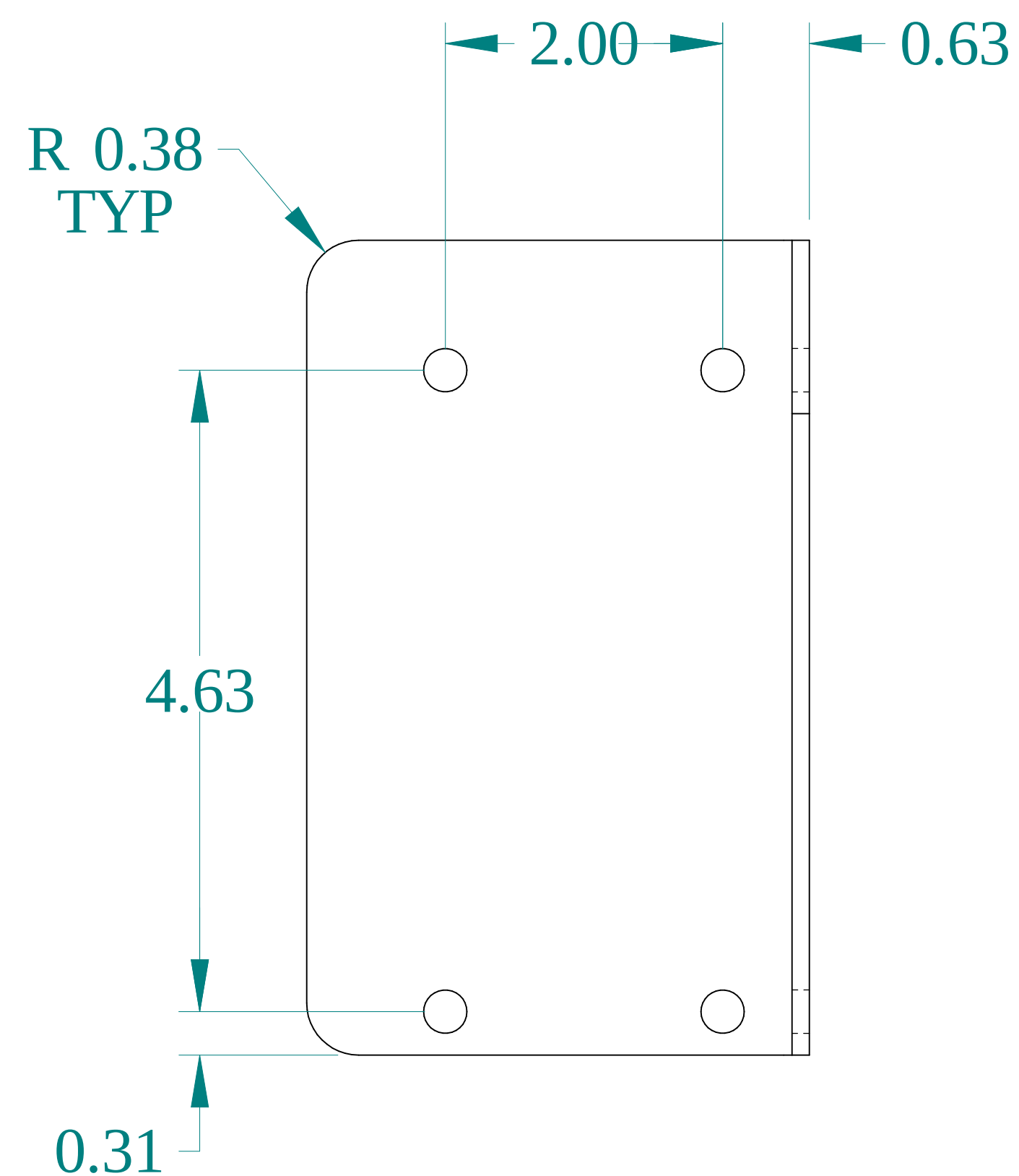
SIDE VIEW
