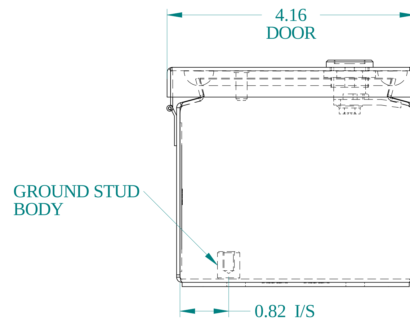
BOTTOM VIEW
