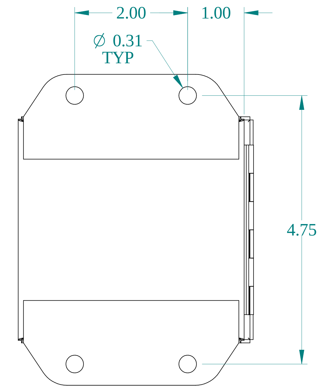
BACK VIEW
