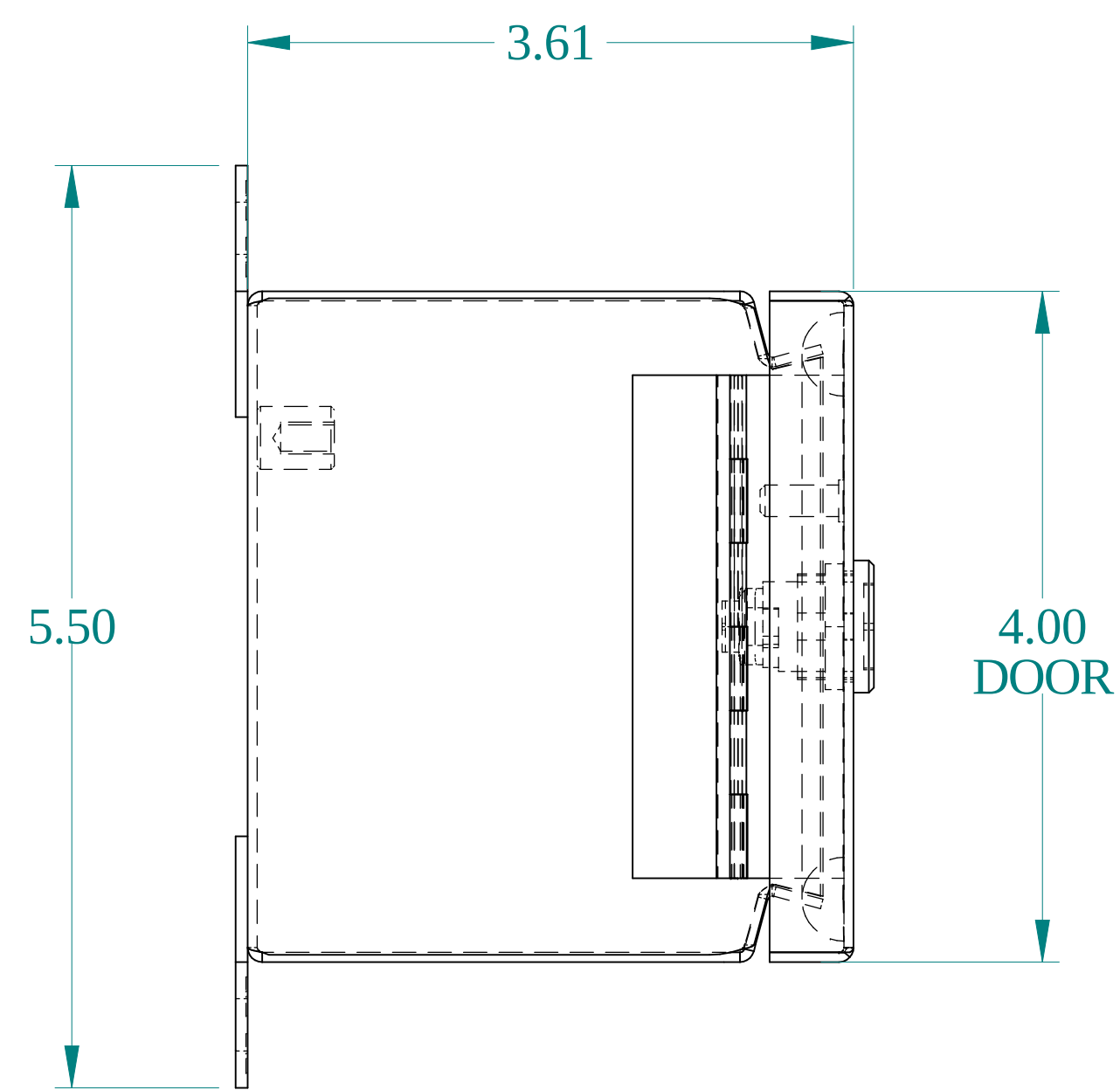
SIDE VIEW
