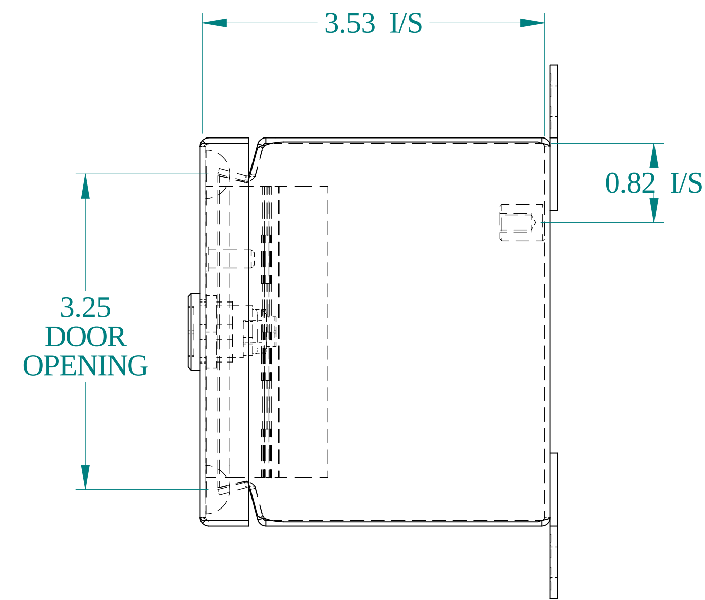
SIDE VIEW
