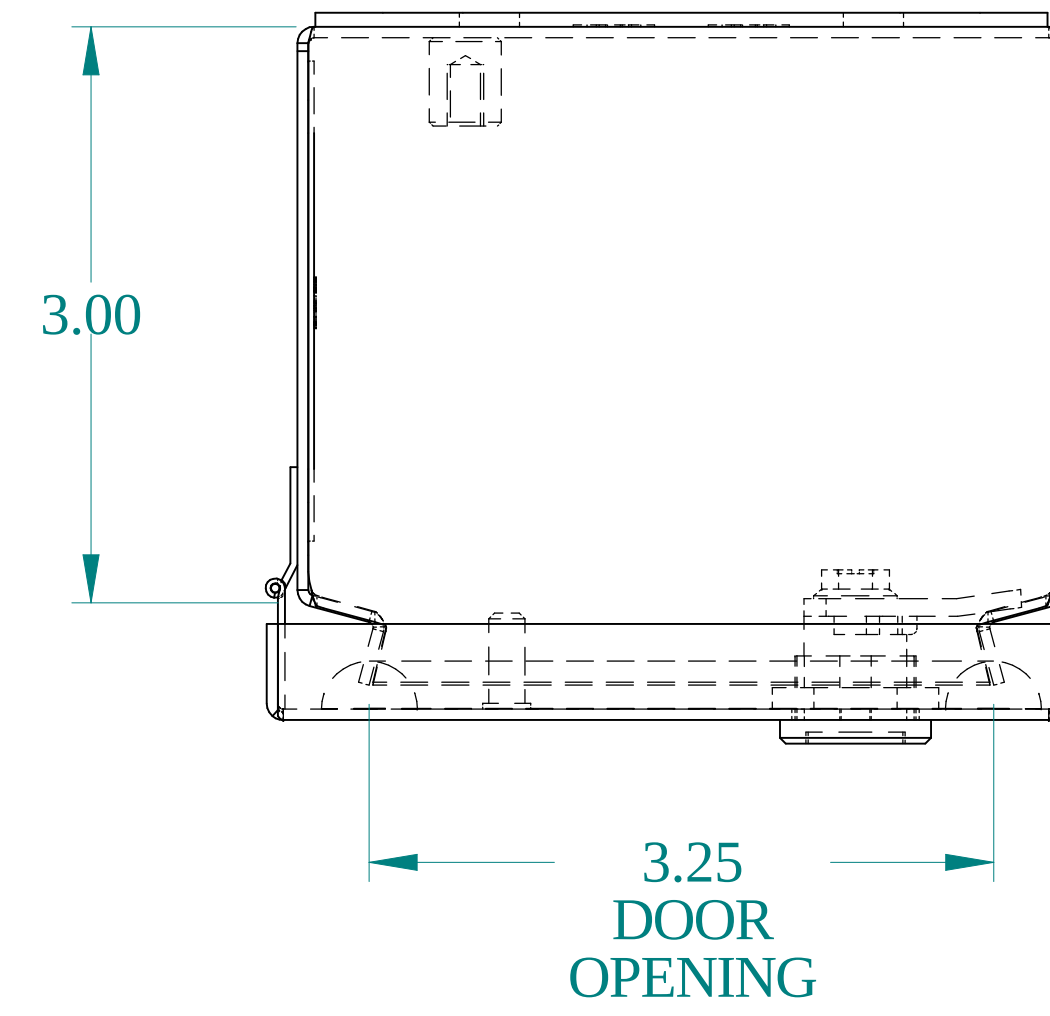
TOP VIEW
