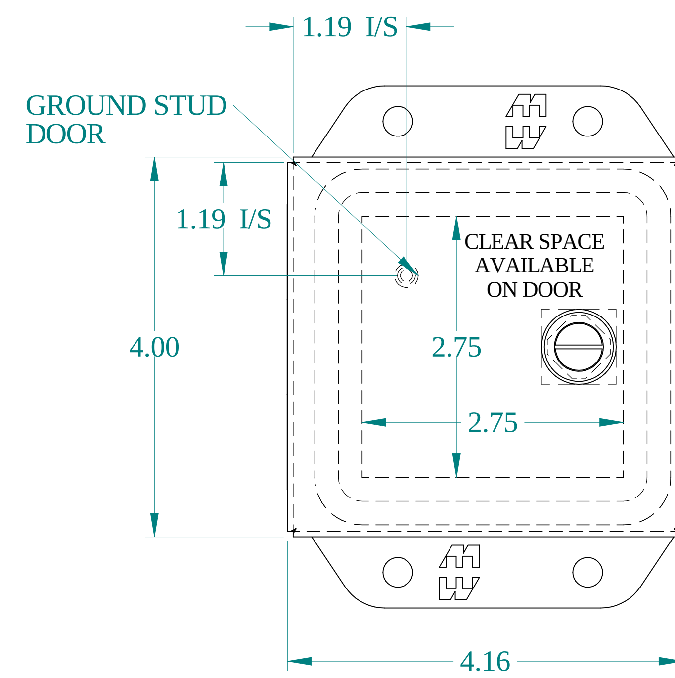
FRONT VIEW
