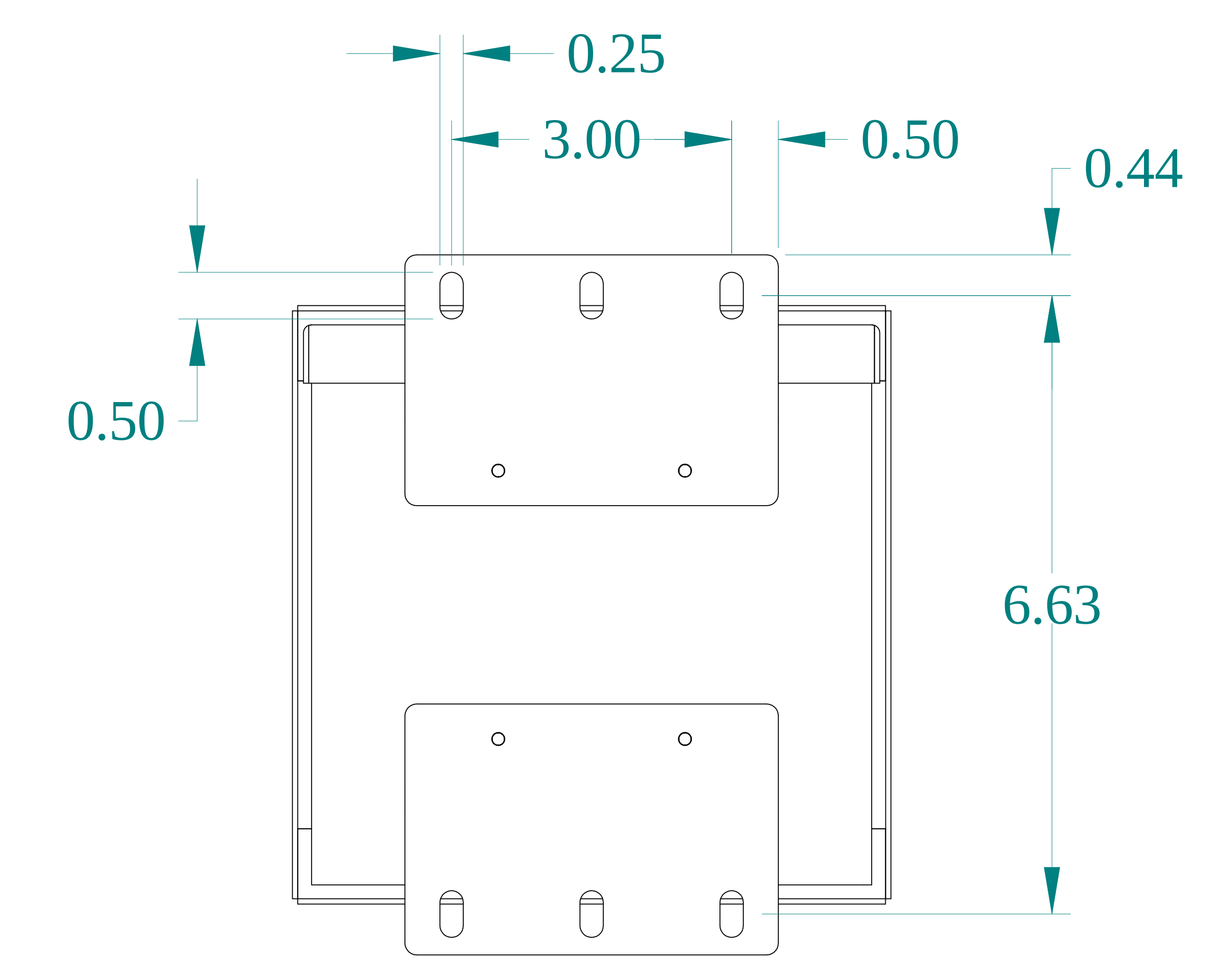
BACK VIEW
