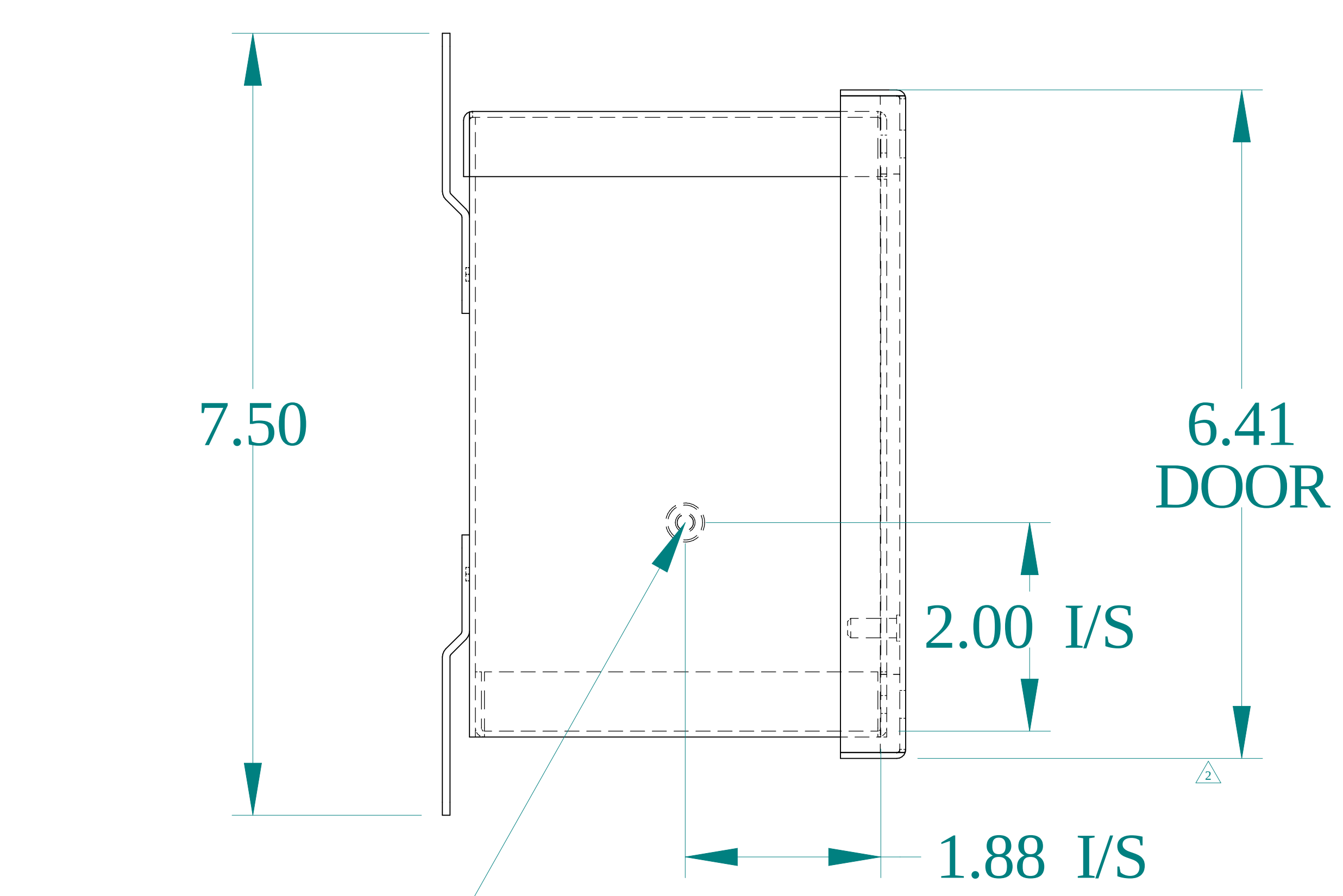
SIDE VIEW
