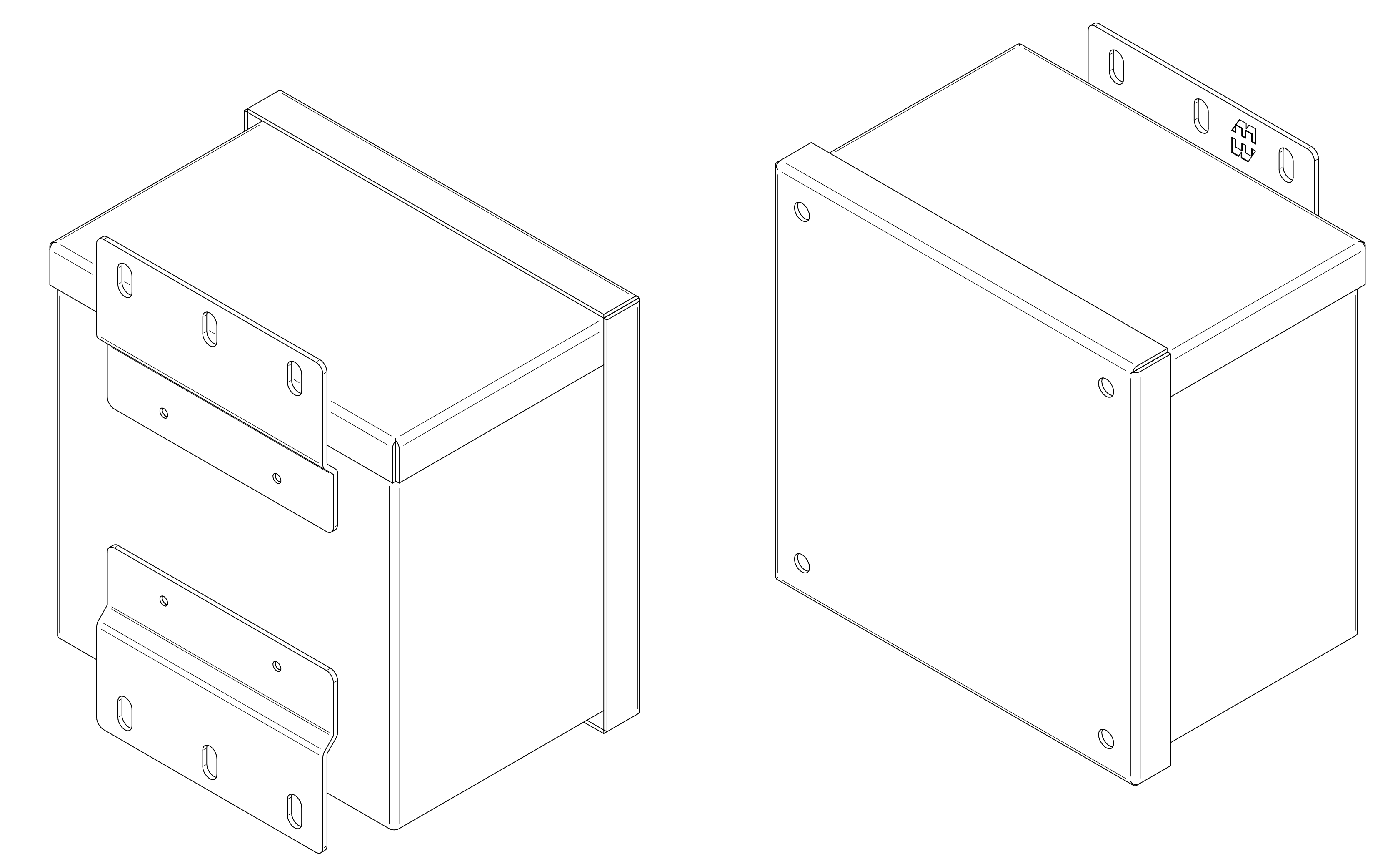
ISOMETRIC VIEWS
