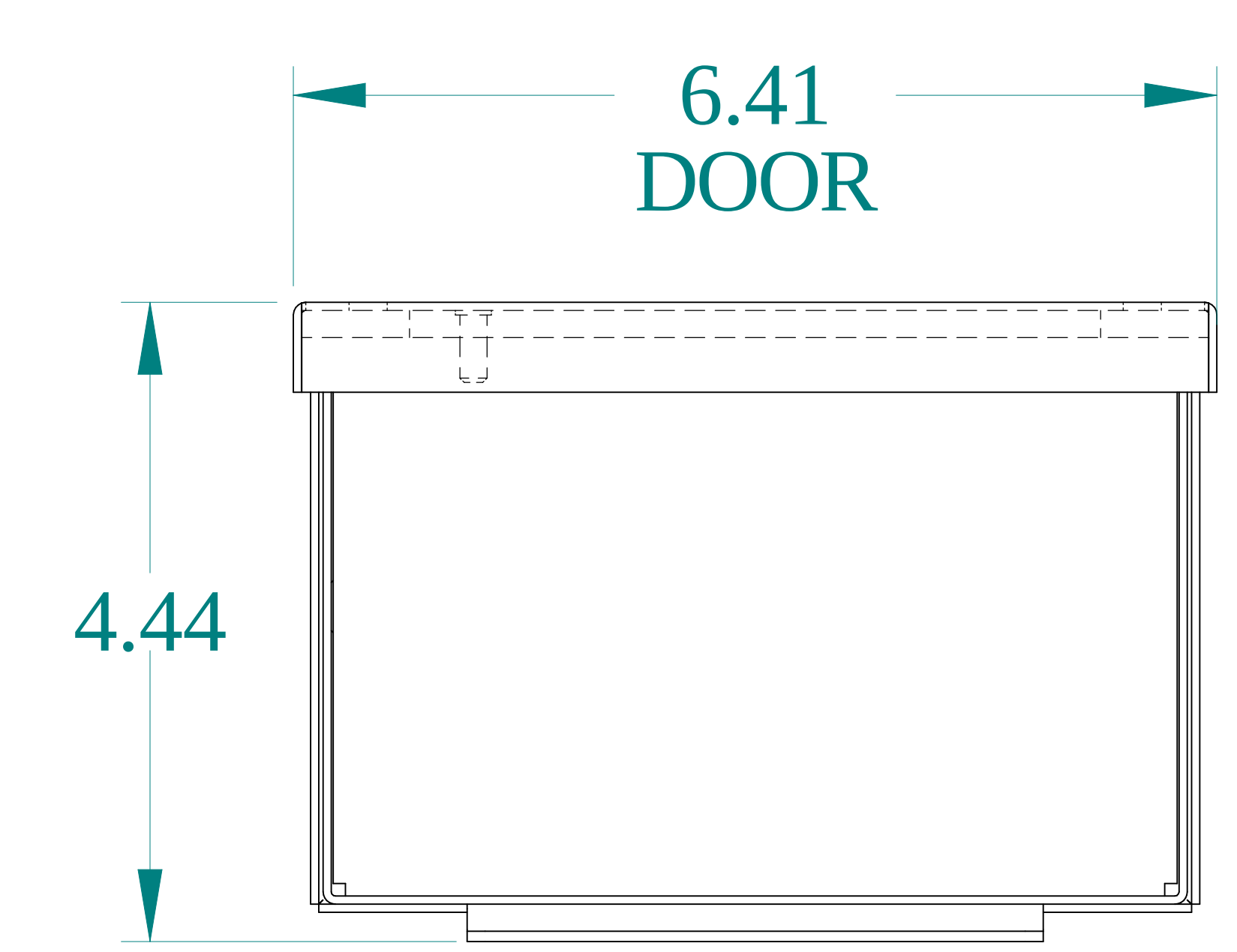
BOTTOM VIEW
