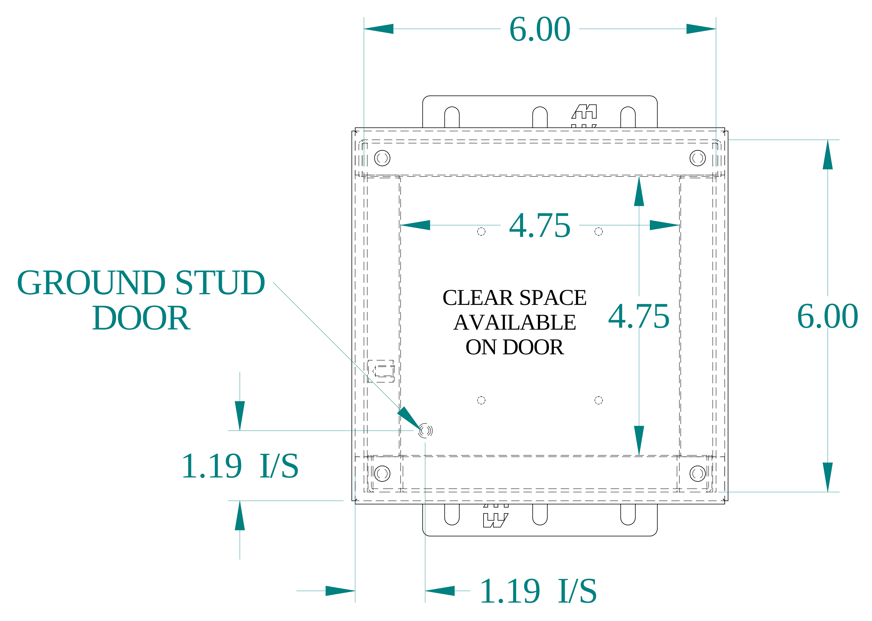
FRONT VIEW
