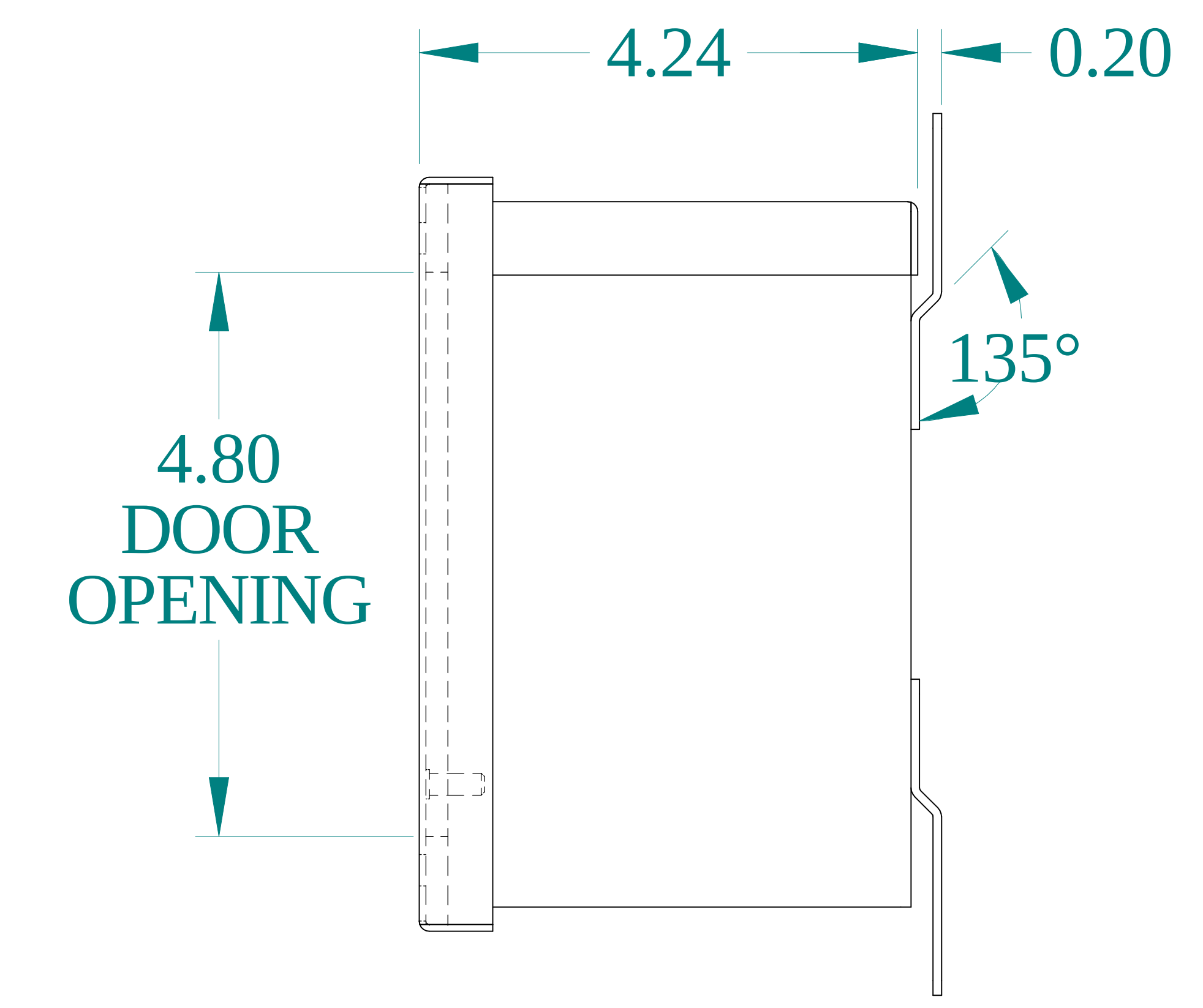
SIDE VIEW
