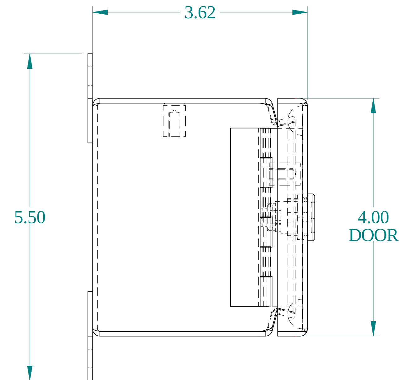
SIDE VIEW
