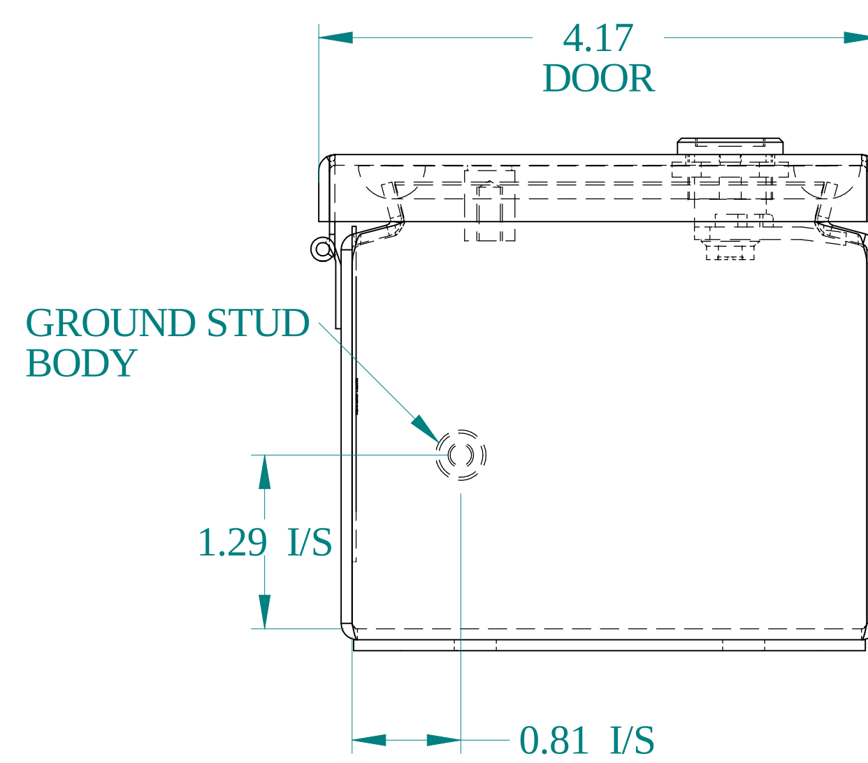
BOTTOM VIEW
