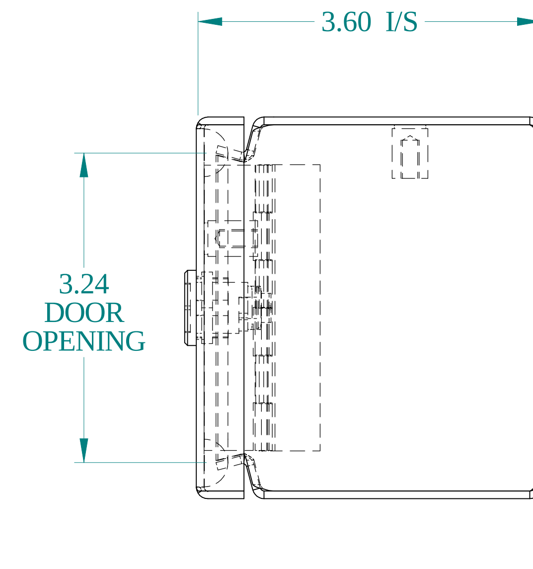
SIDE VIEW
