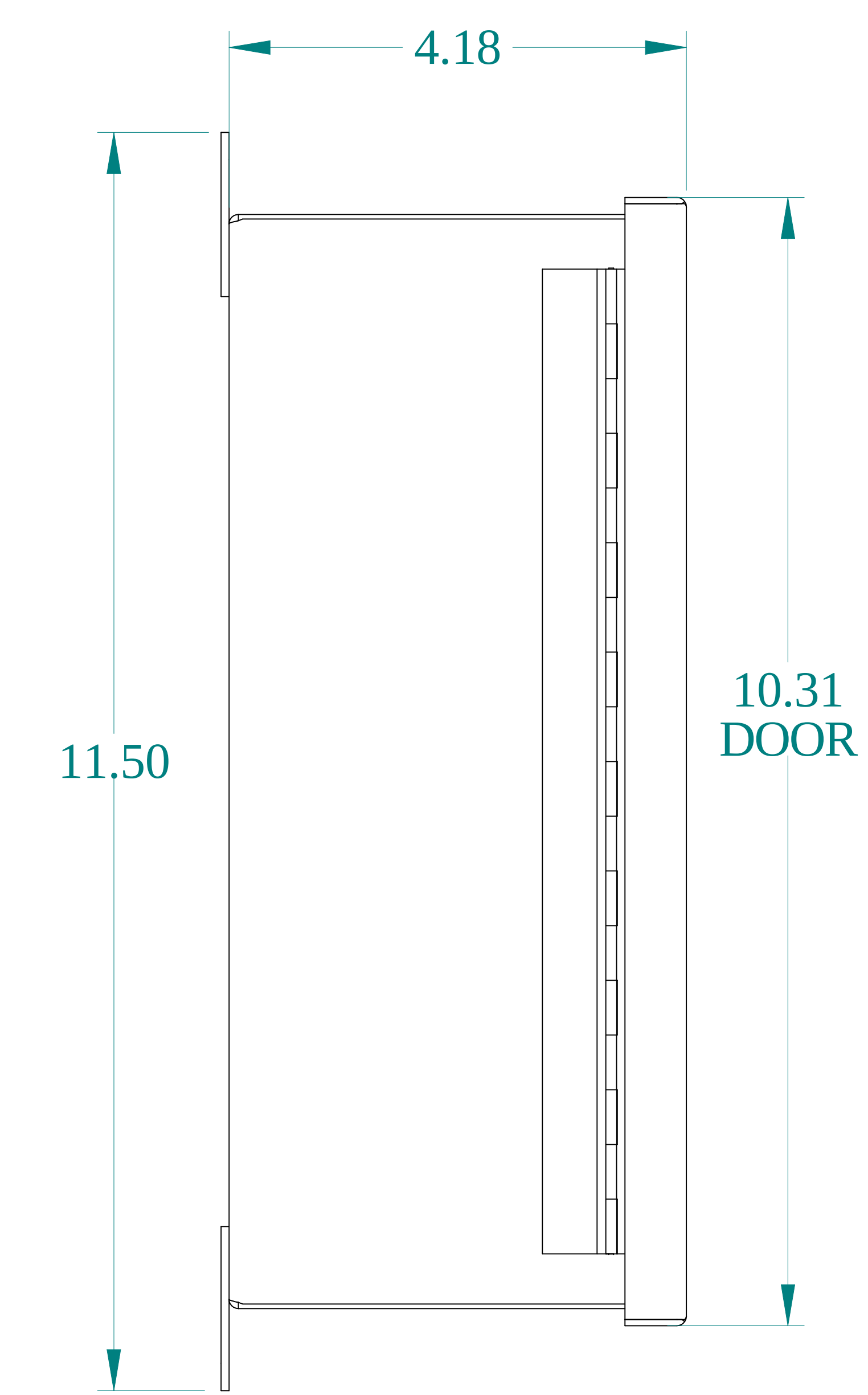
SIDE VIEW
