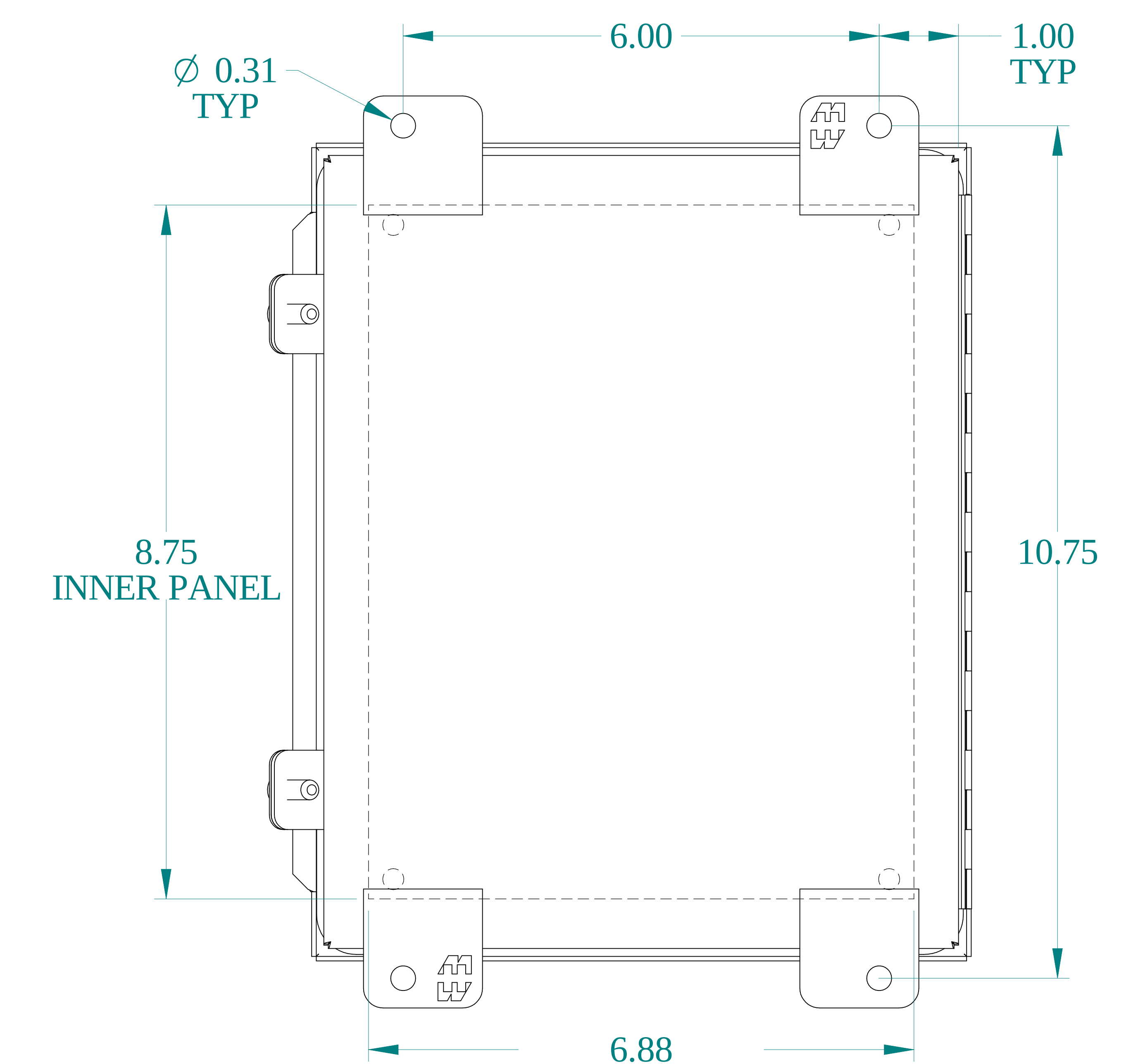
BACK VIEW
