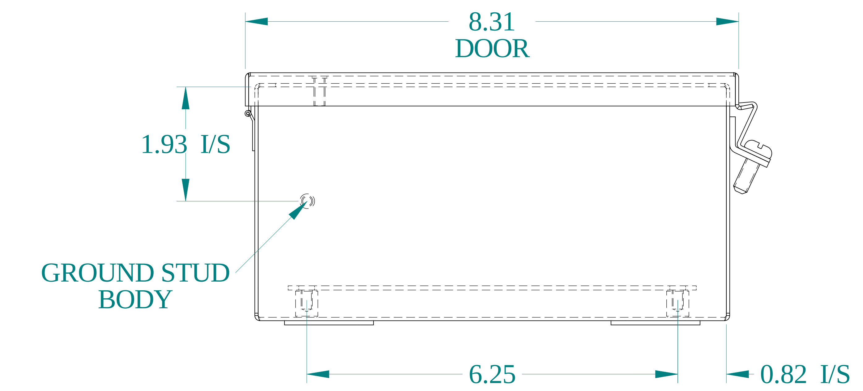
BOTTOM VIEW
