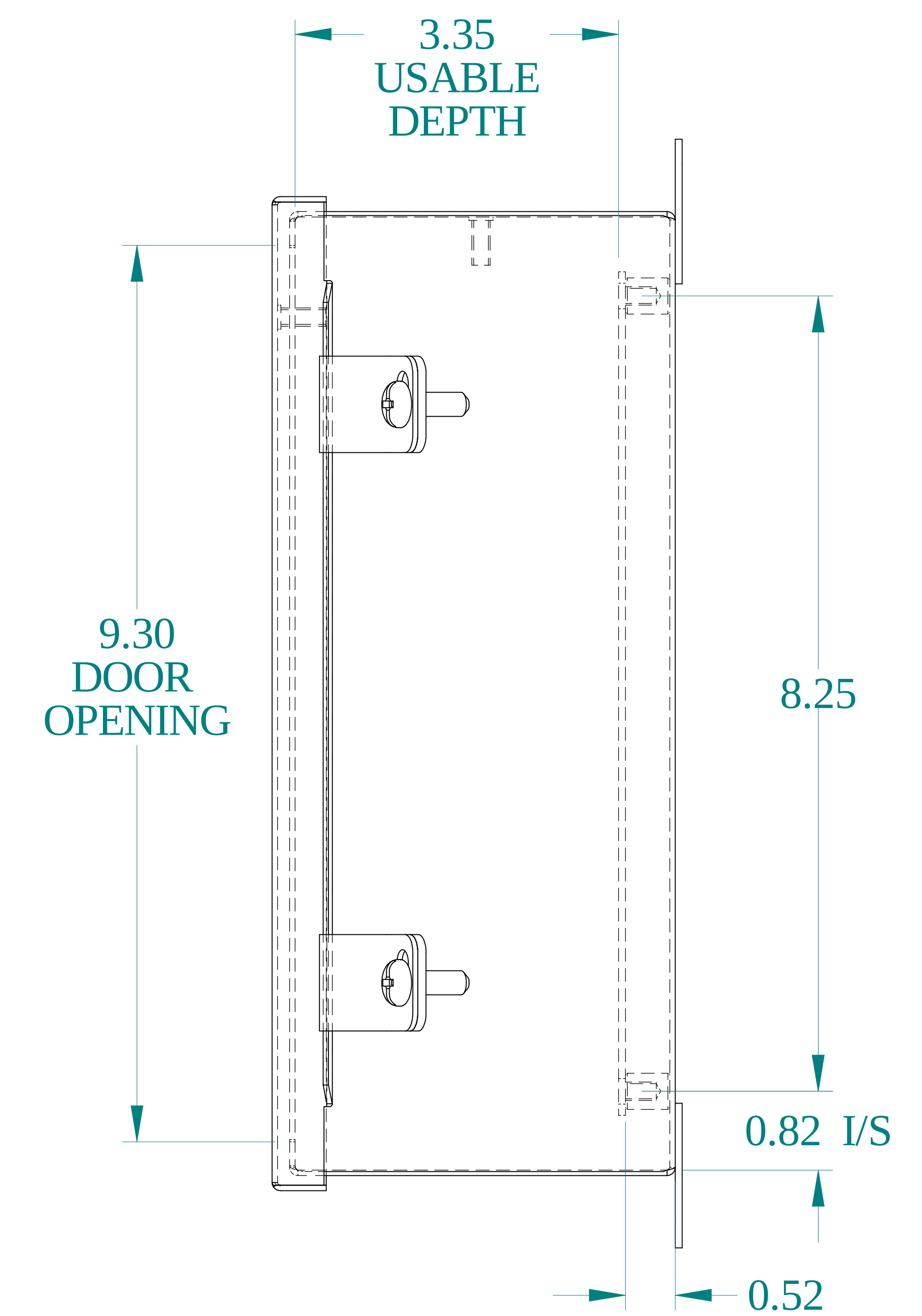
SIDE VIEW
