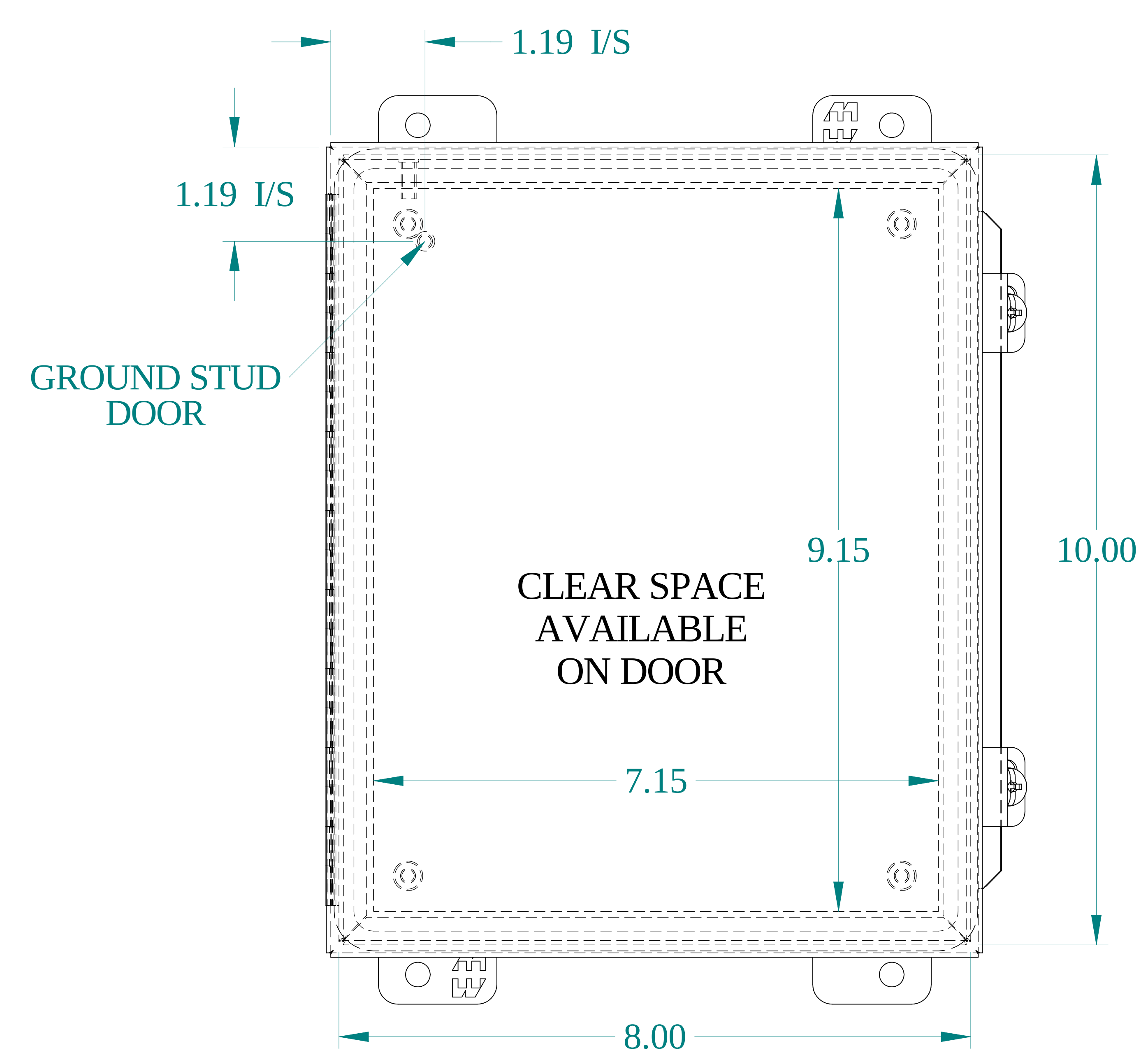
FRONT VIEW
