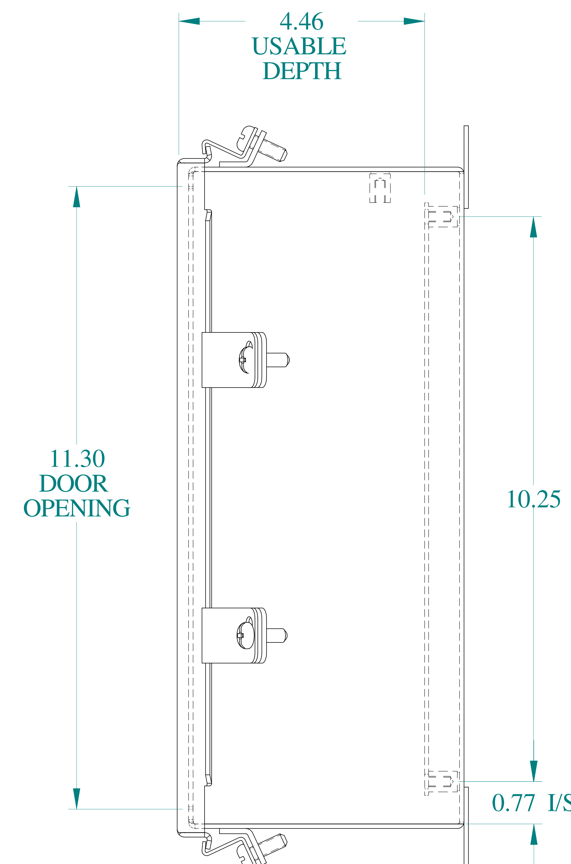
SIDE VIEW
