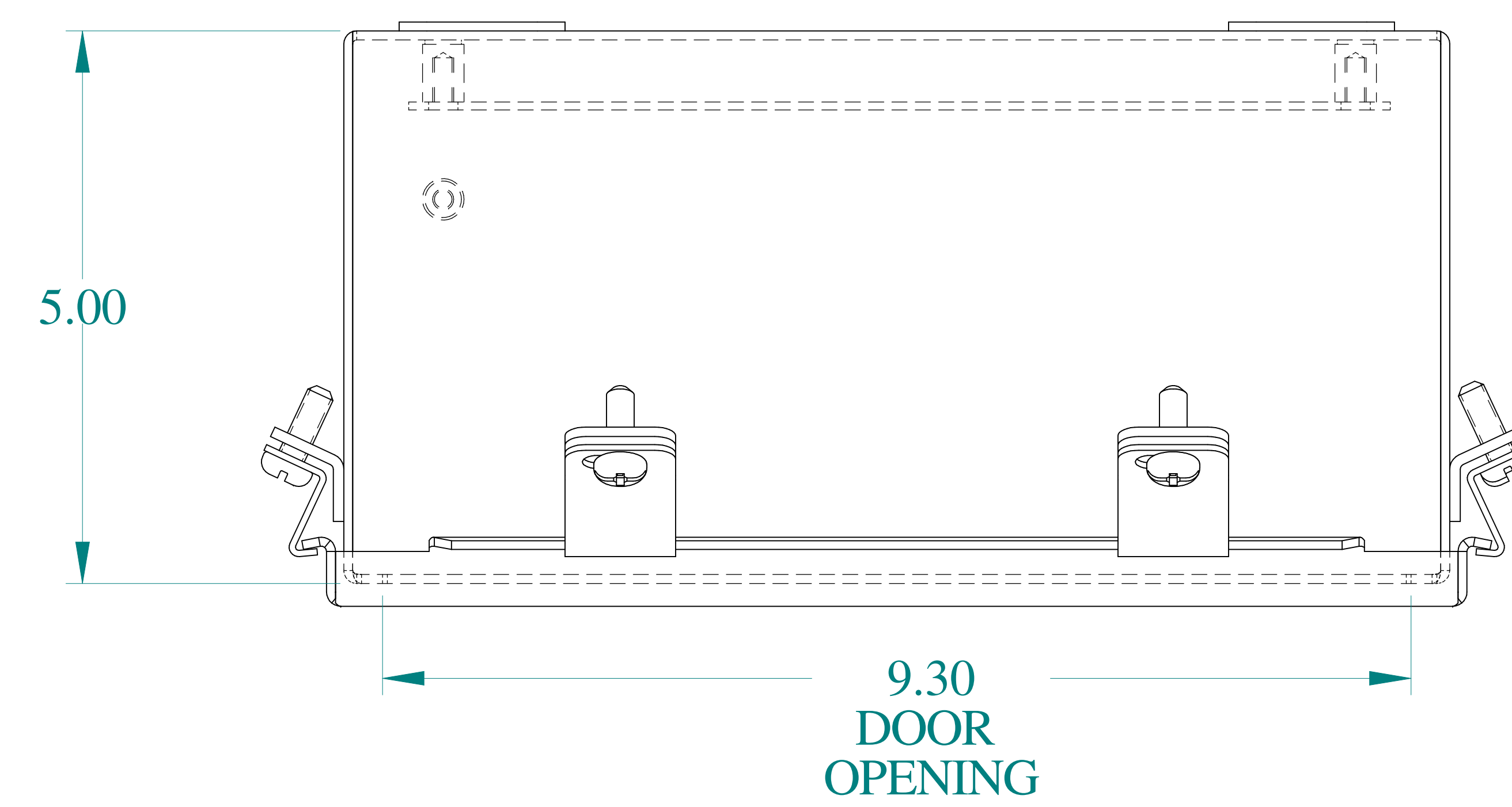
TOP VIEW
