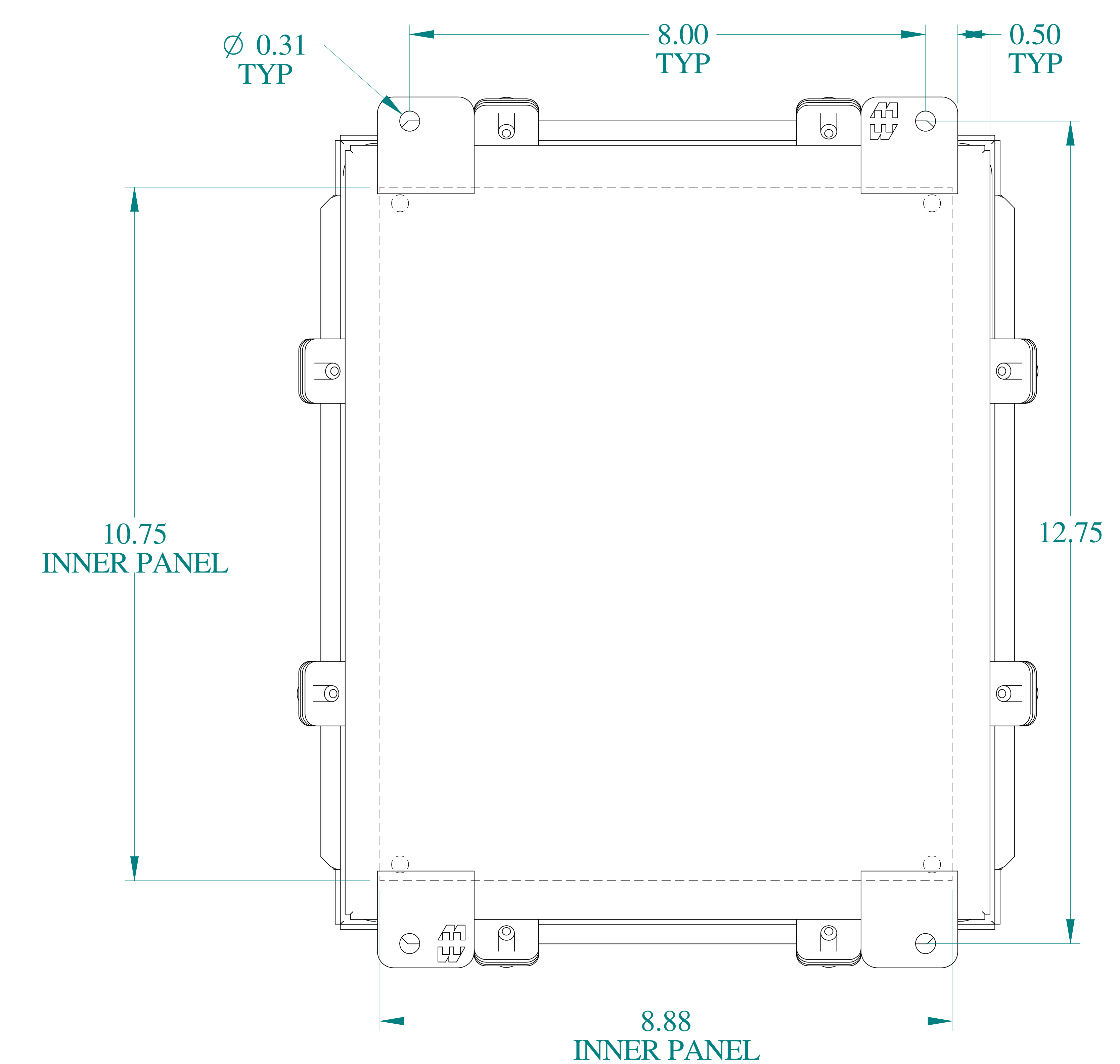
BACK VIEW
