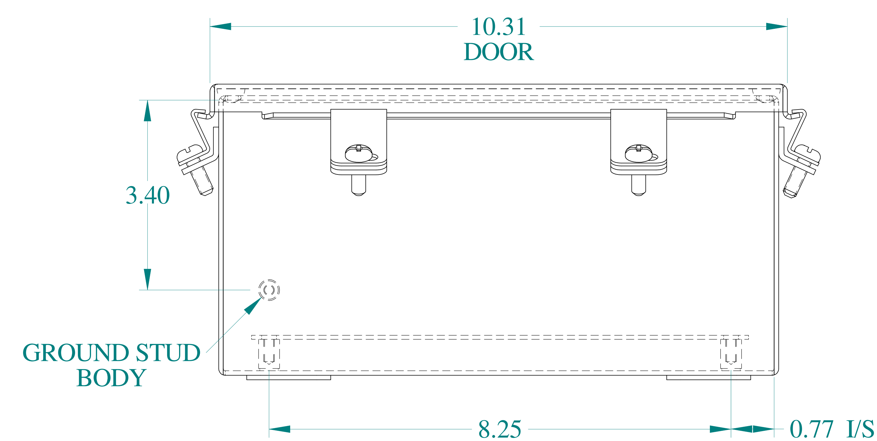
BOTTOM VIEW
