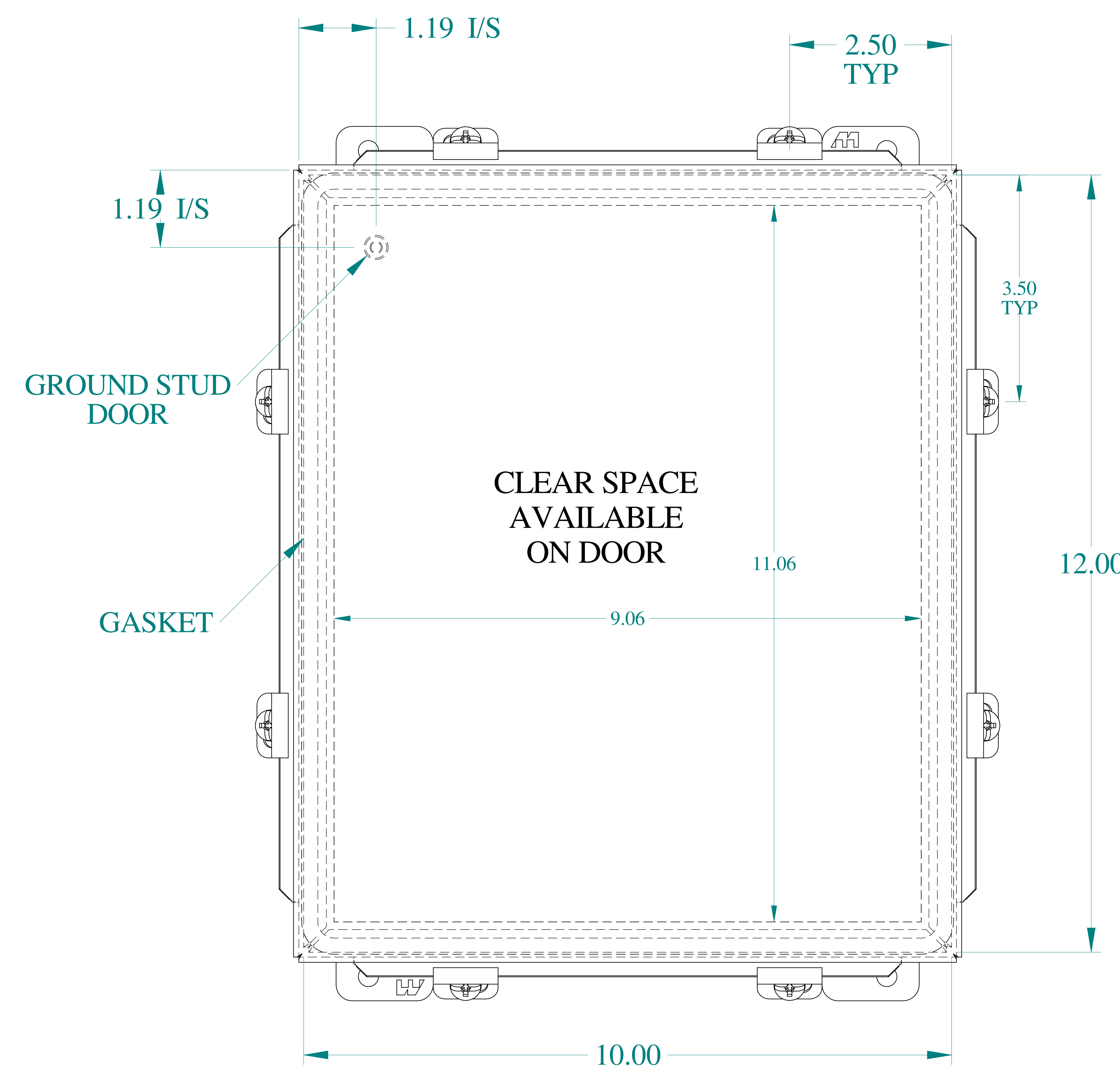
FRONT VIEW
