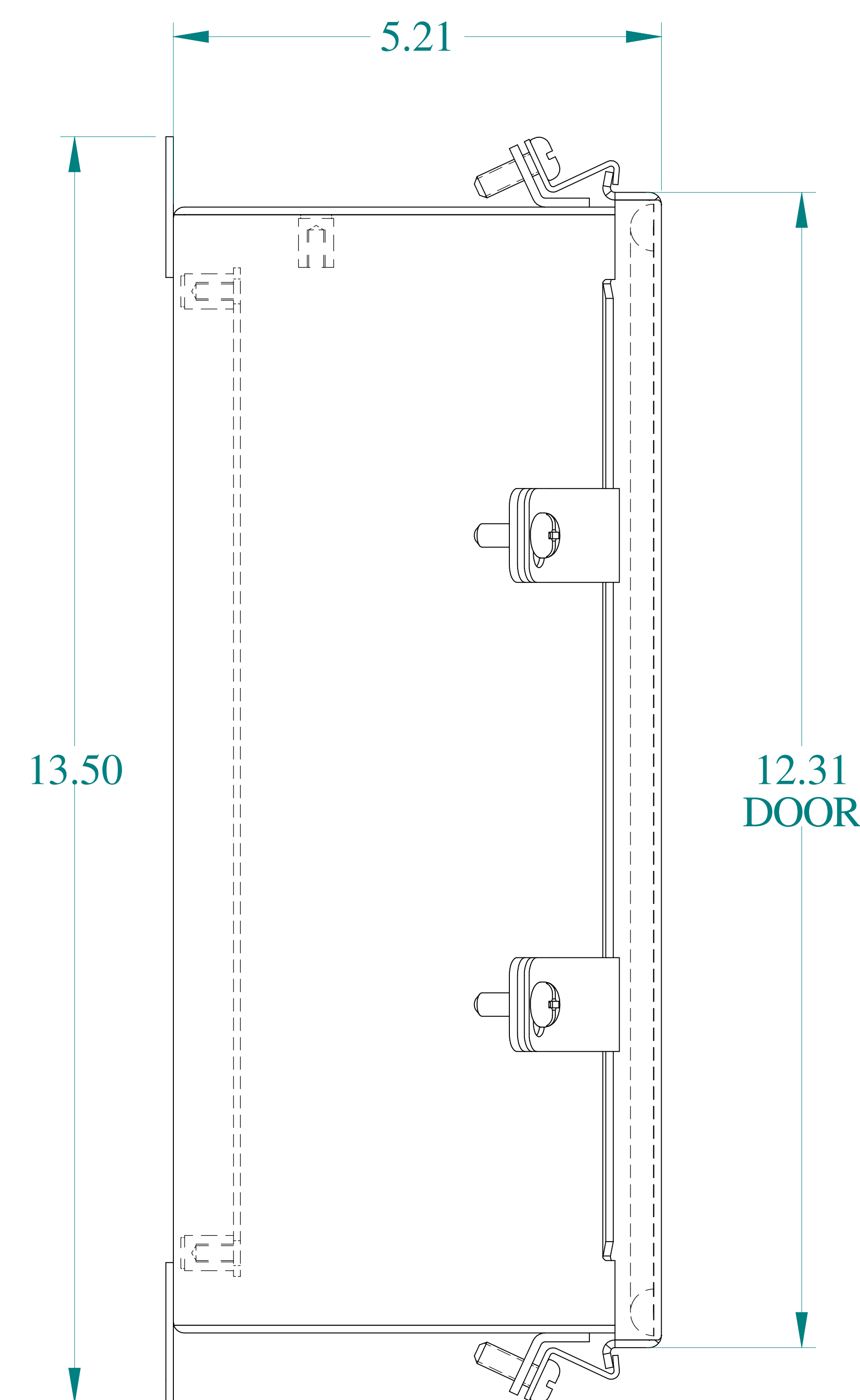
SIDE VIEW
