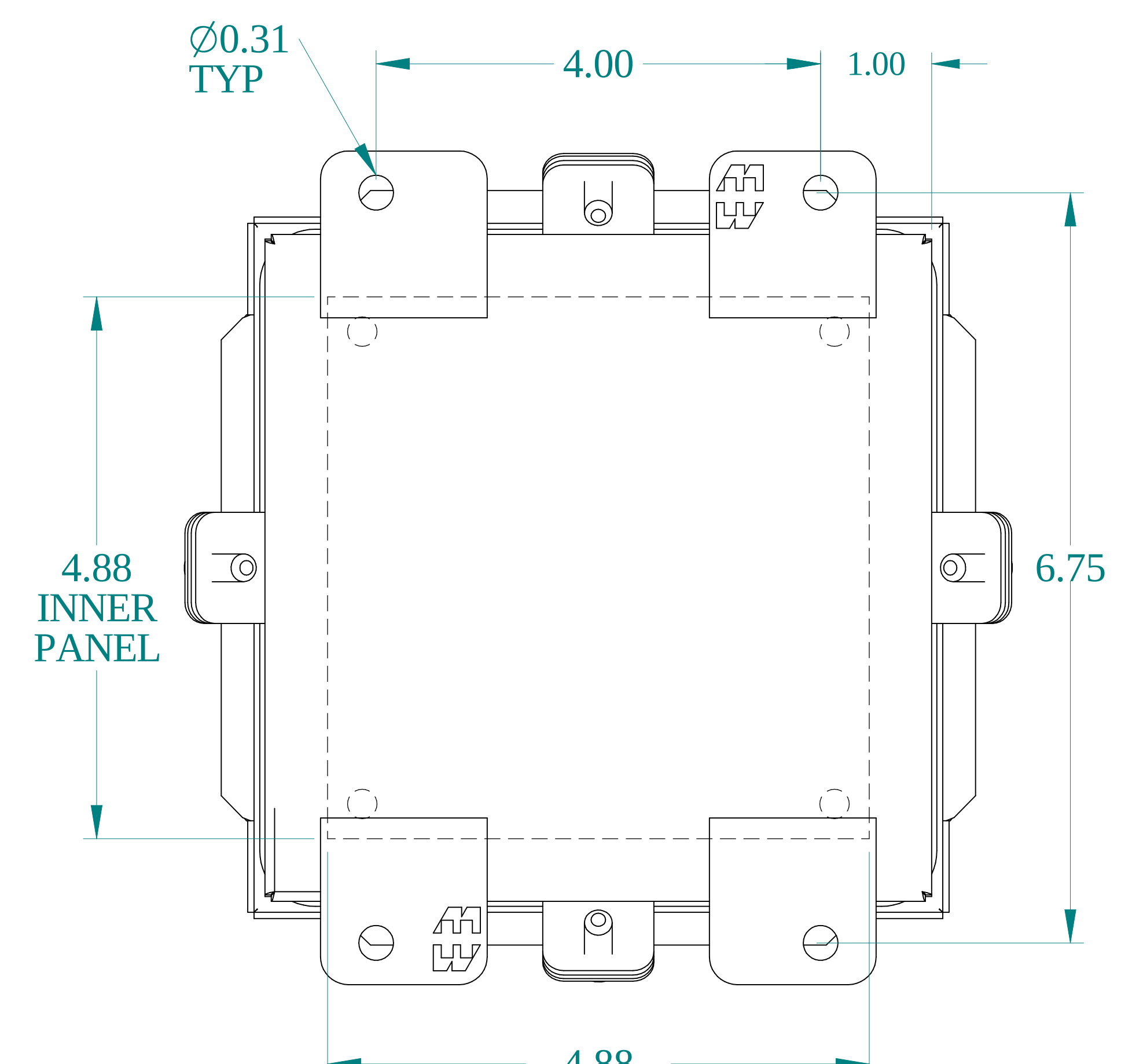
BACK VIEW
