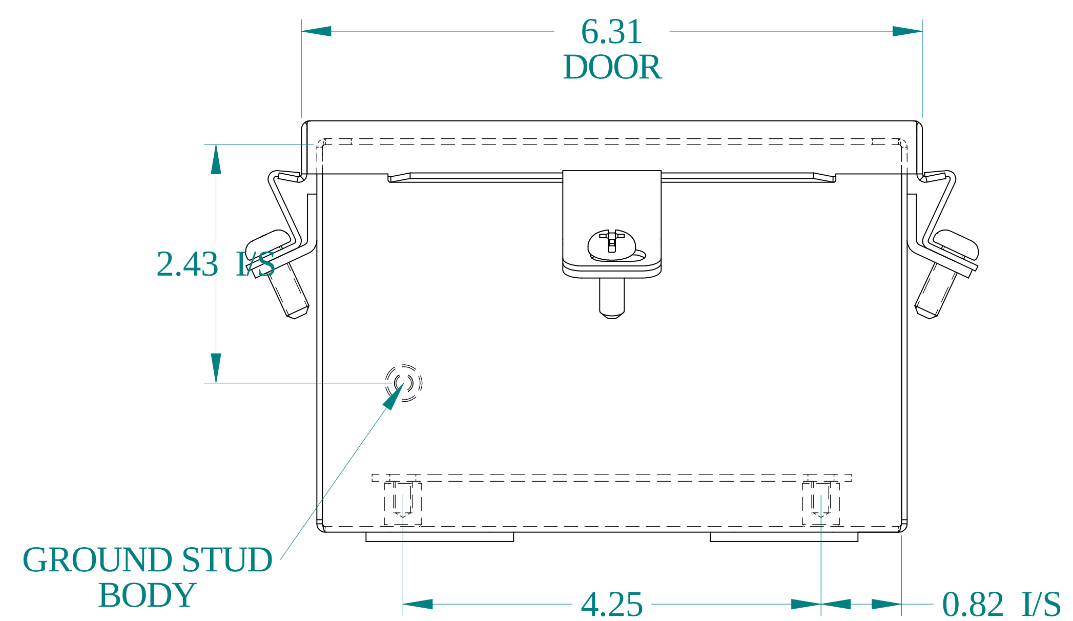
BOTTOM VIEW
