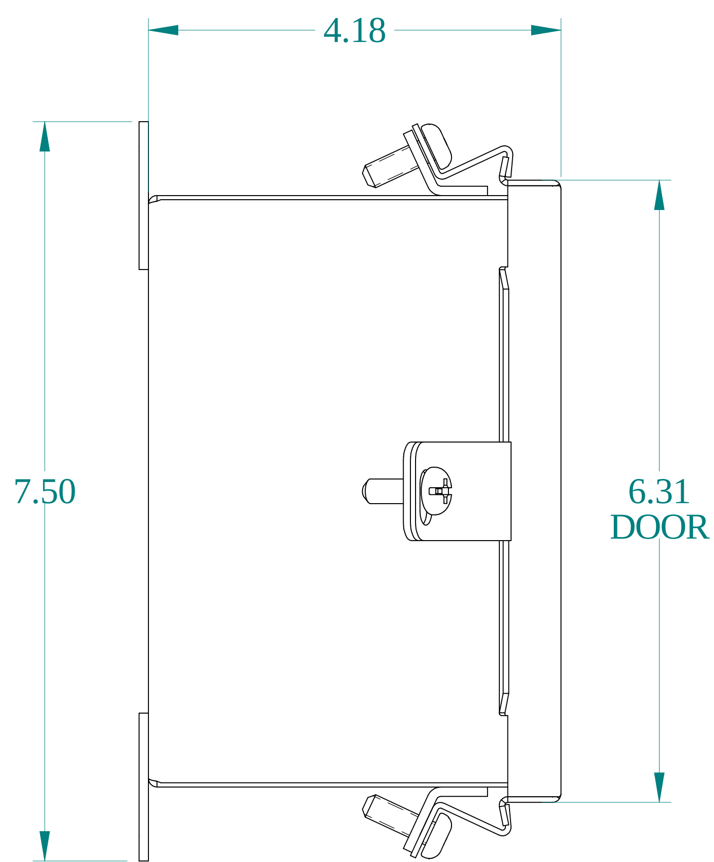
SIDE VIEW
