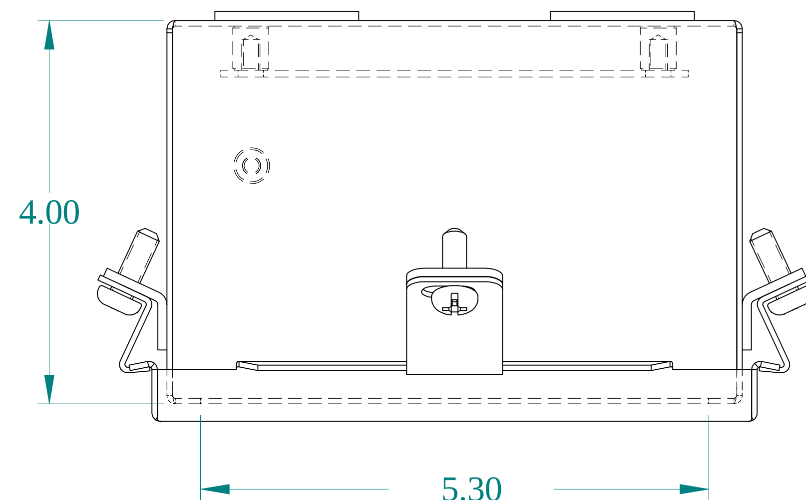
5.30 DOOR OPENING TOP VIEW
