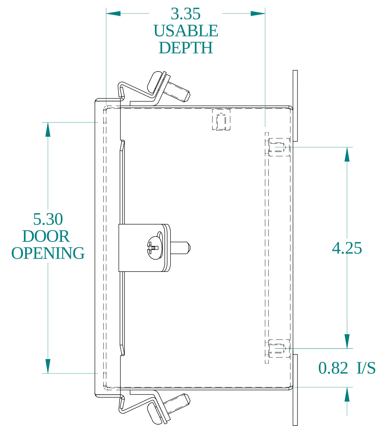
SIDE VIEW
