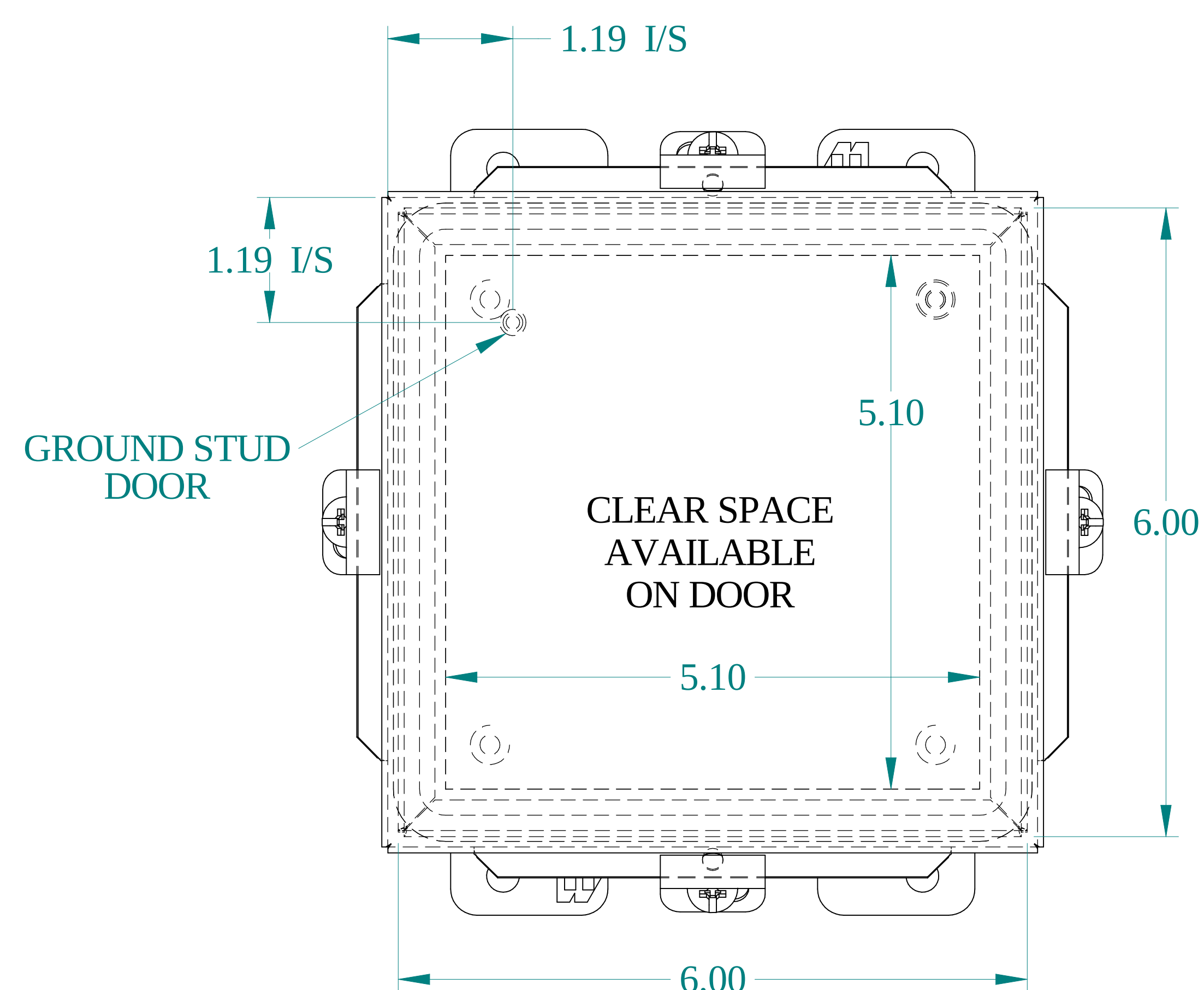
FRONT VIEW
