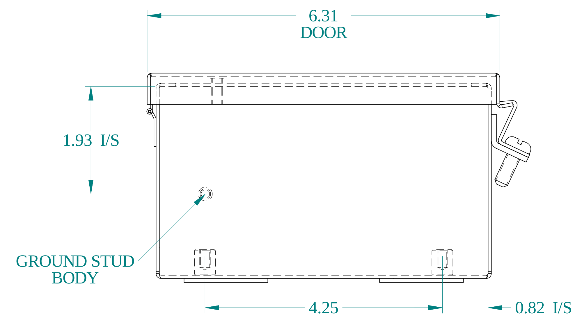
BOTTOM VIEW
