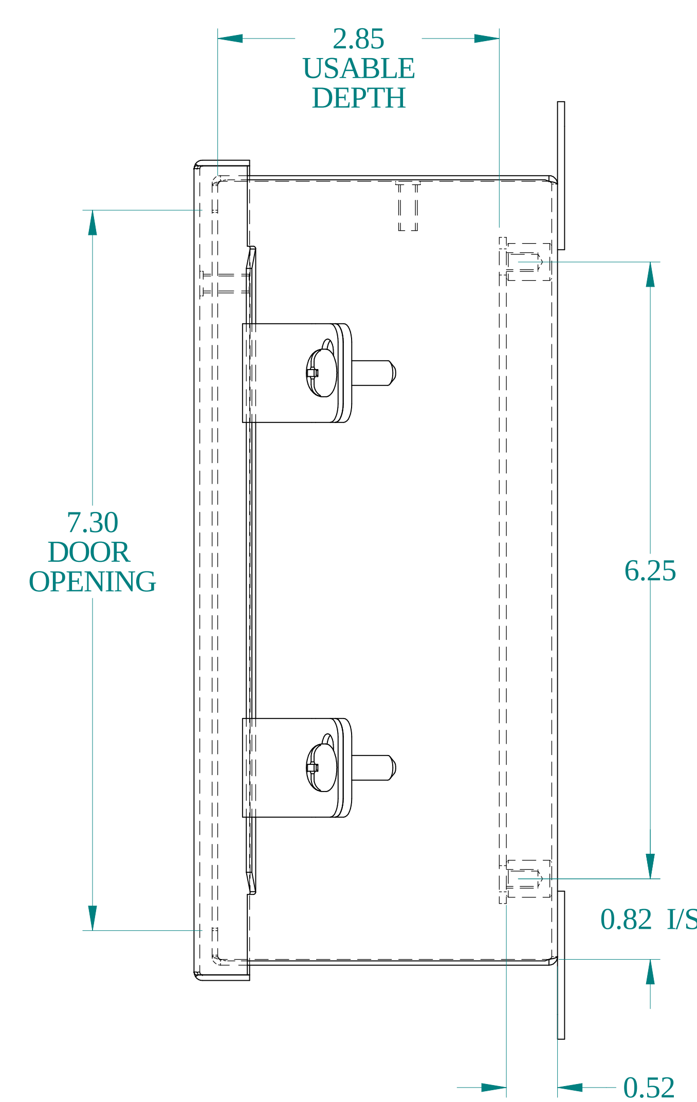
SIDE VIEW
