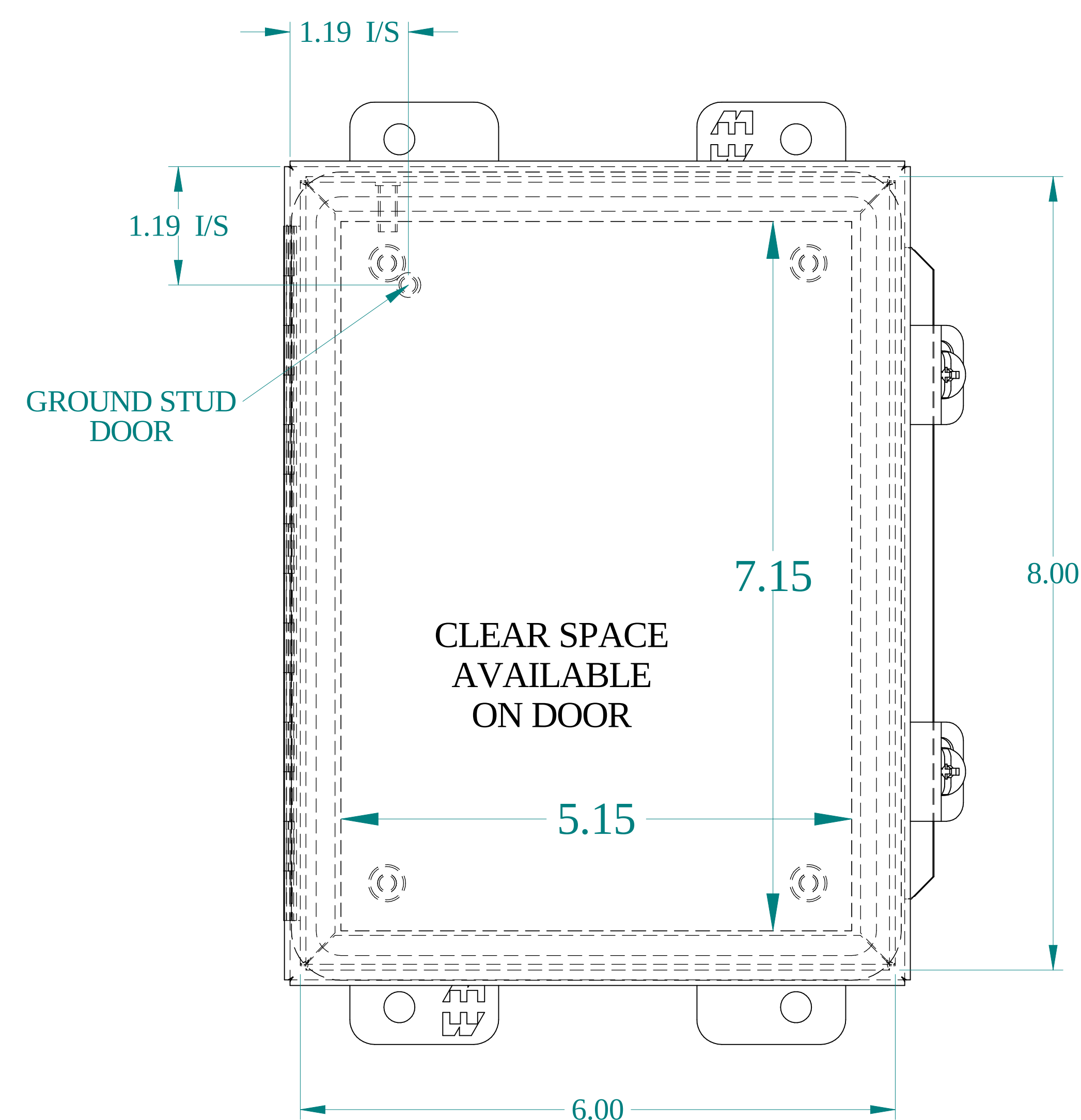
FRONT VIEW
