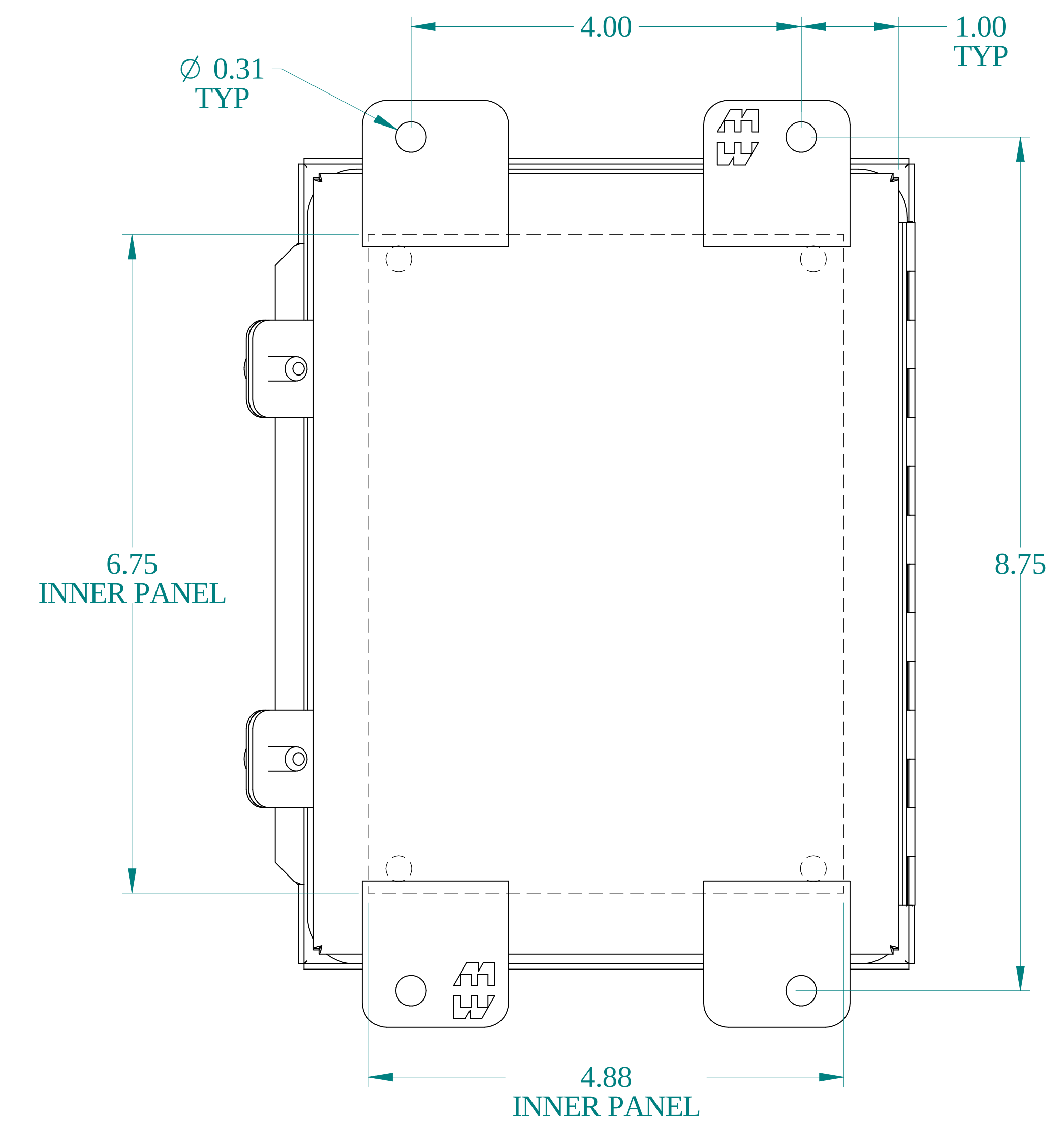
BACK VIEW
