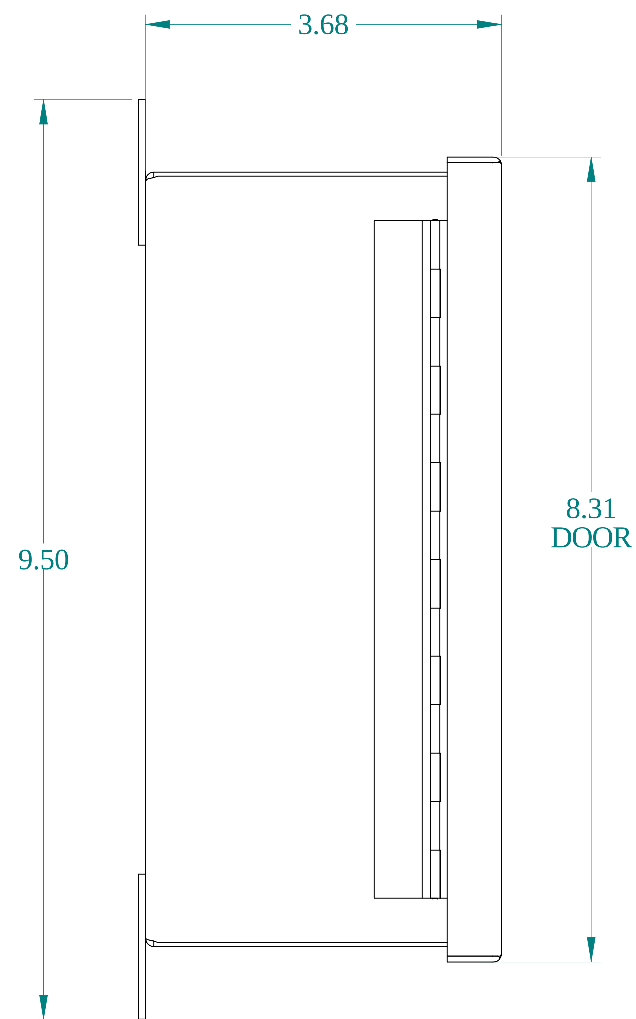
SIDE VIEW
