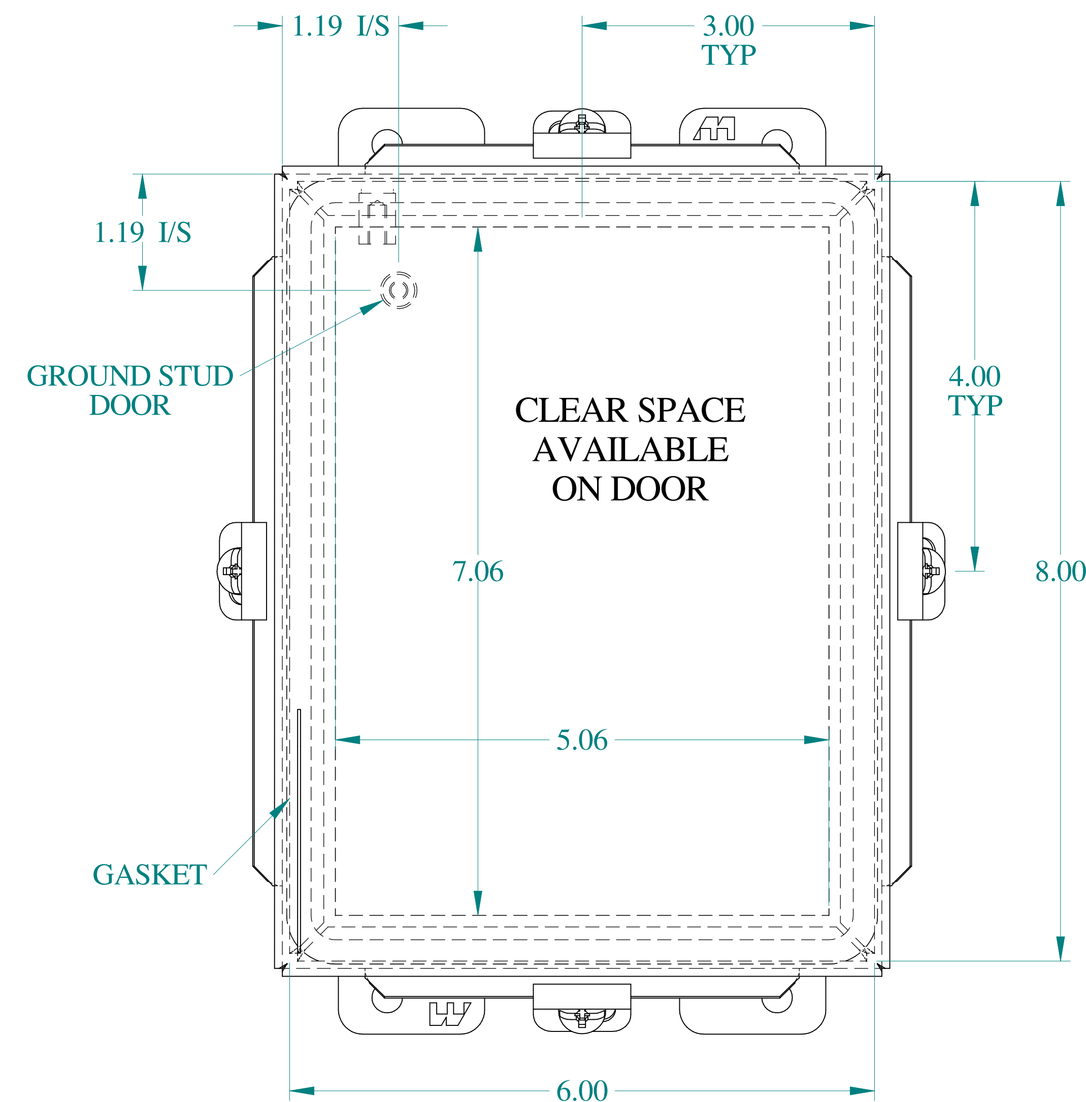
FRONT VIEW
