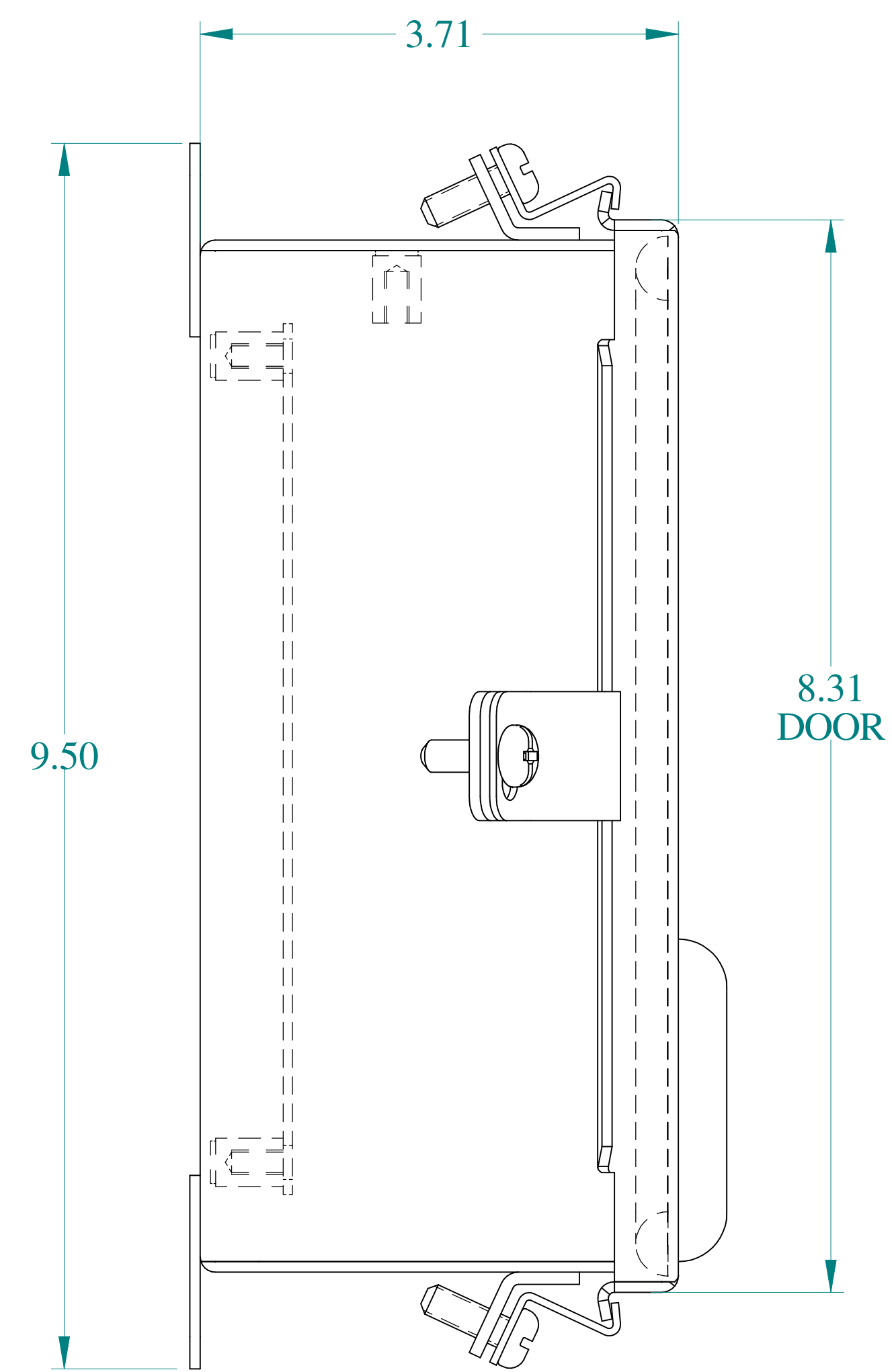
SIDE VIEW
