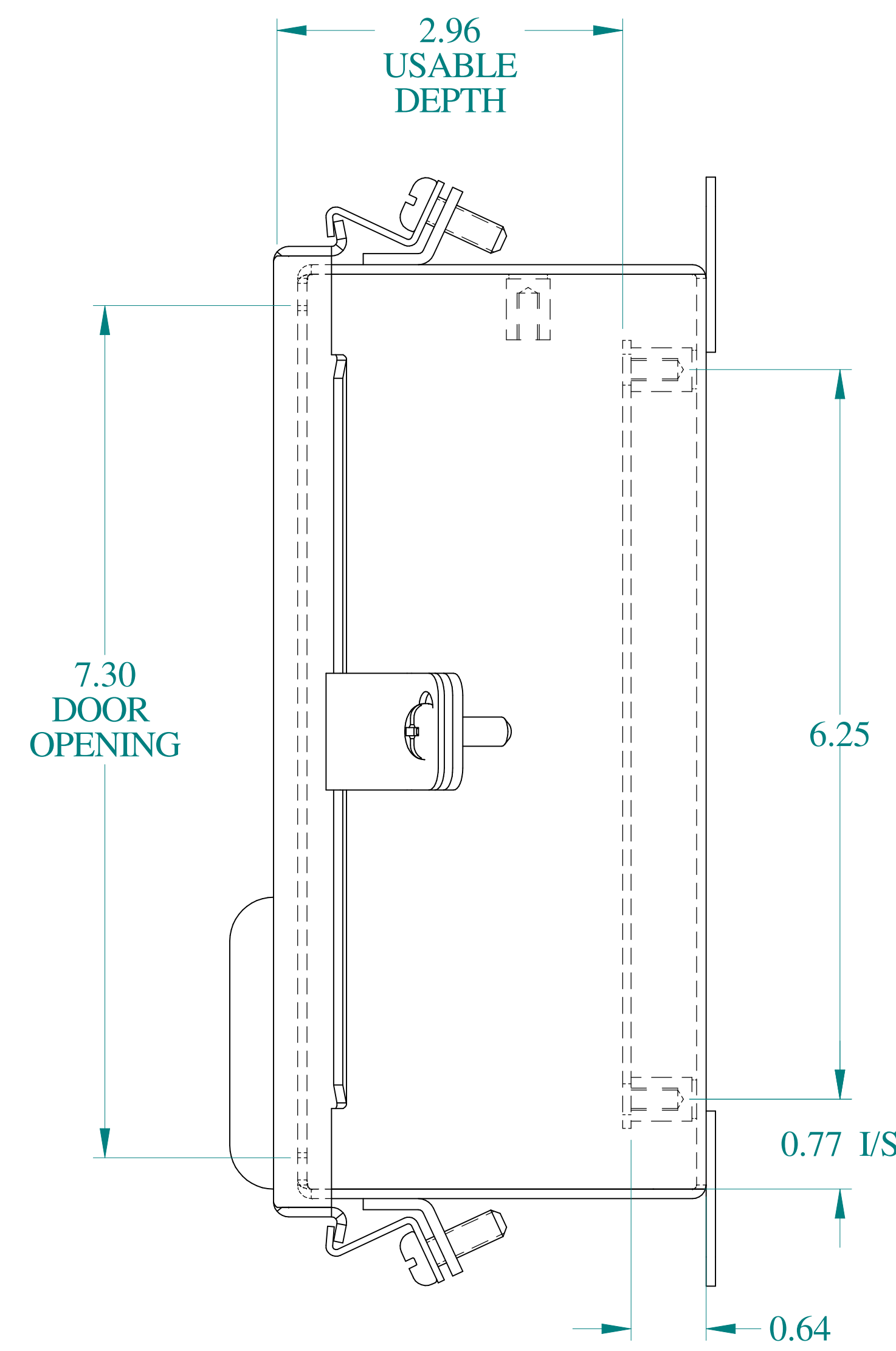
SIDE VIEW
