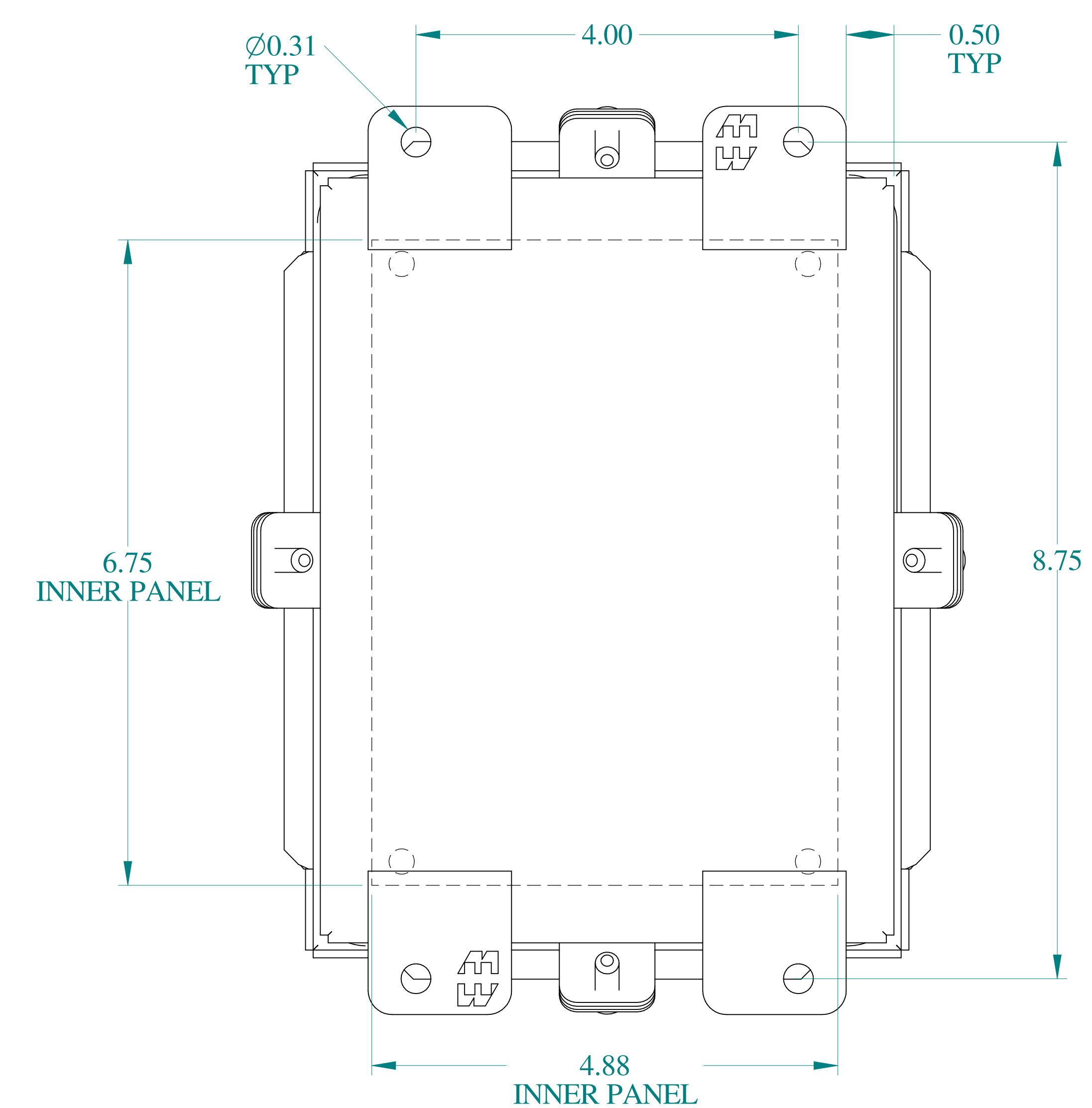
BACK VIEW
