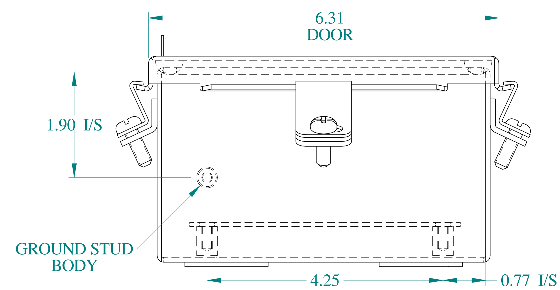
BOTTOM VIEW
