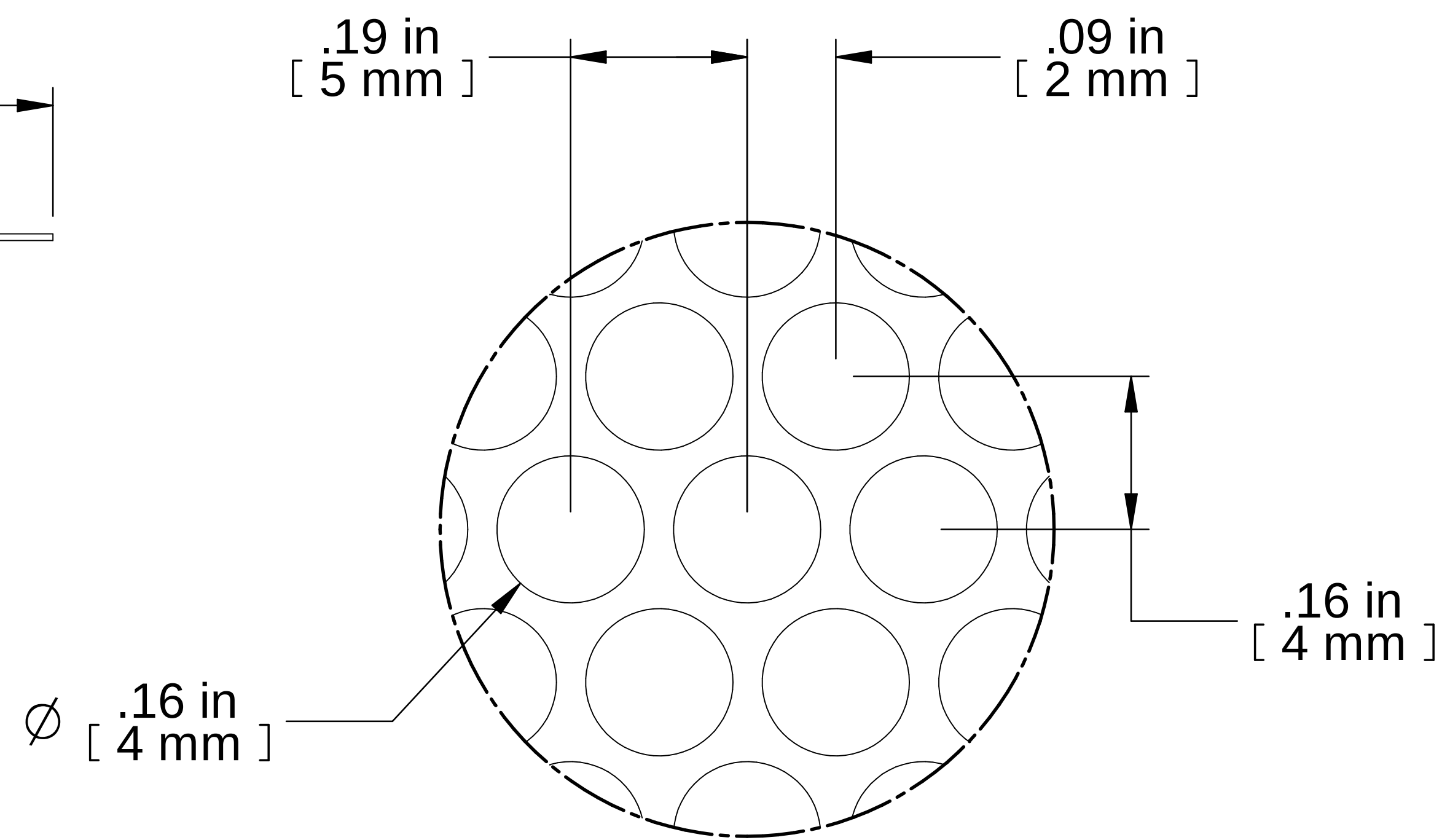
DETAIL A (ENTIRE PANEL PERFORATED)
