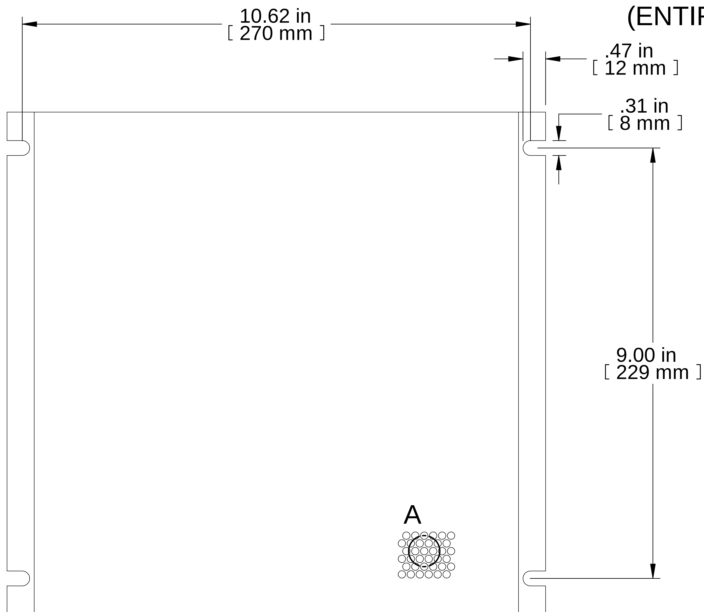
FRONT VIEW
