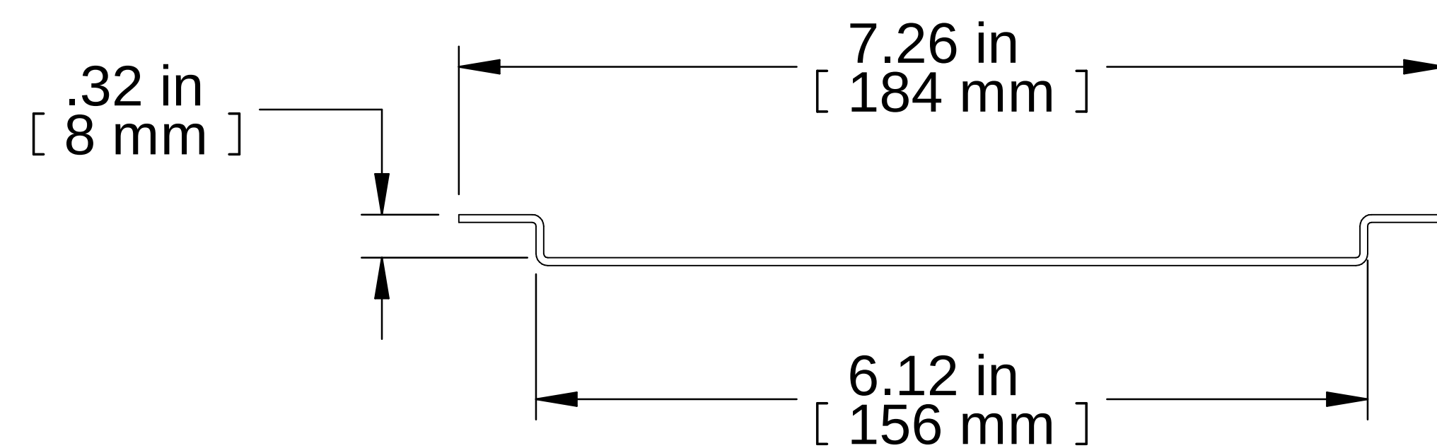
TOP VIEW
