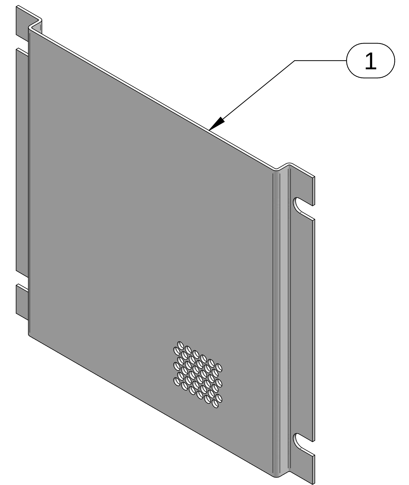
ISOMETRIC
