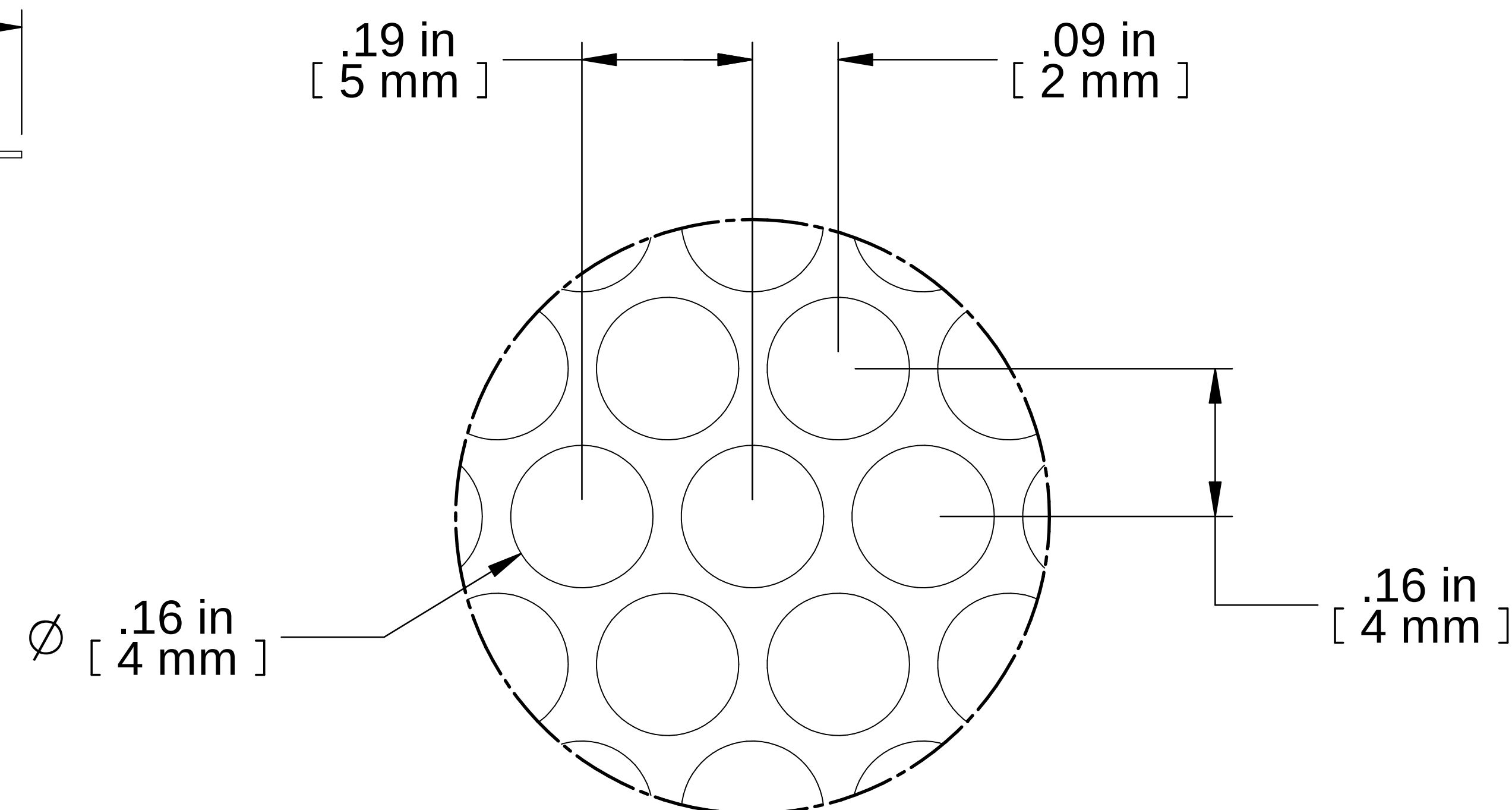
DETAIL A (ENTIRE PANEL PERFORATED)
