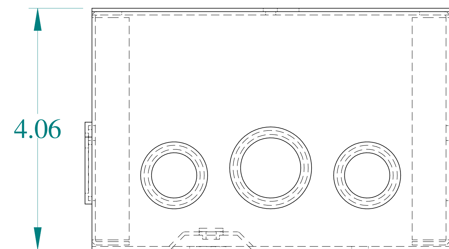
SIDE VIEW
