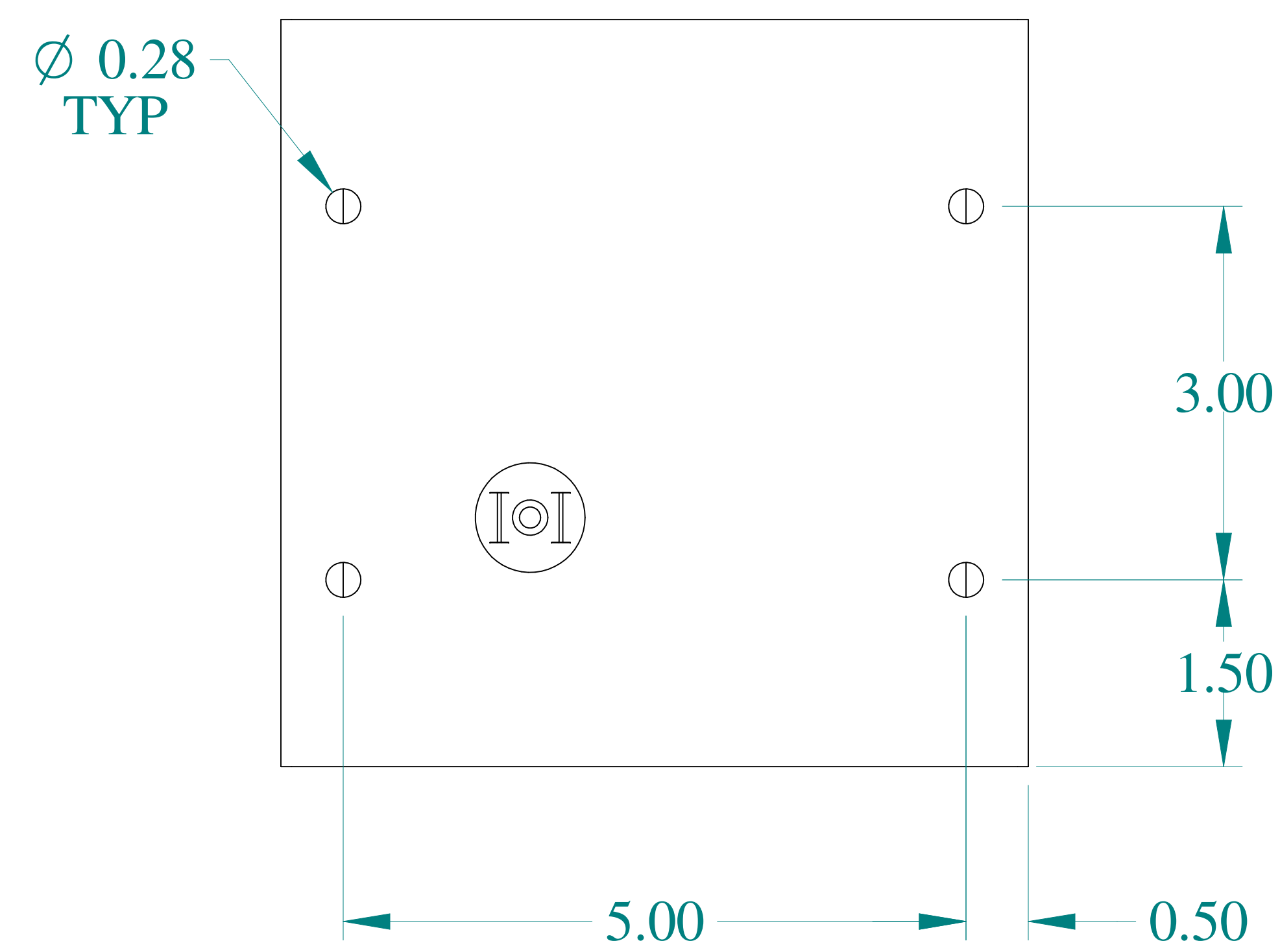
BOTTOM VIEW
