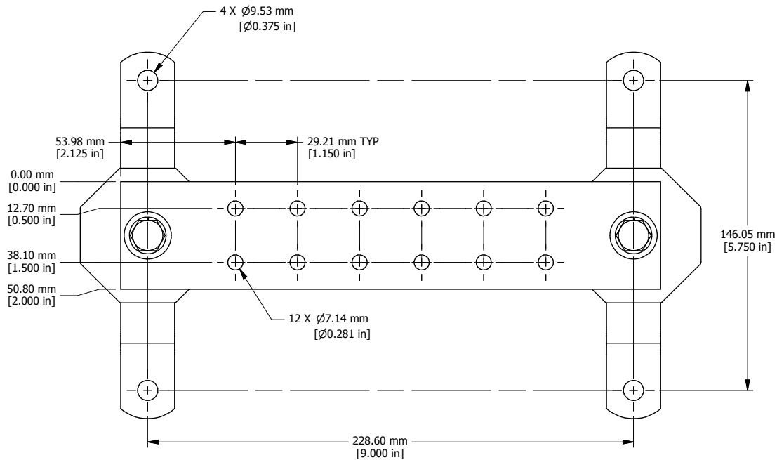
ASSEMBLY - TOP VIEW
