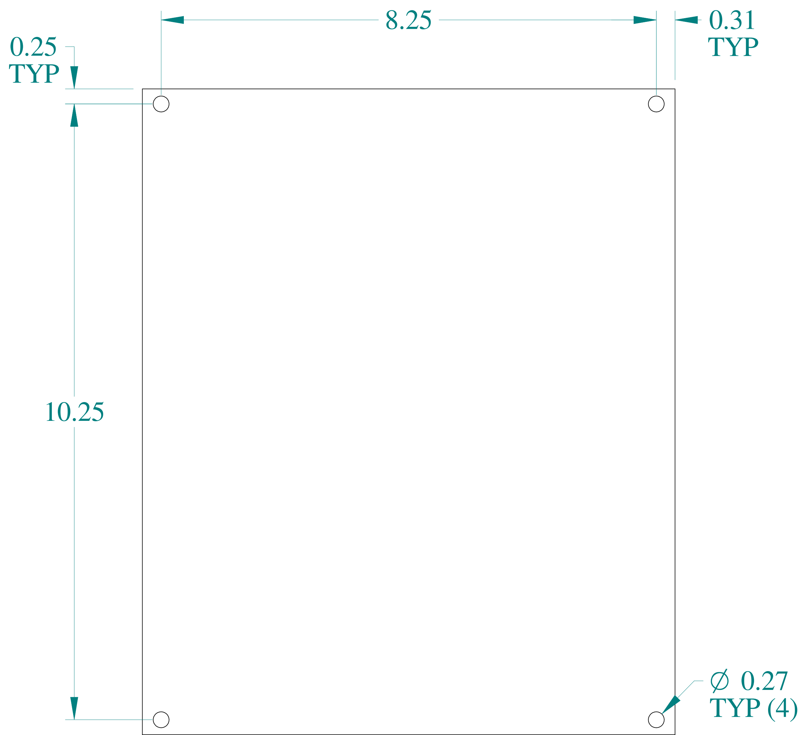
FRONT VIEW
