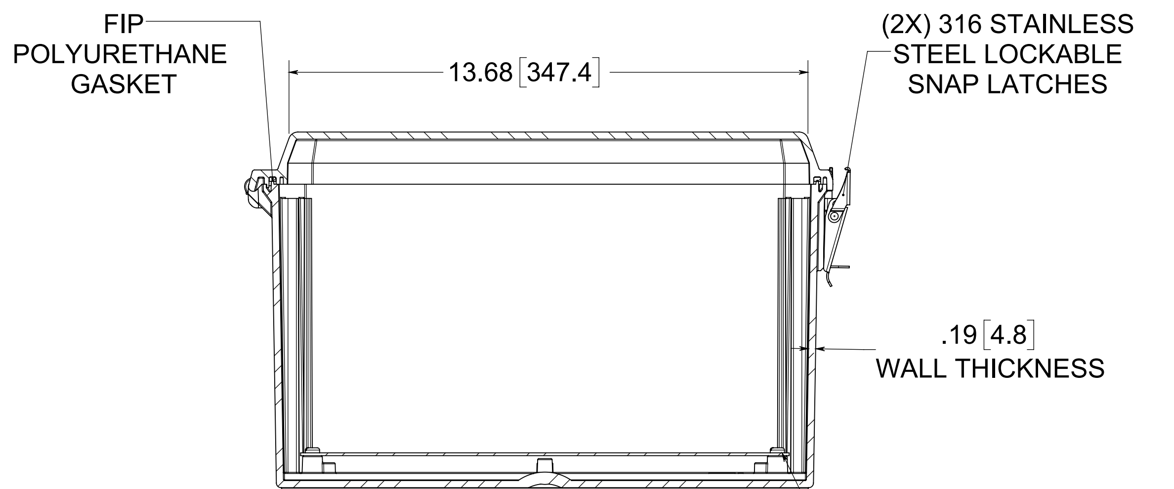
SECTION B-B
