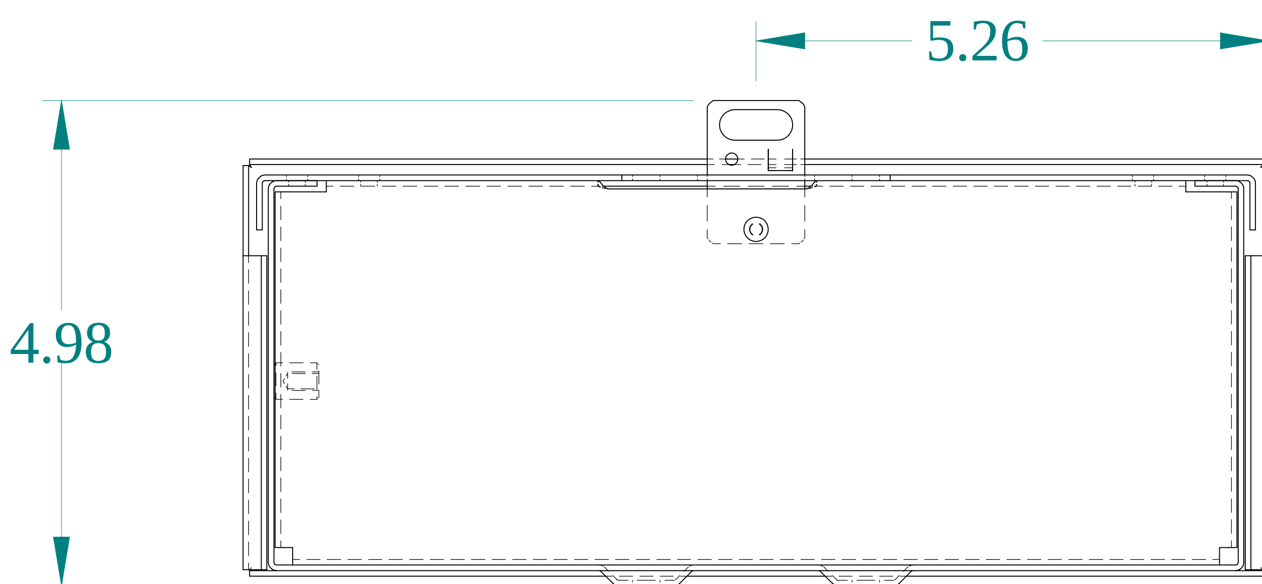
BOTTOM VIEW
