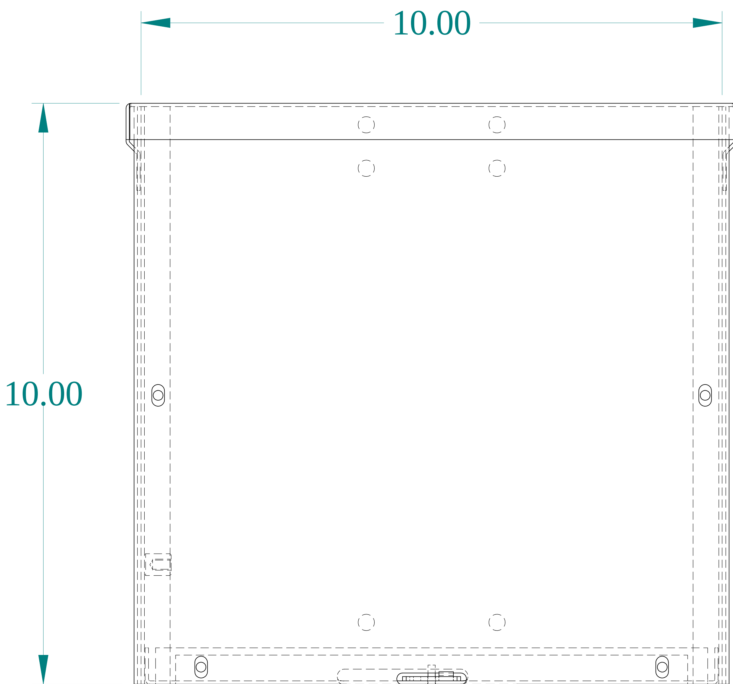
FRONT VIEW
