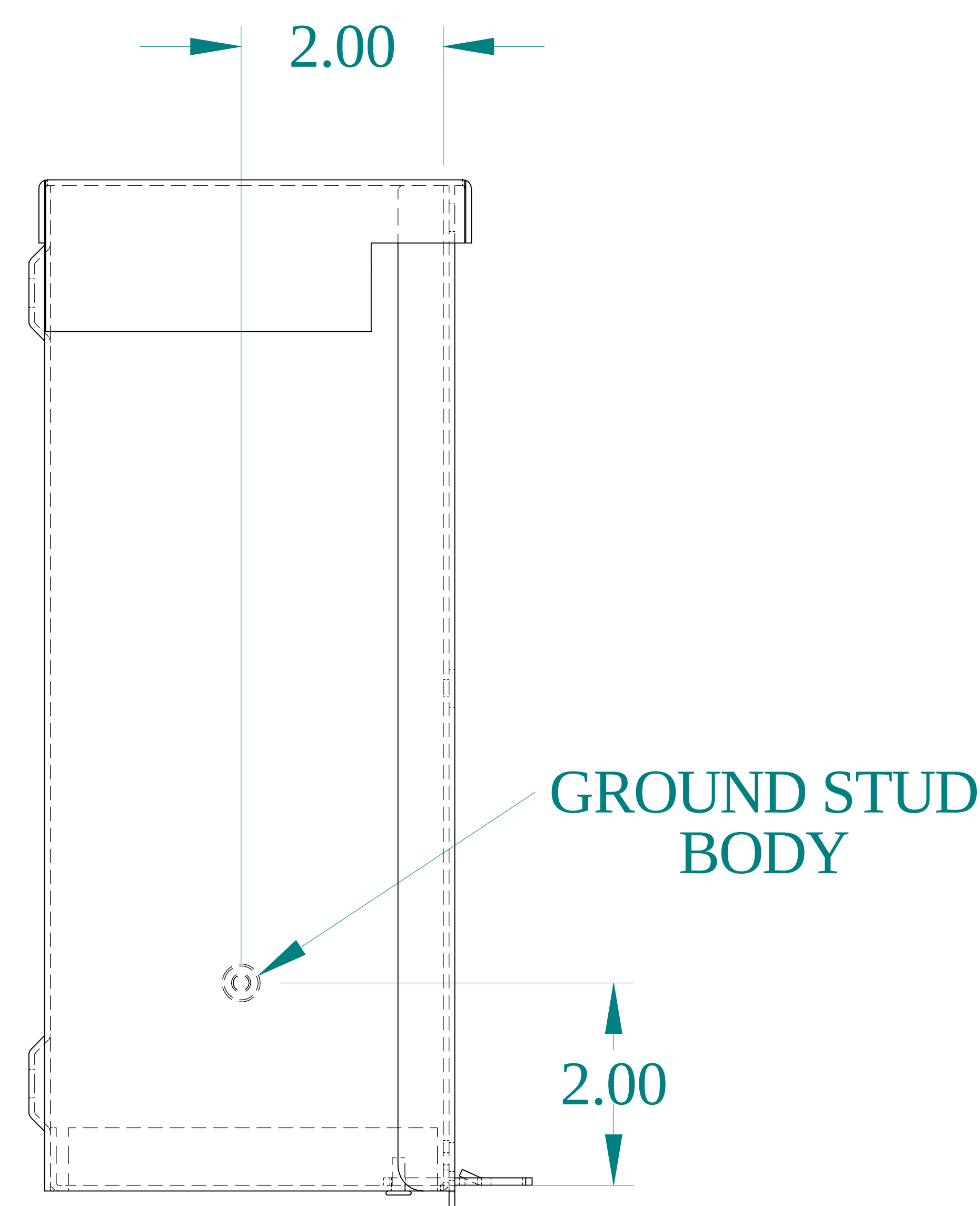
SIDE VIEW
