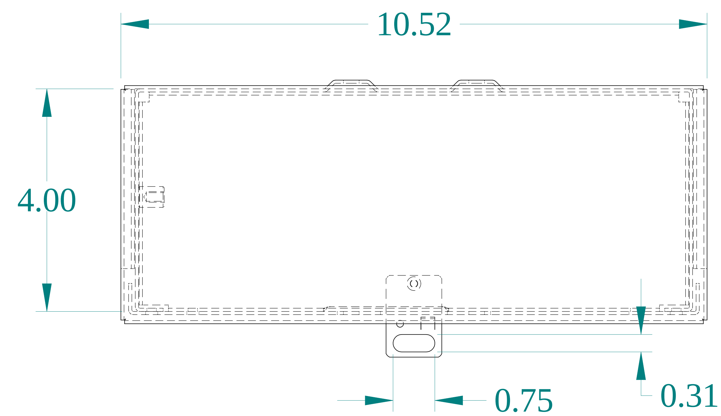
TOP VIEW
