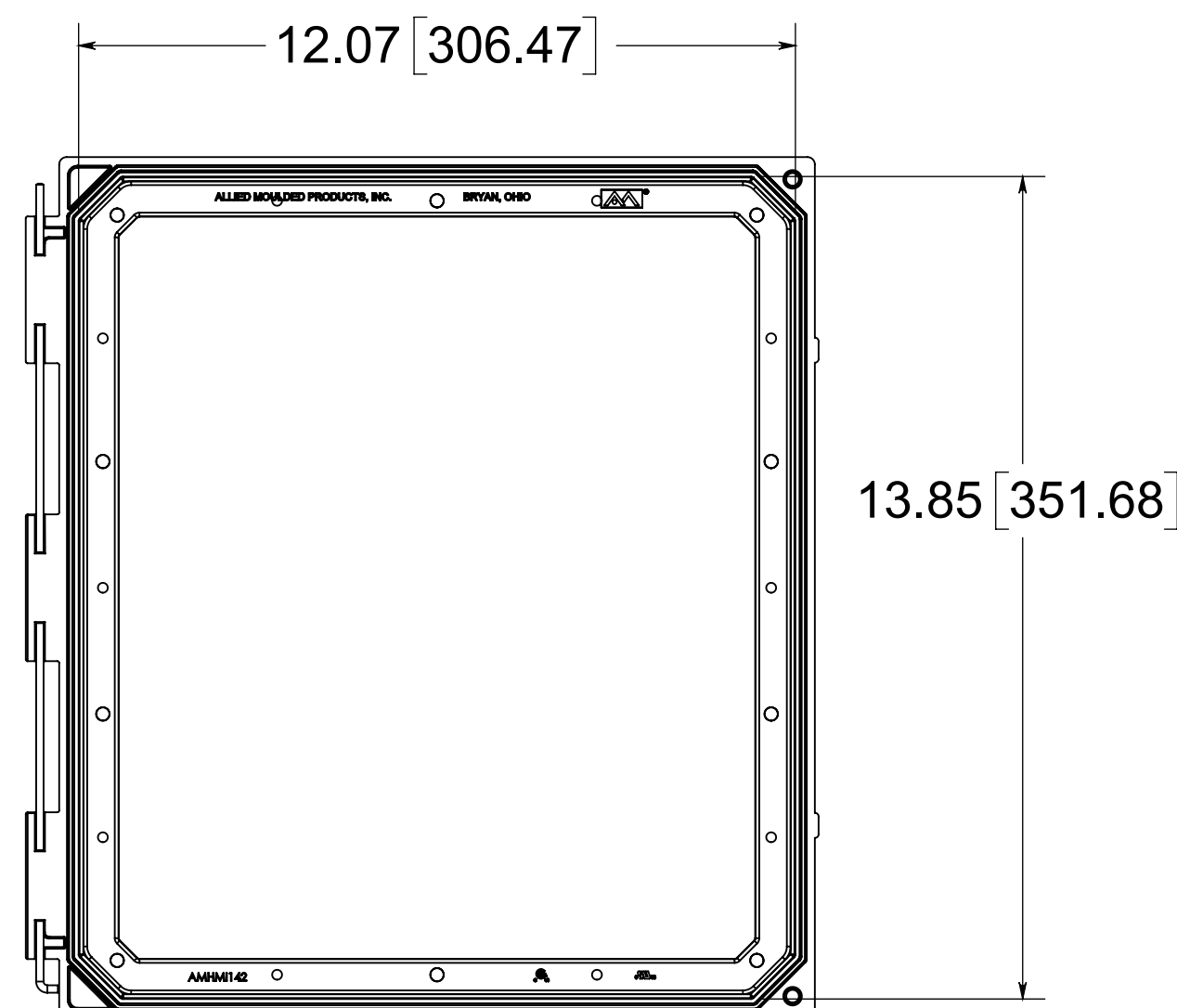
FRONT VIEW WITH COVER REMOVED
