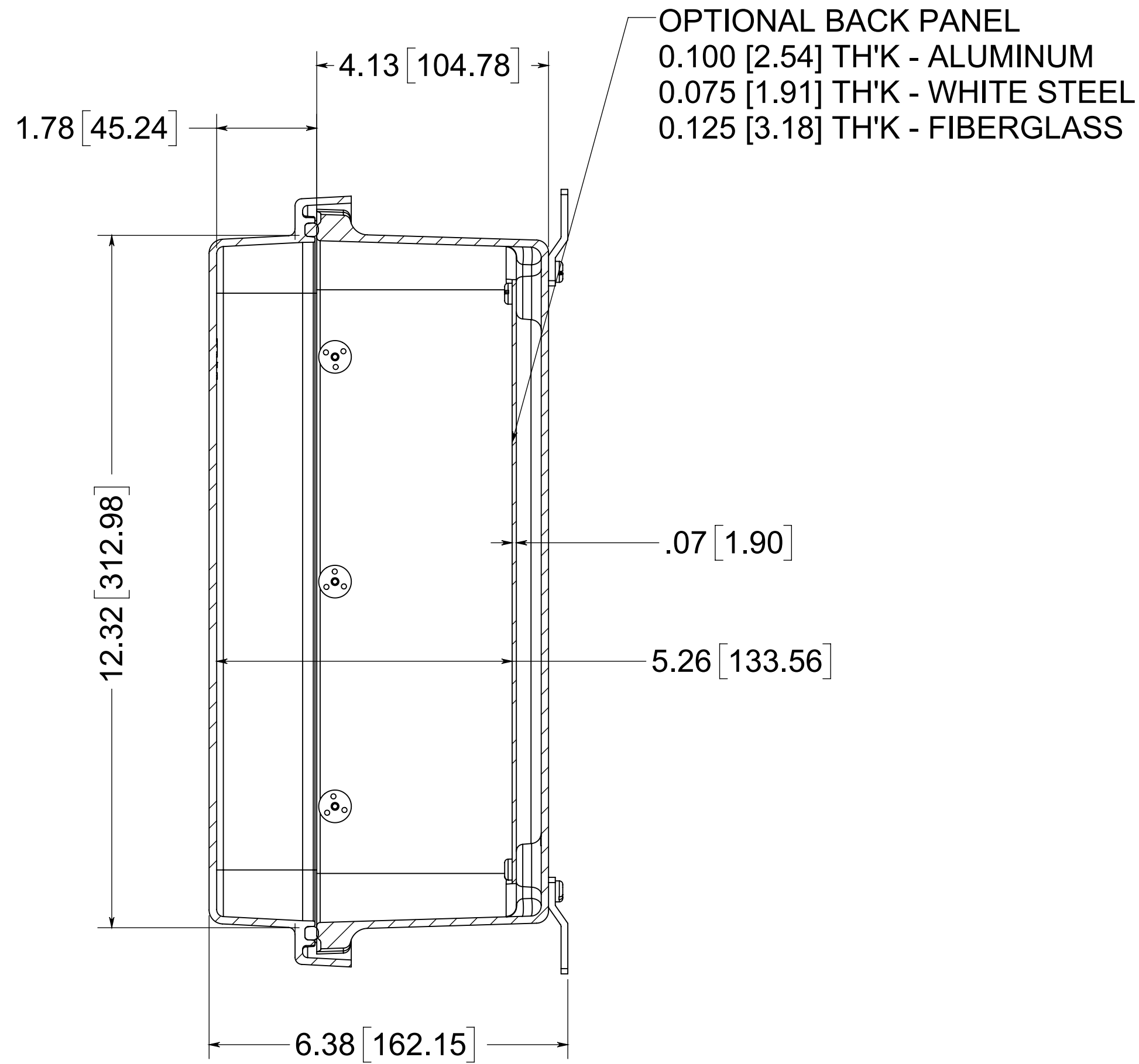
SECTION B-B
