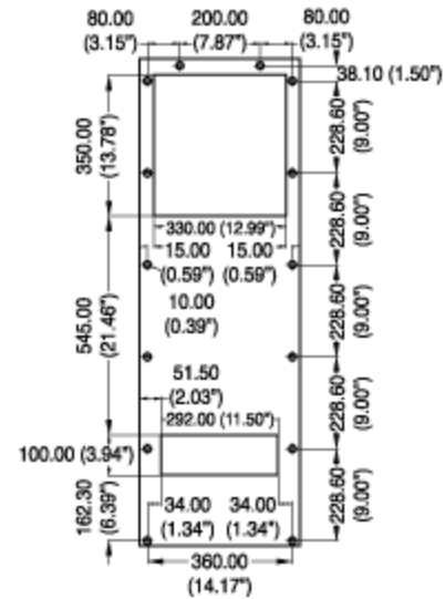
Drilling Template
