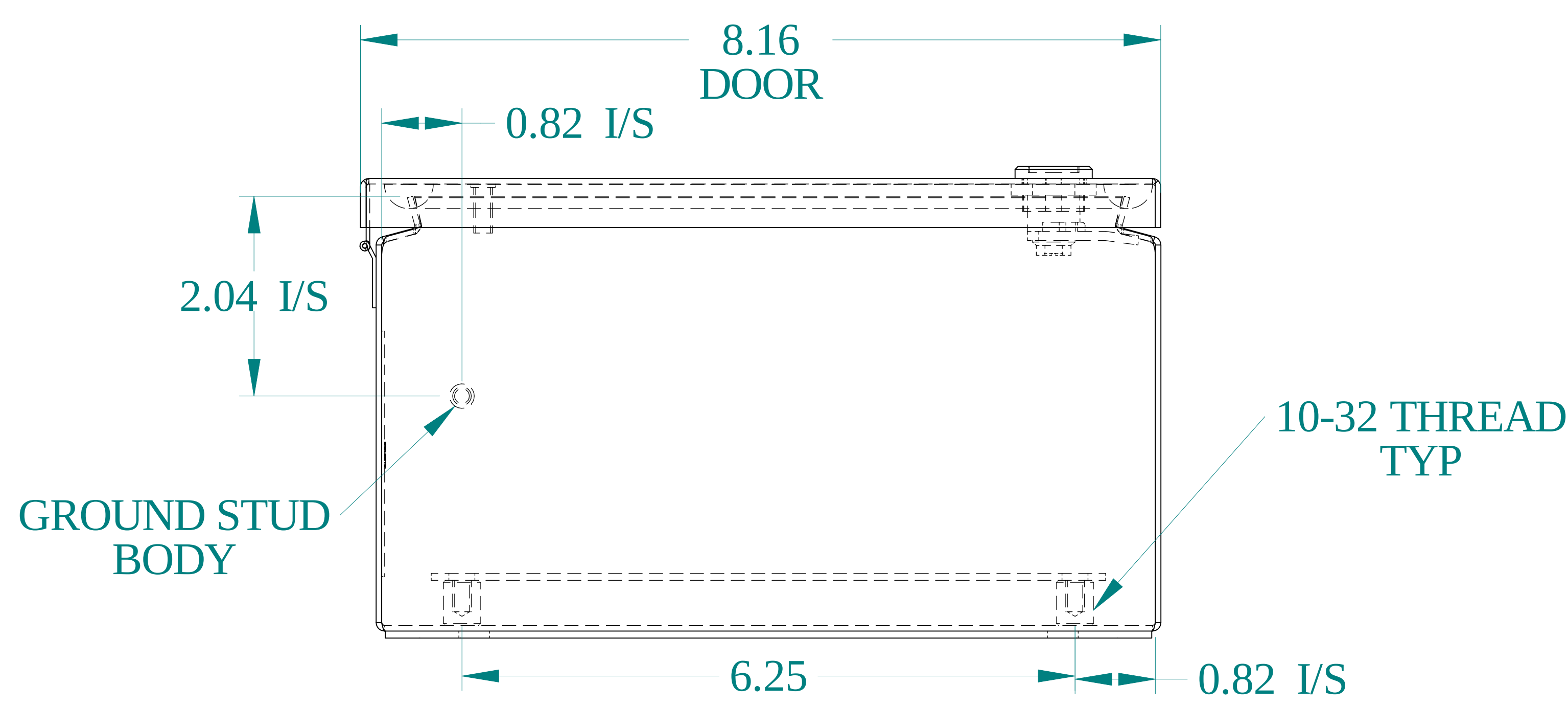
BOTTOM VIEW
