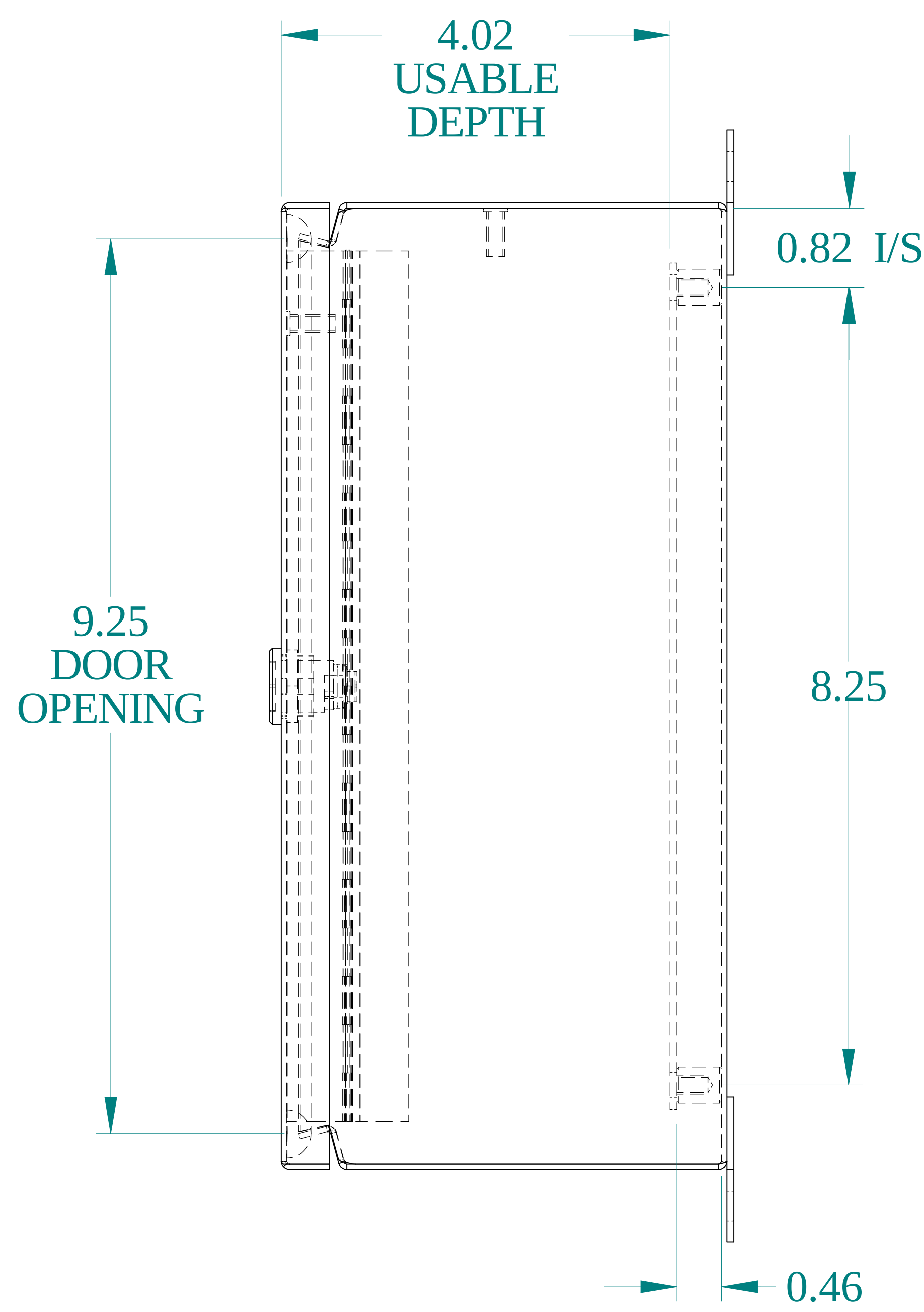
SIDE VIEW
