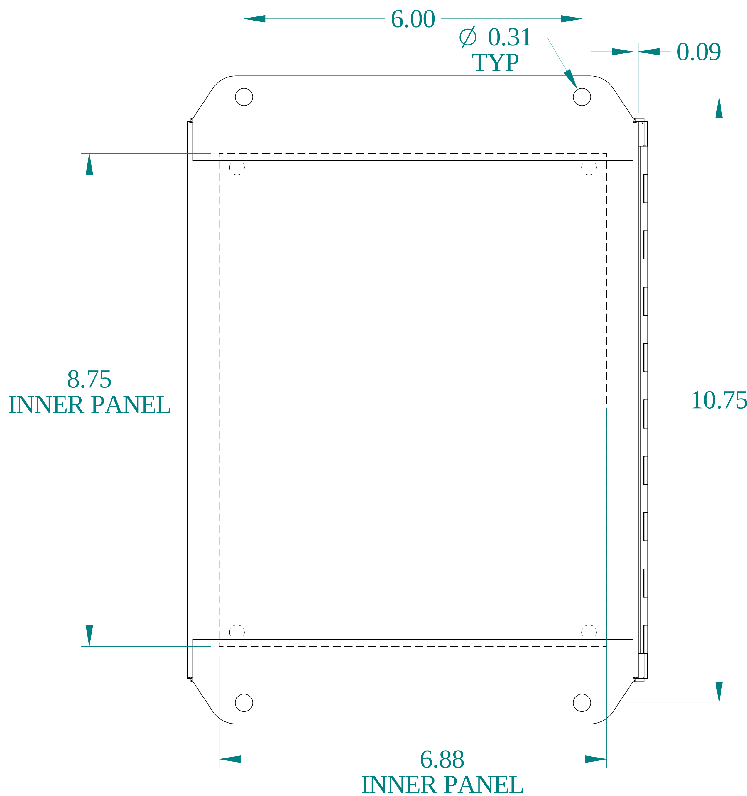
BACK VIEW
