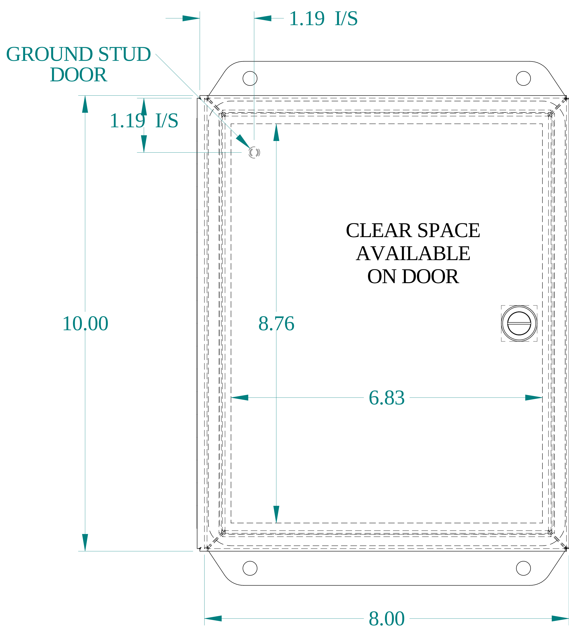
FRONT VIEW
