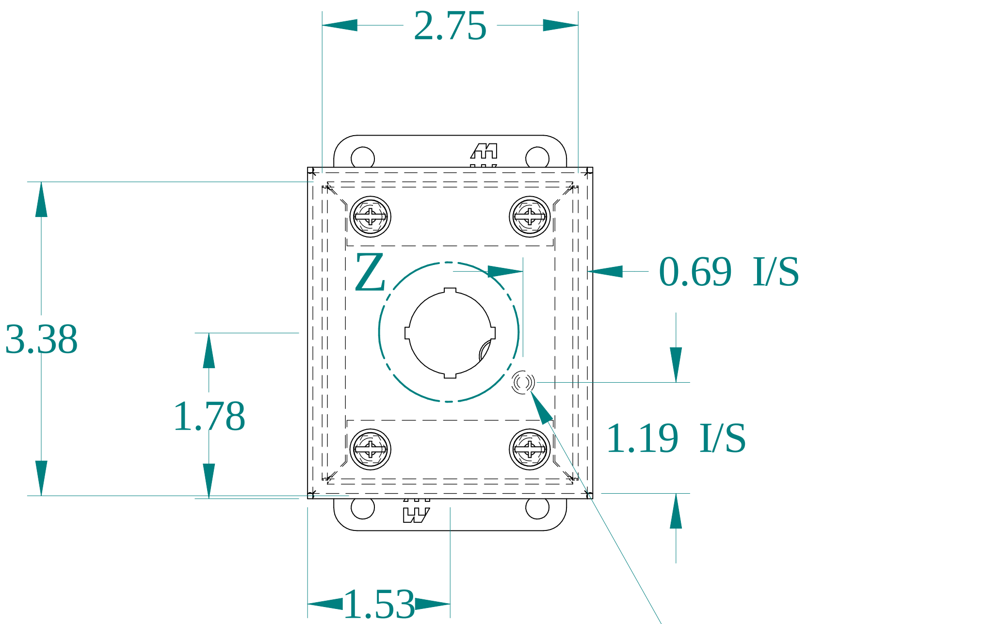
FRONT VIEW
