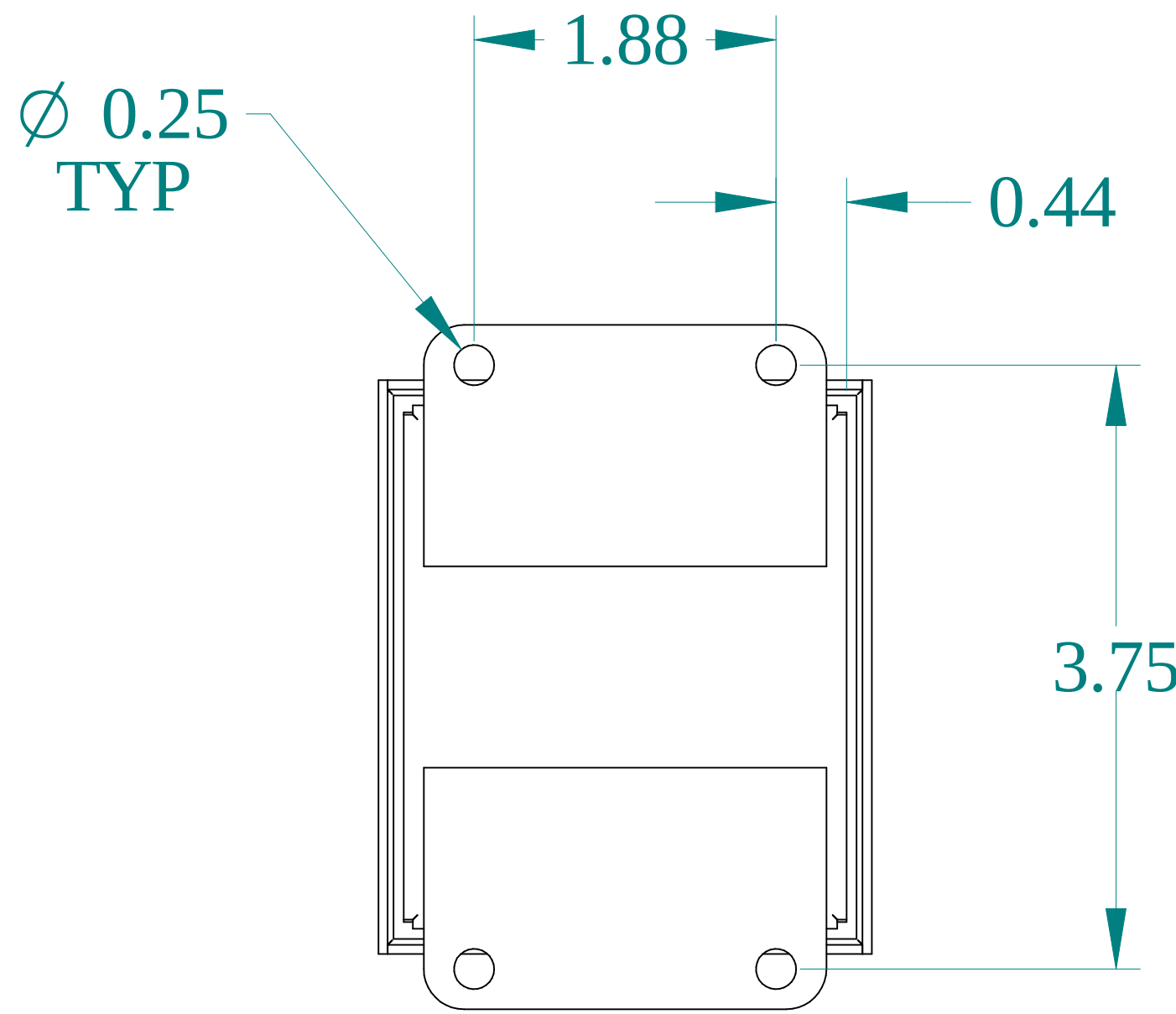
BACK VIEW
