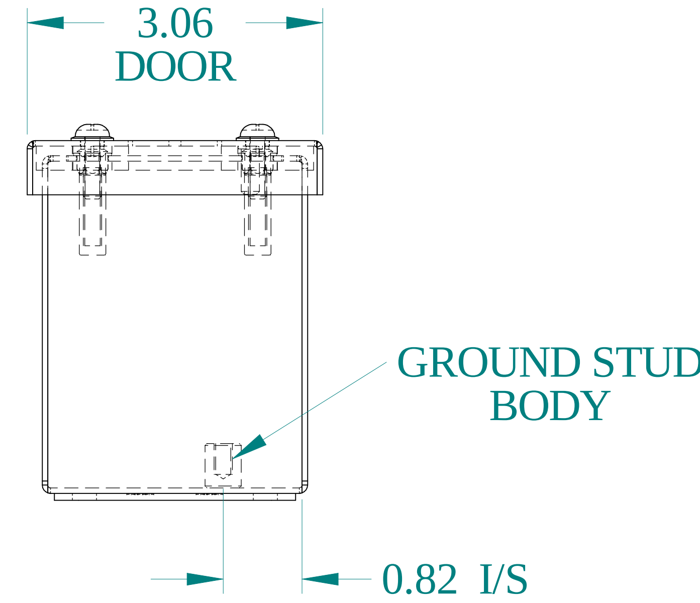
BOTTOM VIEW
