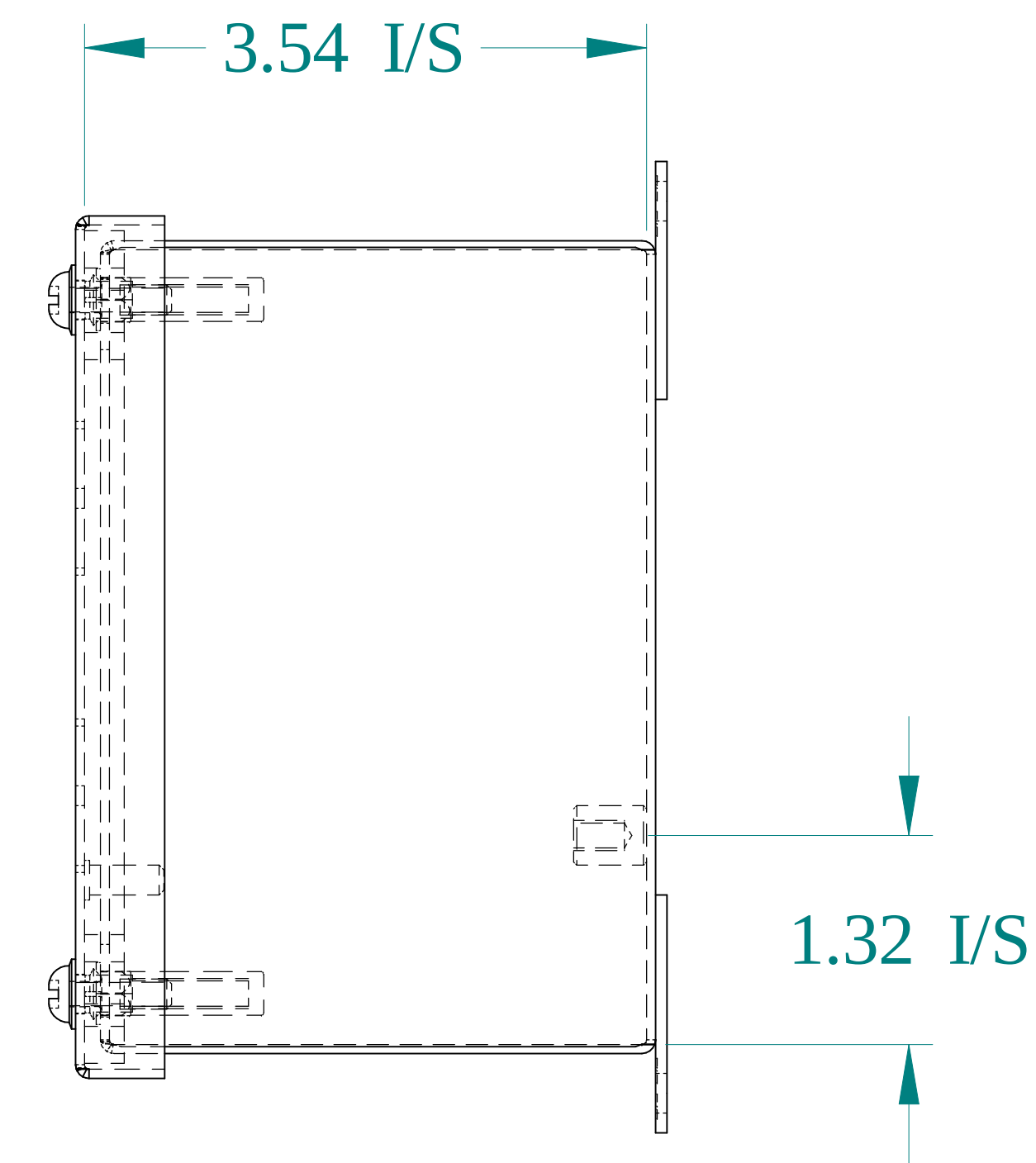
SIDE VIEW
