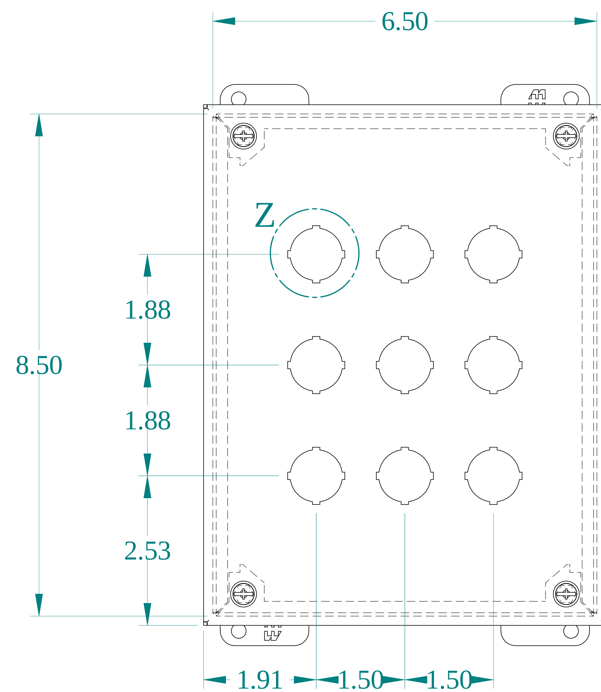
FRONT VIEW
