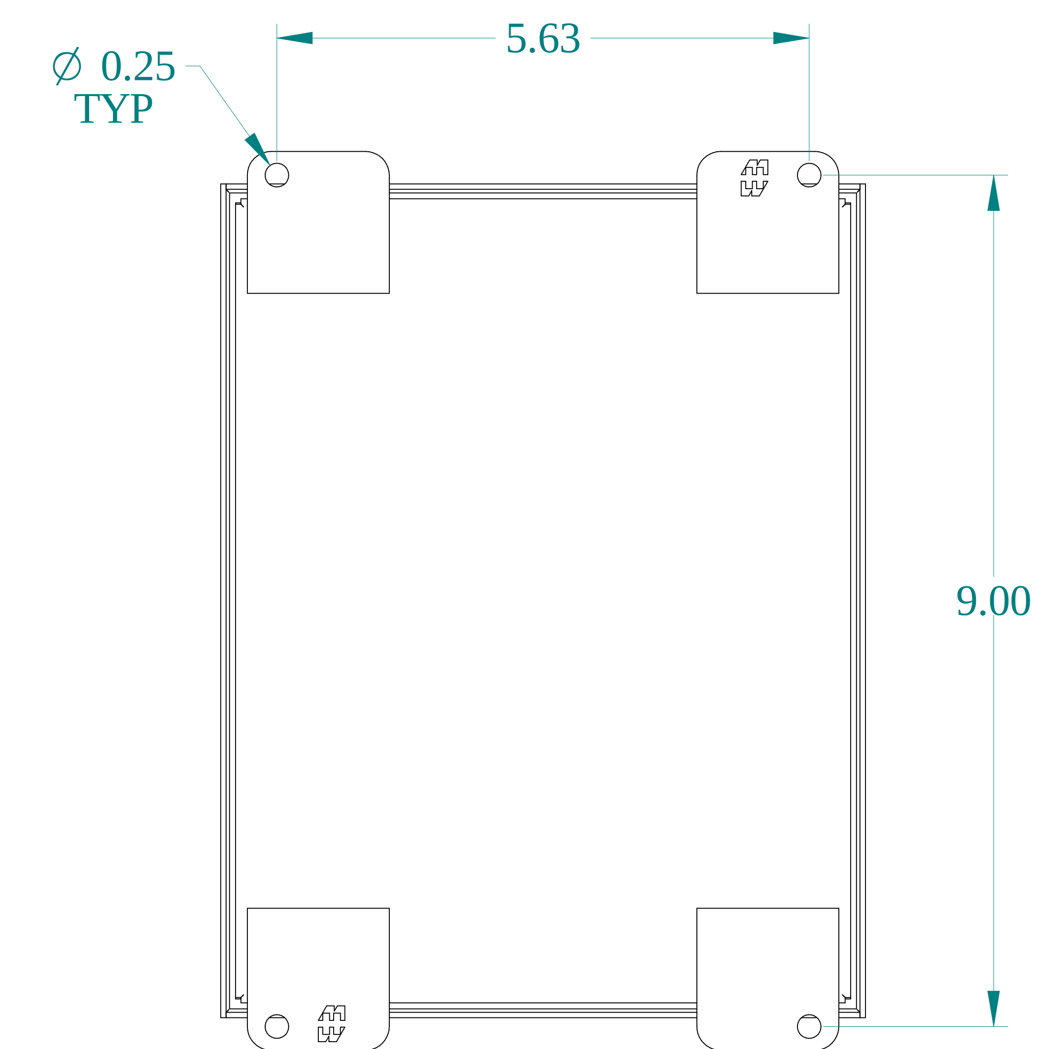
BACK VIEW
