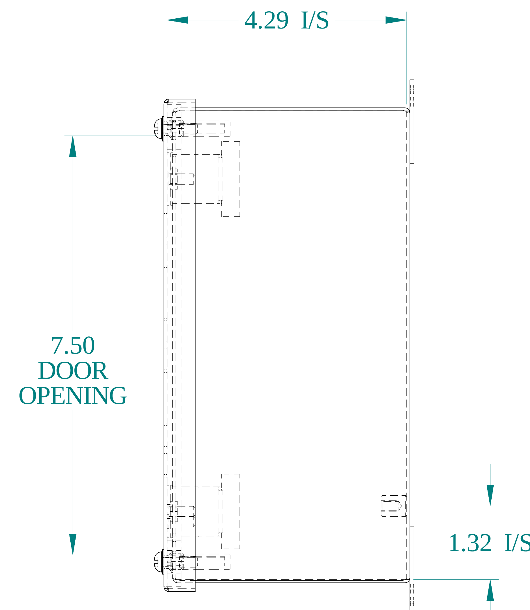
SIDE VIEW
