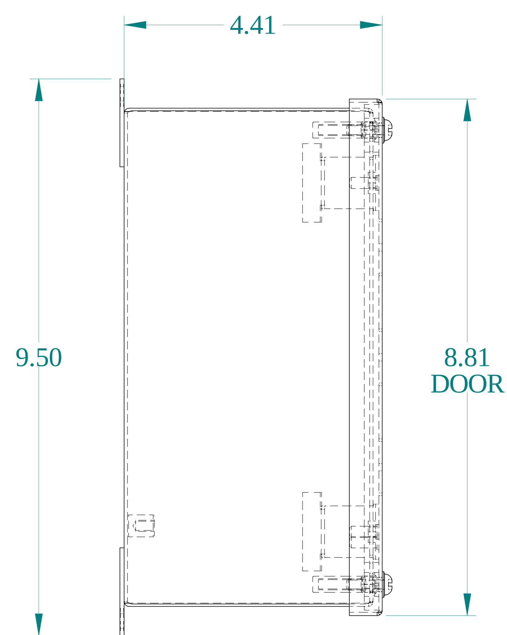
SIDE VIEW
