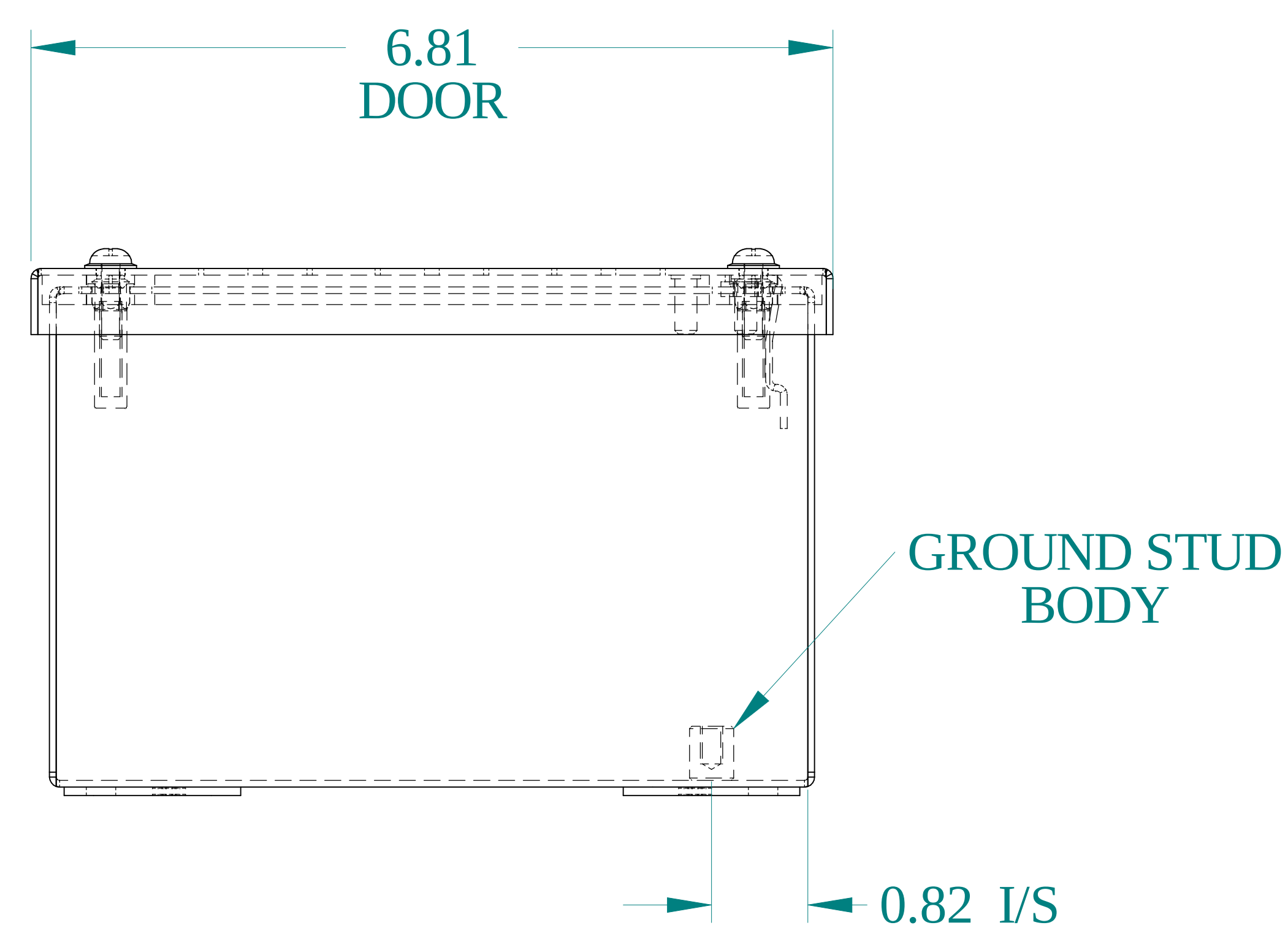
BOTTOM VIEW
