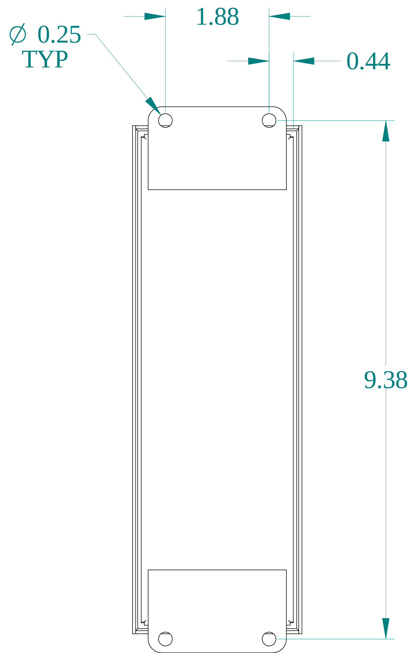
BACK VIEW
