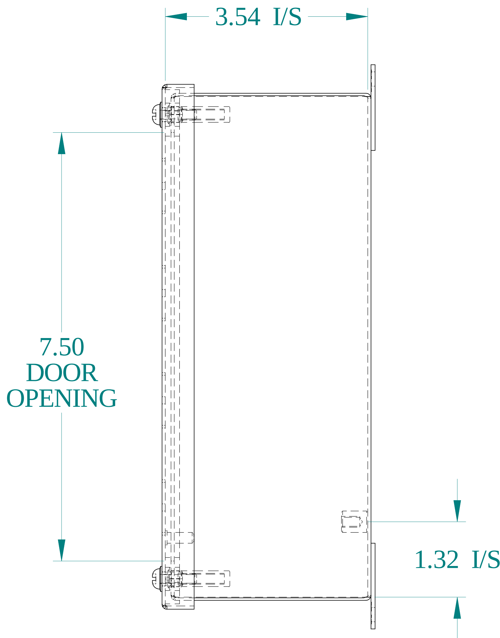
SIDE VIEW
