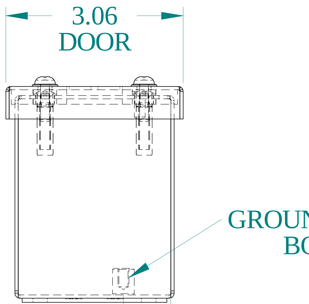
BOTTOM VIEW
