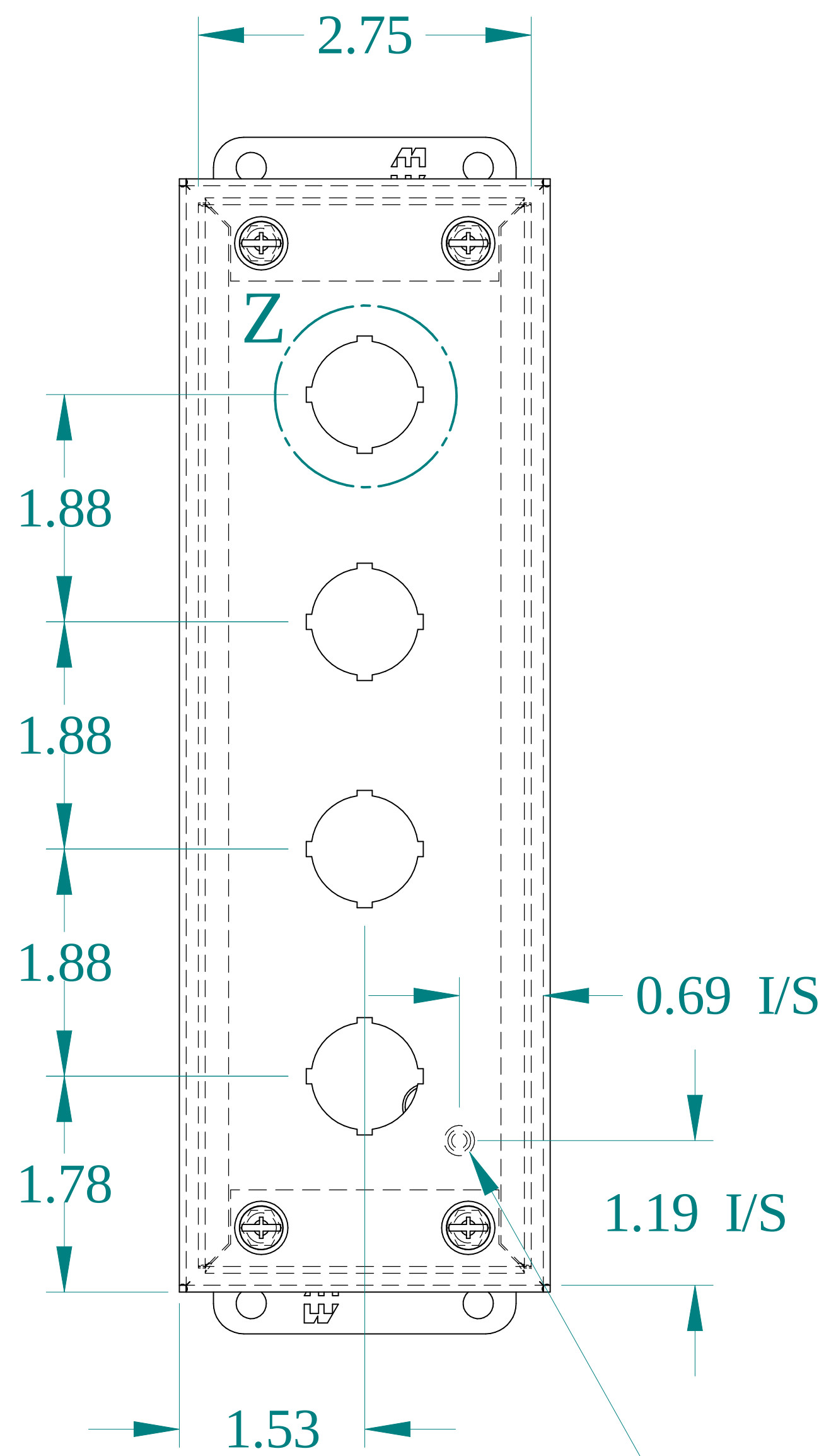
FRONT VIEW
