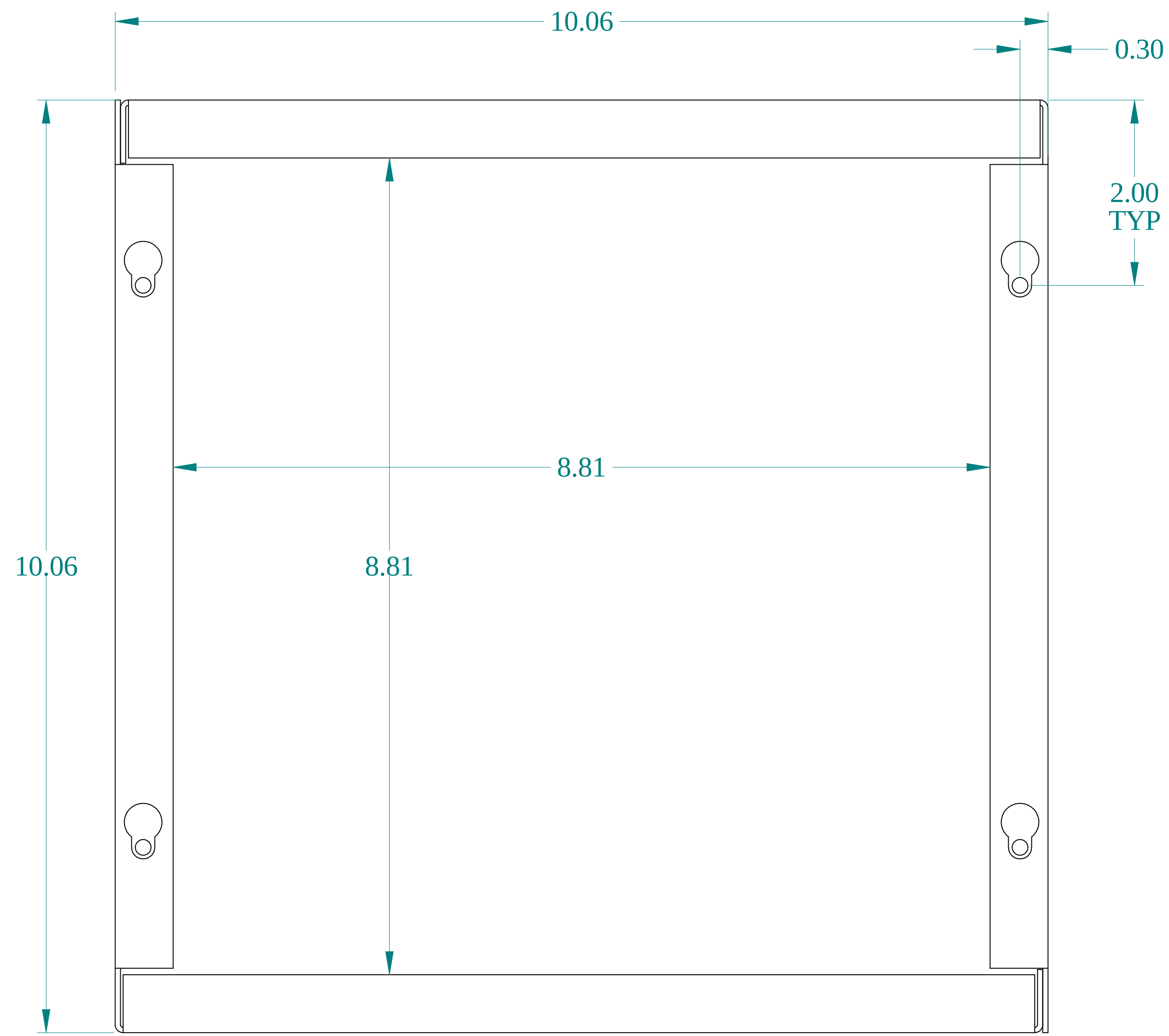
FRONT VIEW
