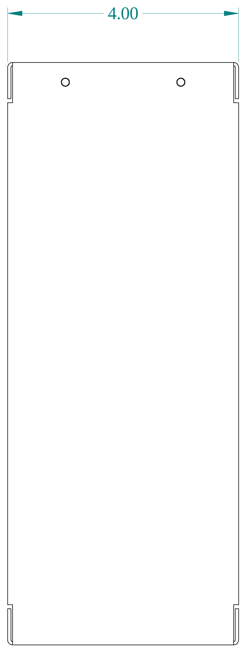
SIDE VIEW
