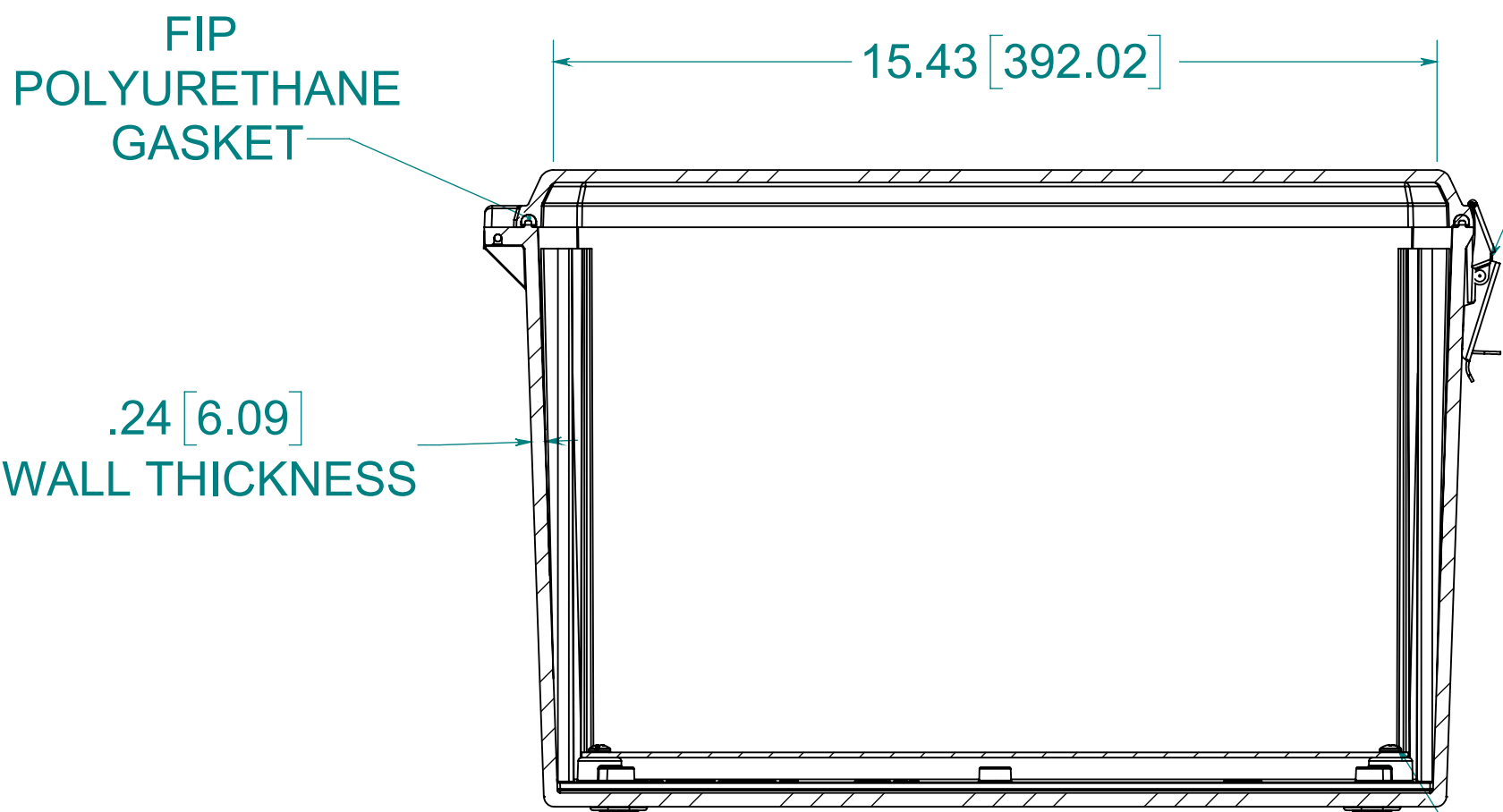
SECTION B-B
