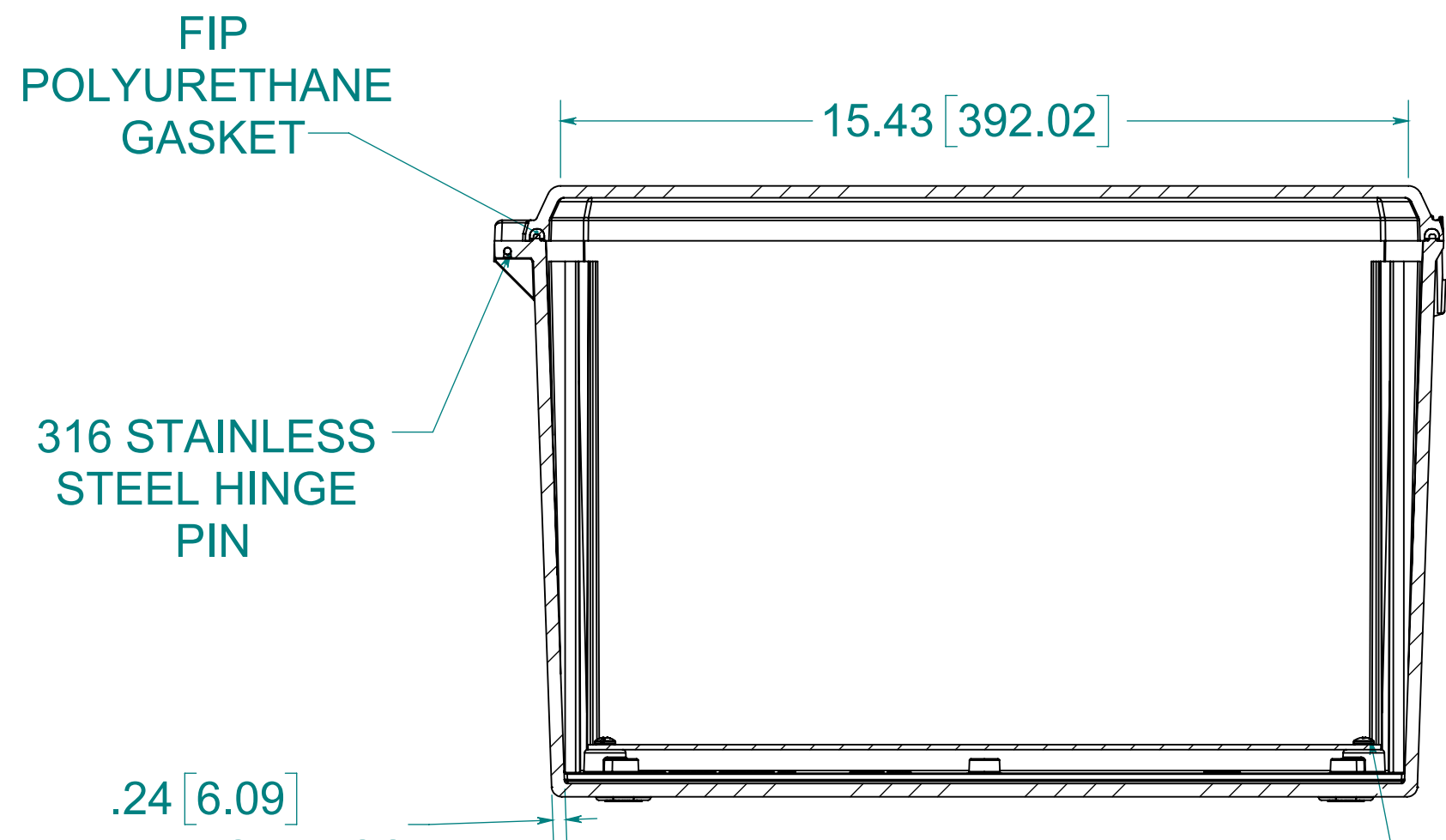
SECTION B-B
