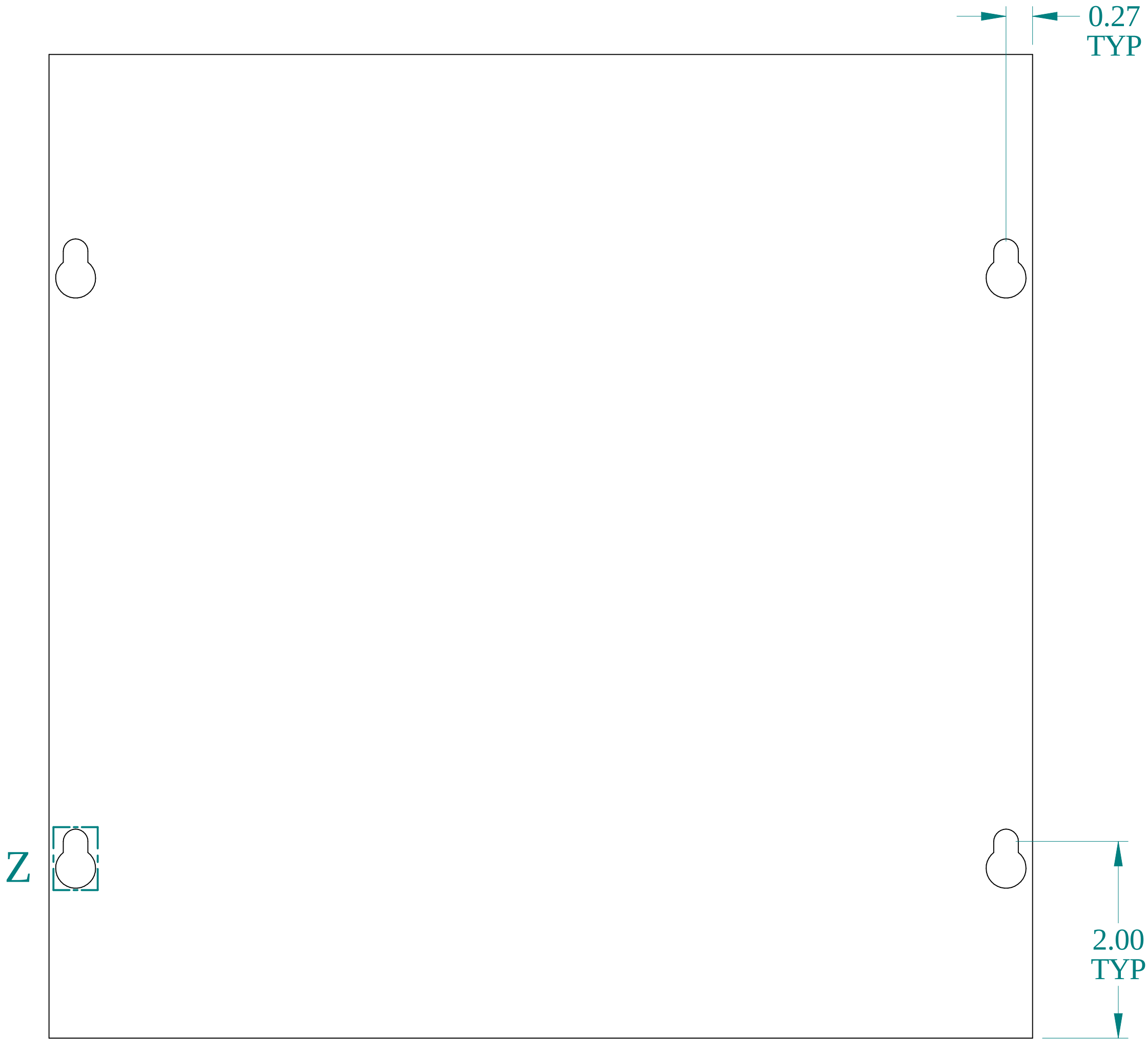
FRONT VIEW
