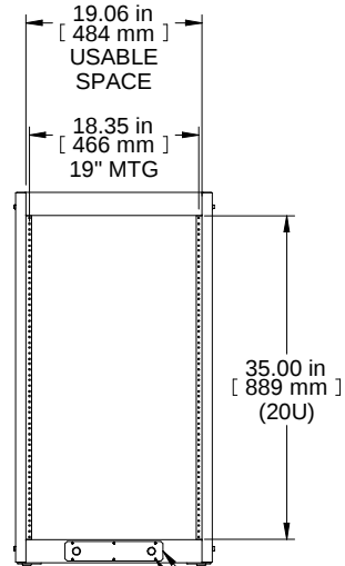
REAR VIEW
