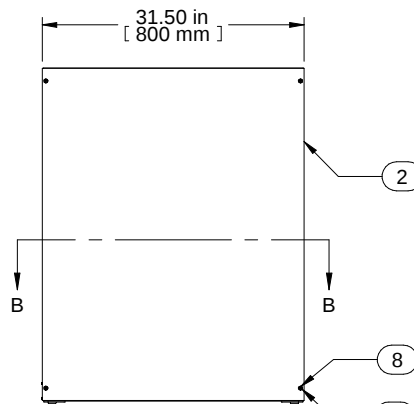
L.S. VIEW
