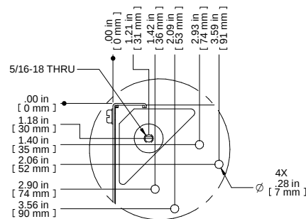
DETAIL C
