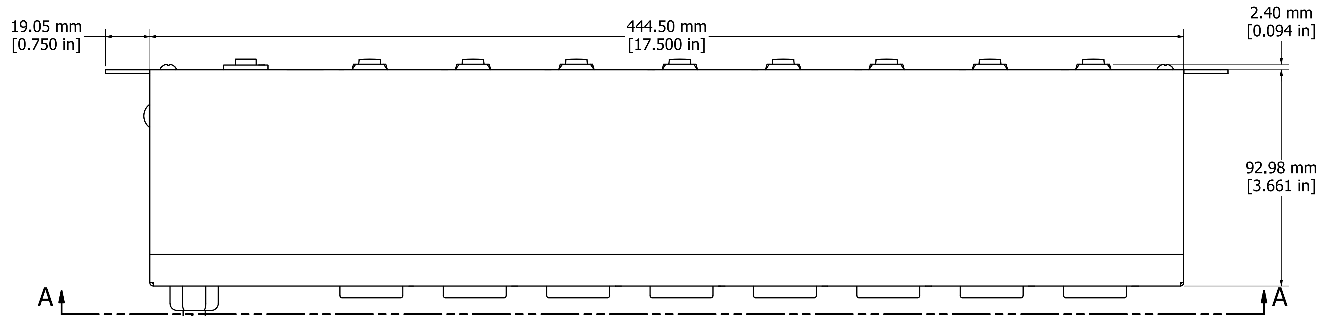
ASSEMBLY - VIEW FROM BOTTOM
