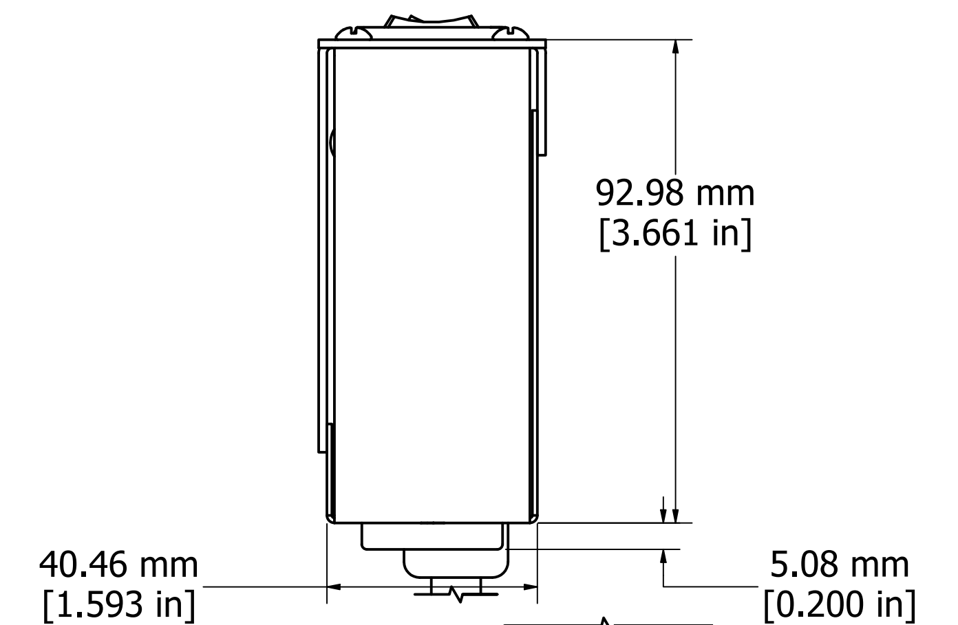
ASSEMBLY - VIEW FROM SIDE
