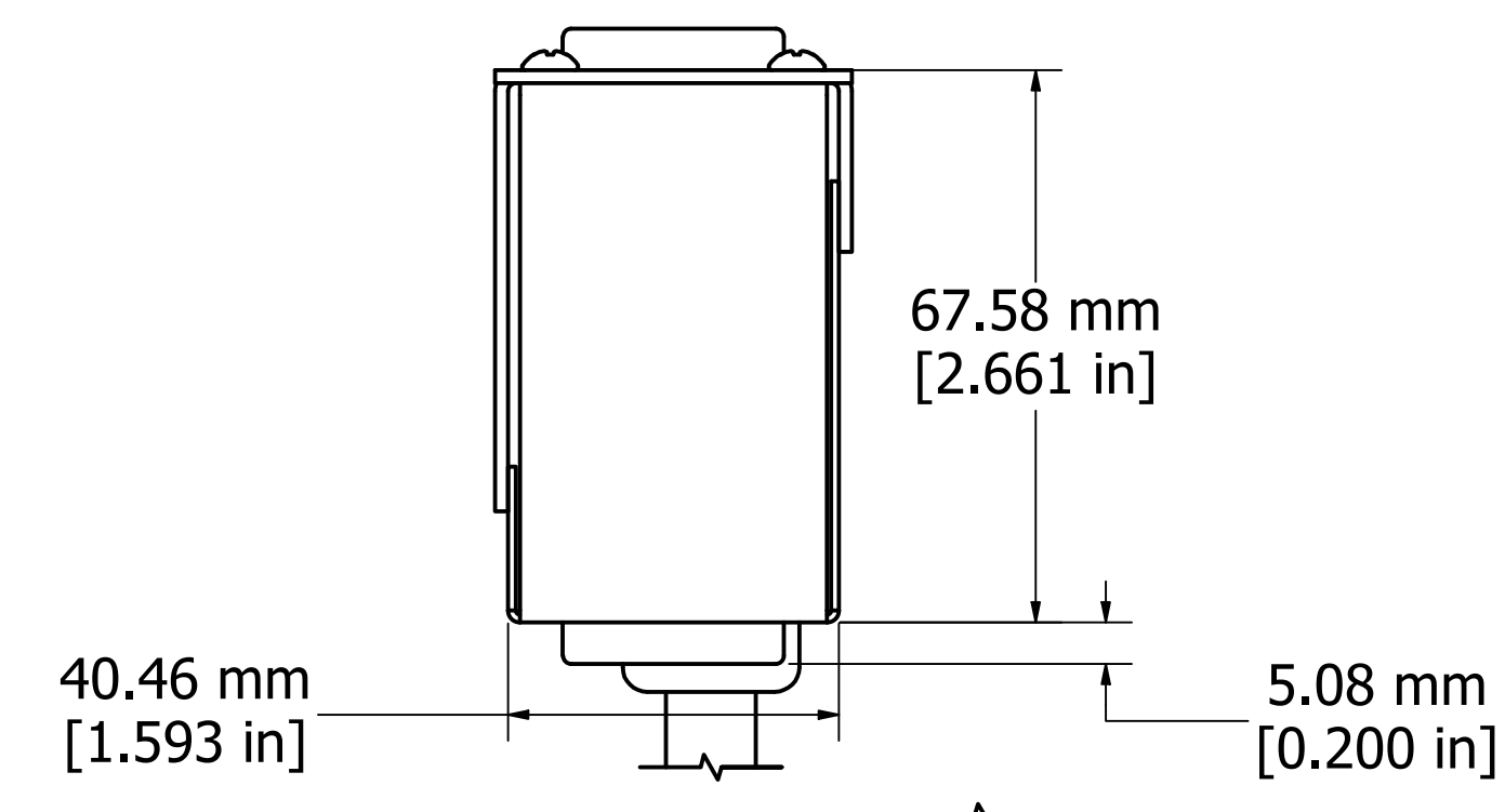
ASSEMBLY - VIEW FROM SIDE
