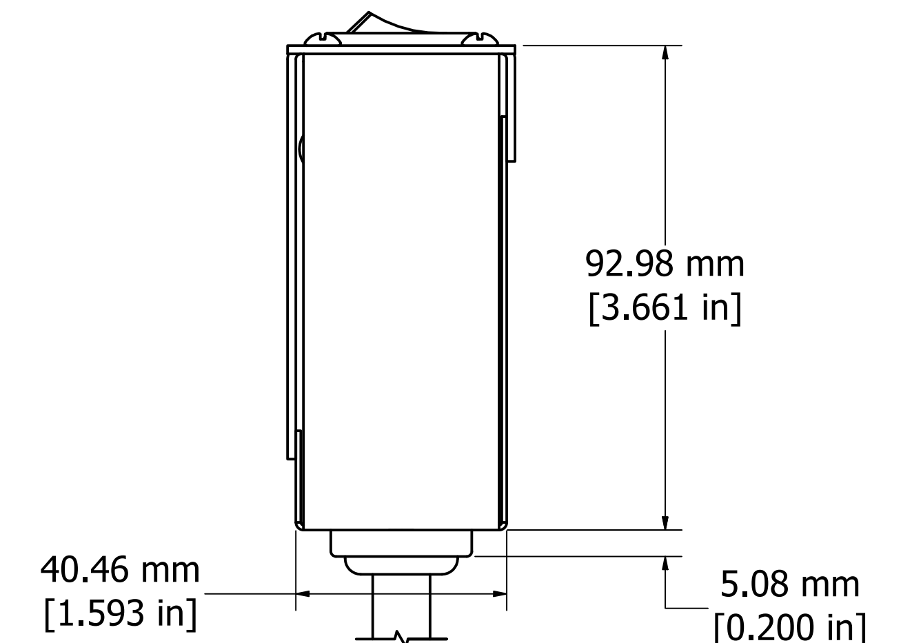
ASSEMBLY - VIEW FROM SIDE
