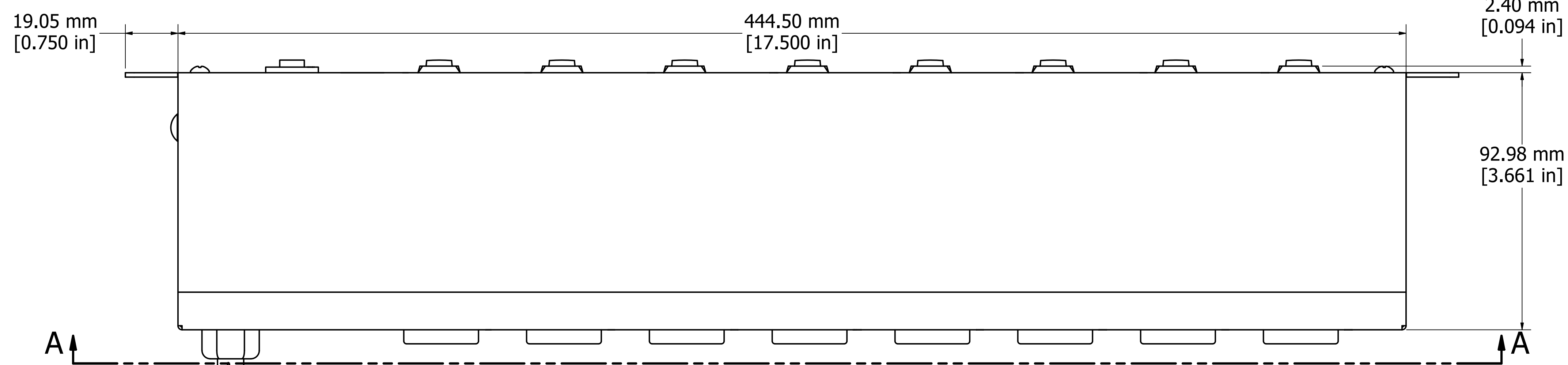
ASSEMBLY - VIEW FROM FRONT
