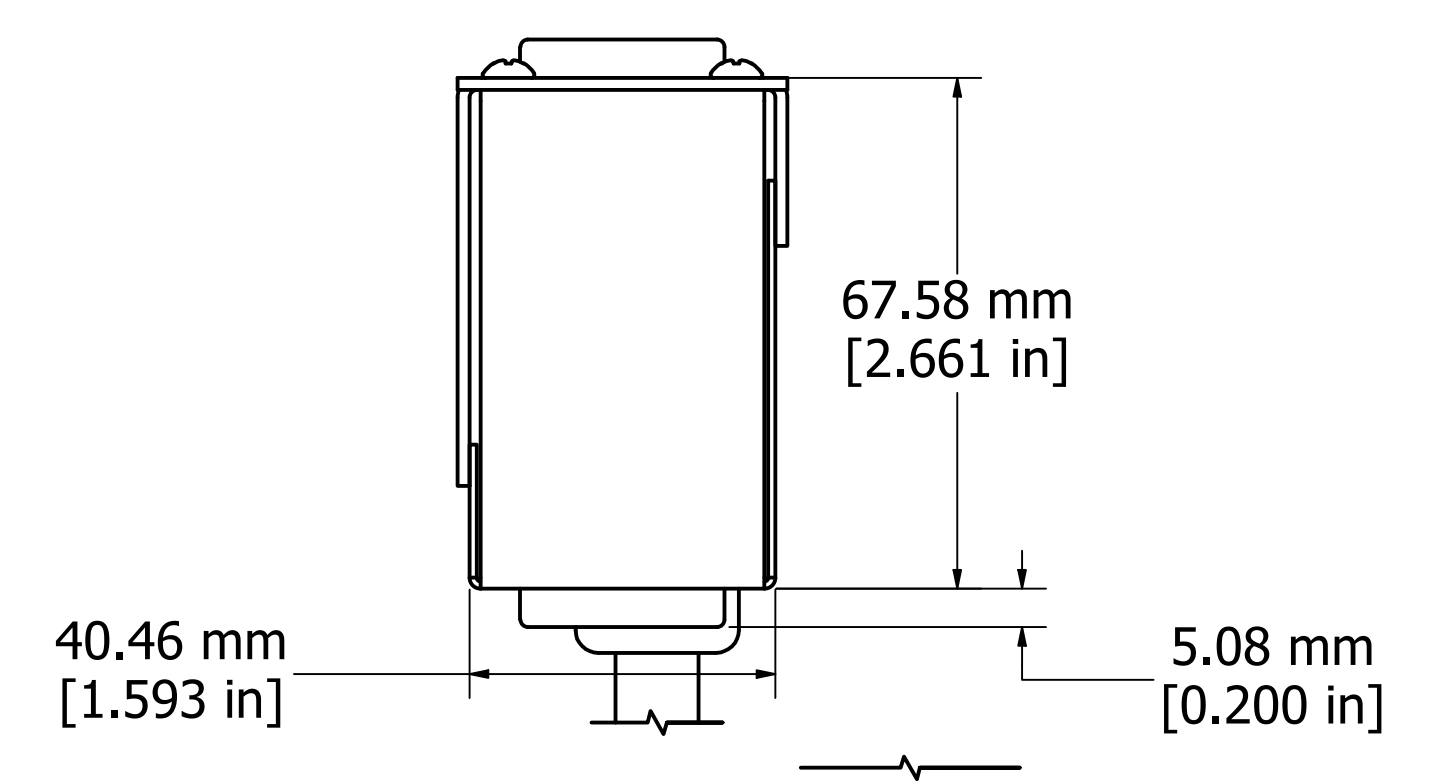
ASSEMBLY - VIEW FROM SIDE
