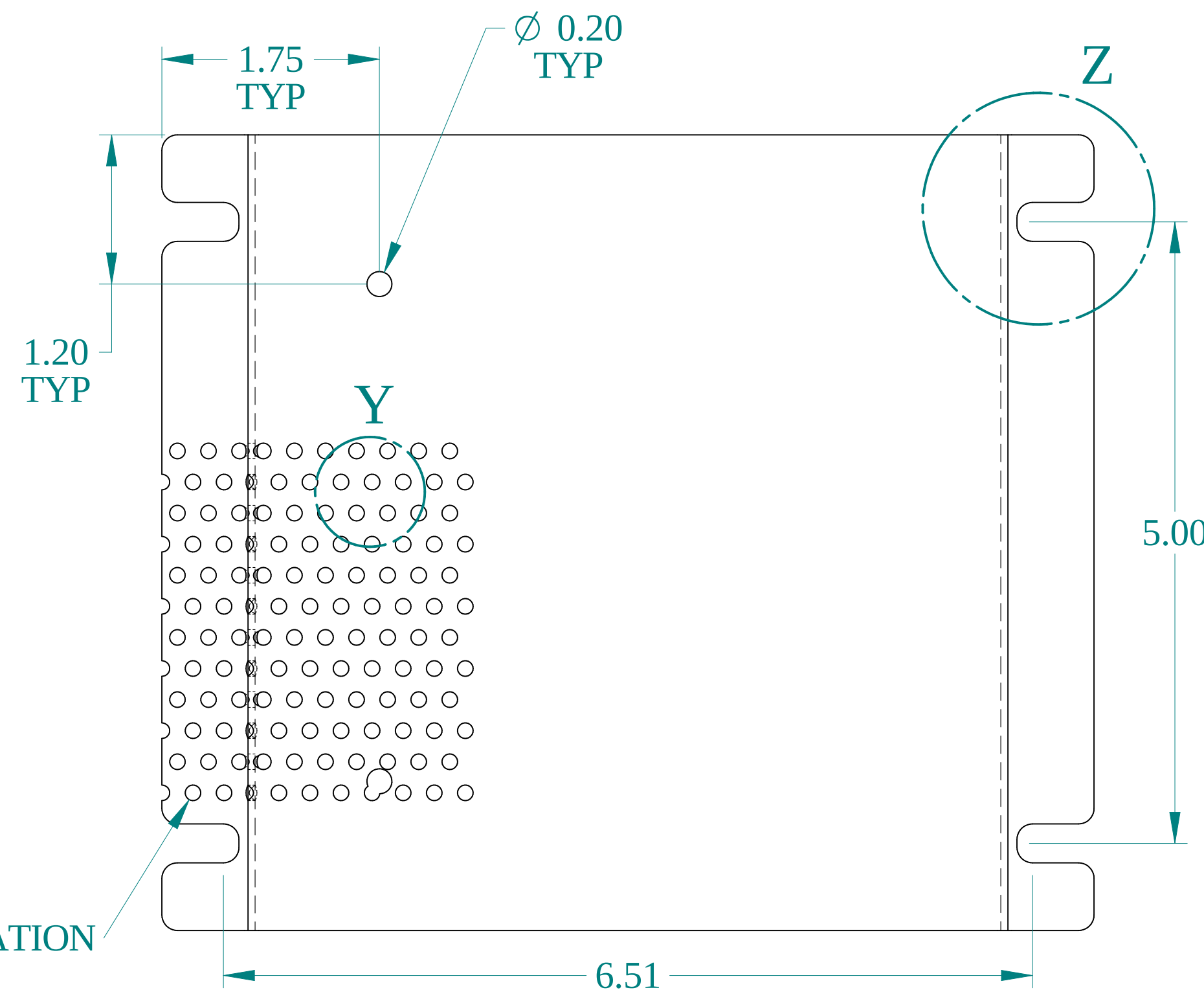
FRONT VIEW
