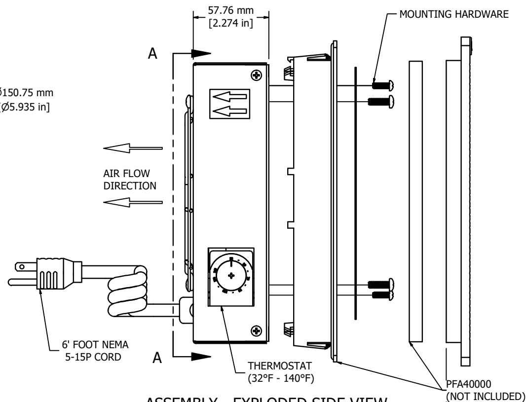
ASSEMBLY - EXPLODED SIDE VIEW
