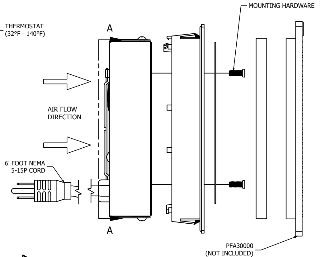
ASSEMBLY - VIEW FROM SIDE
