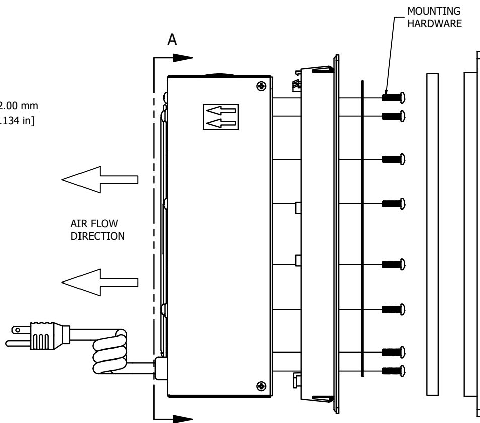
ASSEMBLY - EXPLODED SIDE VIEW
