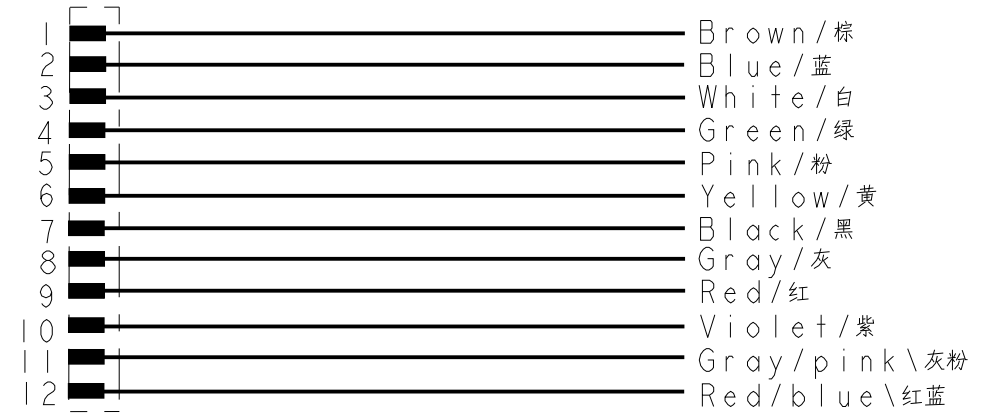
CIRCUIT DIAGRAM MI2, MALE, 12POLES
