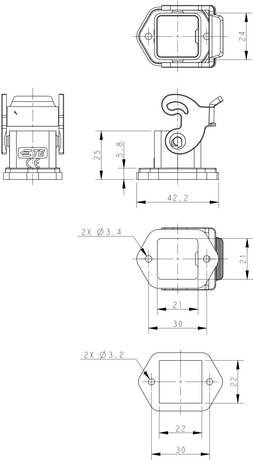
PANNEL CUT OUT FOR REFERENCE 面板开孔尺寸, 仅供参考
