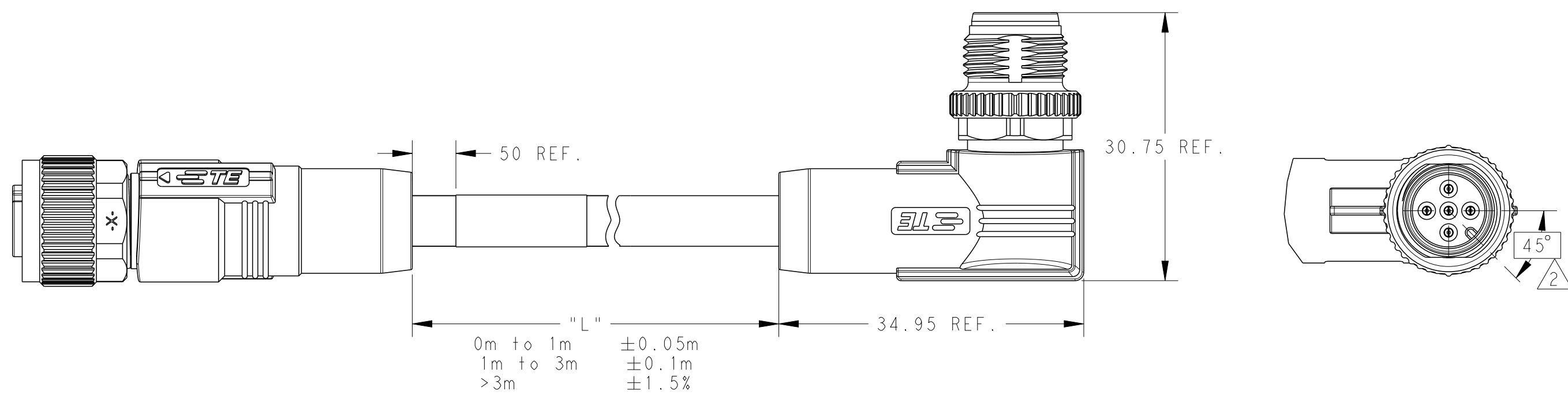
FEMALE STRAIGHT TO MALE RIGHT ANGLE AS SHOWN
