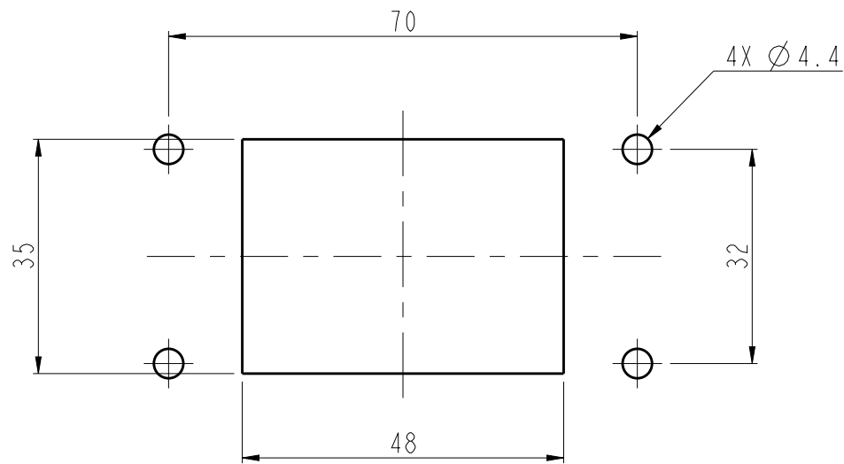
RECOMMENDED PANEL CUT OUT DIMENSION 推荐开孔安装尺寸
