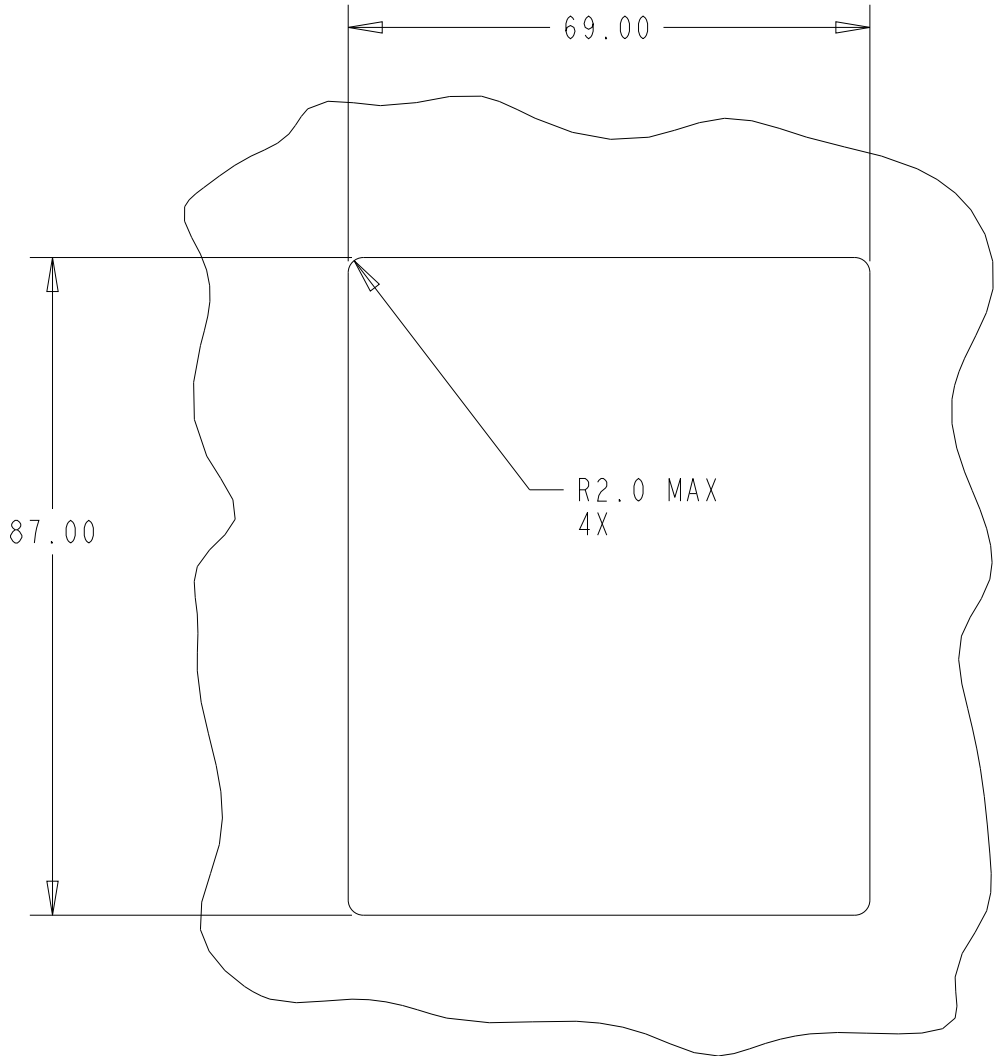
RECOMMENDED PANEL CUTOUT SCALE 1:1
