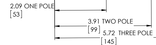
TAP SIDE
