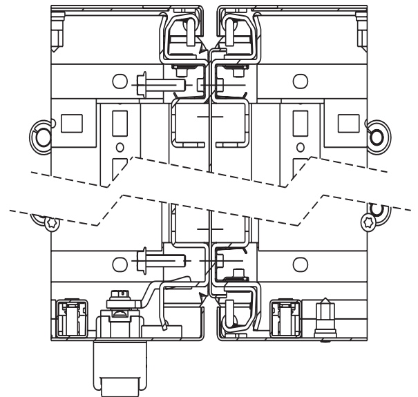
SECTION Z-Z
