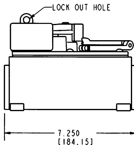
CAT. NO. F34331/A INDUSTRIAL INTERLOCKED RECEPTACLE W/LOCK OUT 30 AMP, 3P4W, 480 VAC FS/FD INTERFACE MATING PLUG - F34332
