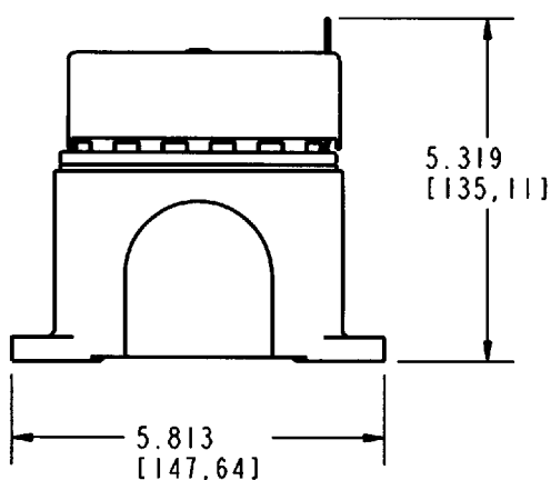
CAT. NO. F34331/A INDUSTRIAL INTERLOCKED RECEPTACLE W/LOCK OUT 30 AMP, 3P4W, 480 VAC FS/FD INTERFACE MATING PLUG - F34332
